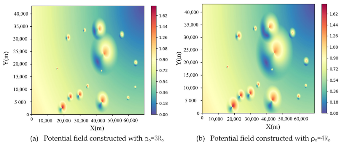
Figure 15. The potential field constructed with the improved APF method.
