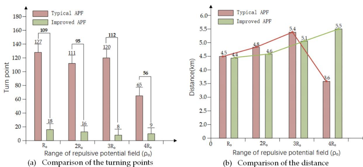
Figure 17. The comparison of the turn points and distance.
