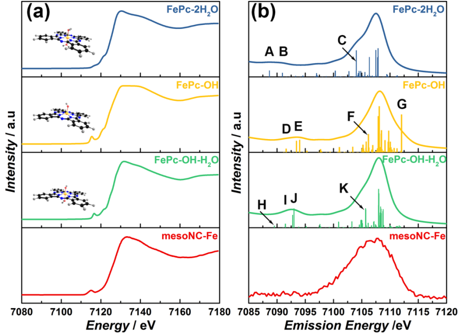
Fig. 8: Comparison of experiments and theory for HERFD-XANES and VTC- K\beta spectroscopies using FePc-2H 2 O, FePc-OH, FePc-OH-H 2 O. Left panel (a): XANES spectrum of mesoNC-Fe (2) compared against FDMNES calculations, Right panel (b): VTC- K\beta spectrum of mesoNC-Fe (2) compared against ORCA calculations. A constant shift of +182.5 eV have been applied.
