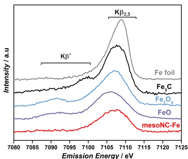
Fig. 5: VTC- K\beta spectra for a selected set of Fe-based compounds and mesoNC-Fe after removal of the K\beta_{1,3} background.
