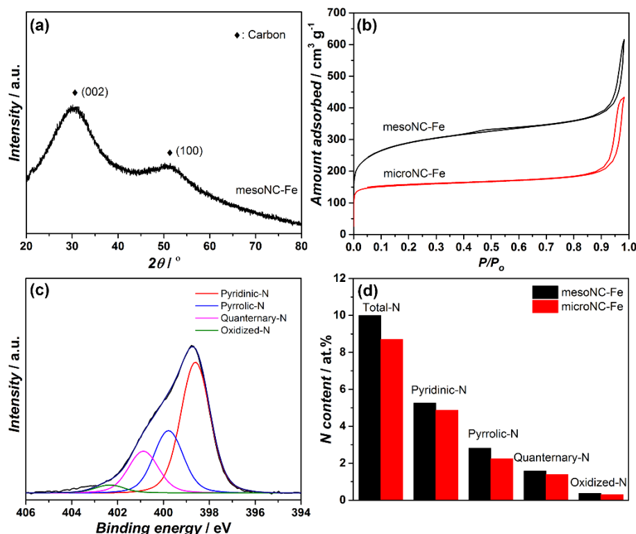
Fig. 3: X-ray diffraction (XRD) patterns of mesoNC-Fe (a); N 2 -sorption isotherms of mesoNC-Fe and microNC-Fe (b); N1s XPS regions of mesoNC-Fe with deconvolution into the N-speciation (c) and N distribution mesoNC-Fe and microNC-Fe (d).
