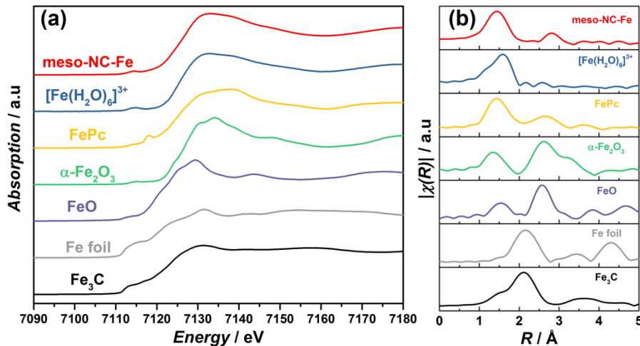
Fig. 4: (a) Fe K-edge XANES spectra and (b) FT-EXAFS k^2\chi(k) functions for meso-NC-Fe, [\text{Fe}(\text{H}_2\text{O})_6]^{3+} in water (0.01M), FePc, \alpha\text{-Fe}_2\text{O}_3 , FeO, Fe foil, and \text{Fe}_3\text{C} . Spectrum of [\text{Fe}(\text{H}_2\text{O})_6]^{3+} in water was retrieved from the F. W. Lytle database ; the International X-ray absorption society website at http://ixs.iit.edu/database/ ; and the spectrum of FePc was kindly provided by Zitolo, et al. [19]
