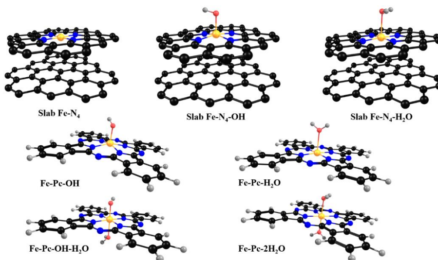
Fig. 7: DFT-optimized geometry for potential local environments of the iron active site in their most stable multiplicity state.
