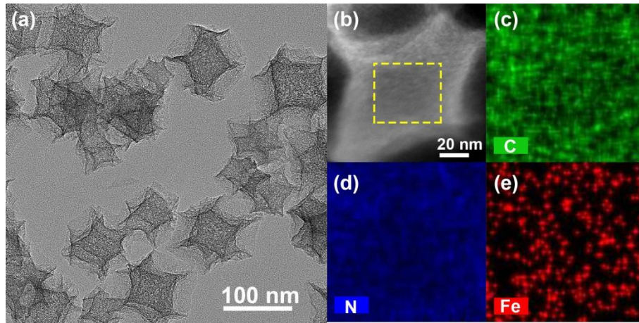
Fig. 2: Bright field TEM and dark field STEM images of mesoNC-Fe (a, b); EDX mapping of C, N and Fe (c-e).
