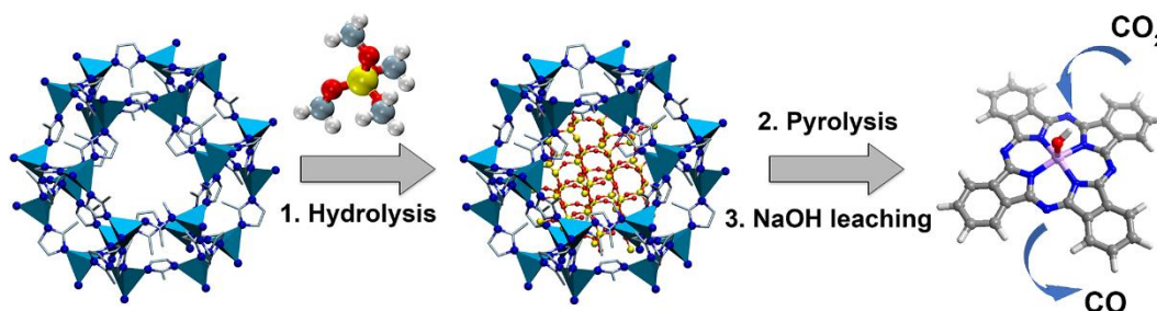
Fig. 1. Schematic illustration of the synthesis of the mesoNC-Fe catalyst. (1) Impregnation and hydrolysis of TMOS molecules in ZIF-8-Fe. (2) Pyrolysis of ZIF-8-Fe@SiO 2 in N 2 to decompose ZIF-8-Fe and form NC-Fe@SiO 2 . (3) NaOH leaching to remove SiO 2 to generate the mesoNC-Fe catalyst.
