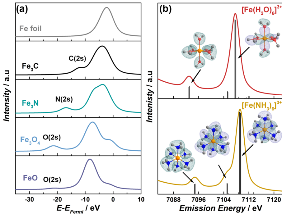
Fig. 6: Calculated VTC- K\beta spectra for a \alpha -Fe, \text{Fe}_3\text{C} , \text{Fe}_3\text{N} , \text{Fe}_3\text{O}_4 , FeO, [\text{Fe}(\text{H}_2\text{O})_6]^{3+} and [\text{Fe}(\text{NH}_3)_6]^{3+} compounds. Left panel (a): spectra for periodic structures calculated with the FDMNES code with the energy scale referenced against the Fermi level. The ligands states sensitivity of K\beta'' is outlined by the ligand orbitals label. Right panel (b): spectra for cluster models calculated with ORCA. A constant shift of +182.5 eV have been applied. Representative alpha molecular orbitals for each peaks are superimposed.
