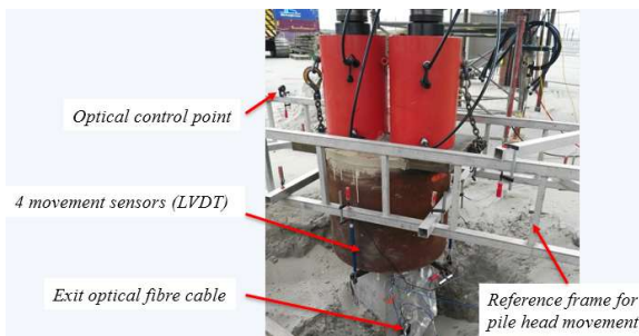
Figure 5. Test site instrumentation 2/2
