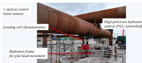
Figure 4. Test site instrumentation 1/2
