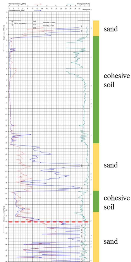
Figure 1. Soil profile at testing site
