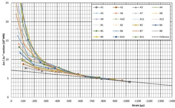
Figure 6. EA according to Fellenius for SLT 2
