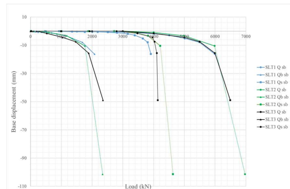
Figure 8. Load-settlement graph SLT
