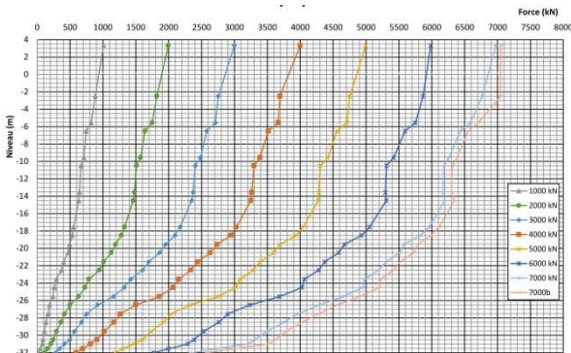
Figure 7. Force distribution along the pile for SLT 2
