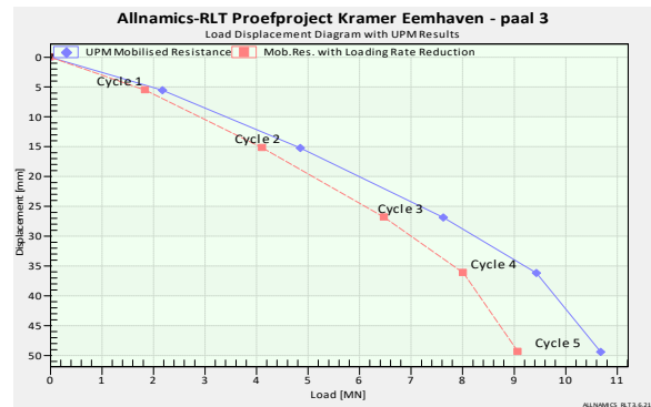
Figure 11. Load-settlement graph RLT at pile P3
