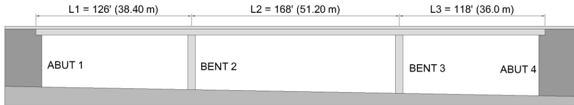
Figure 1 —Elevation view of the bridge.
