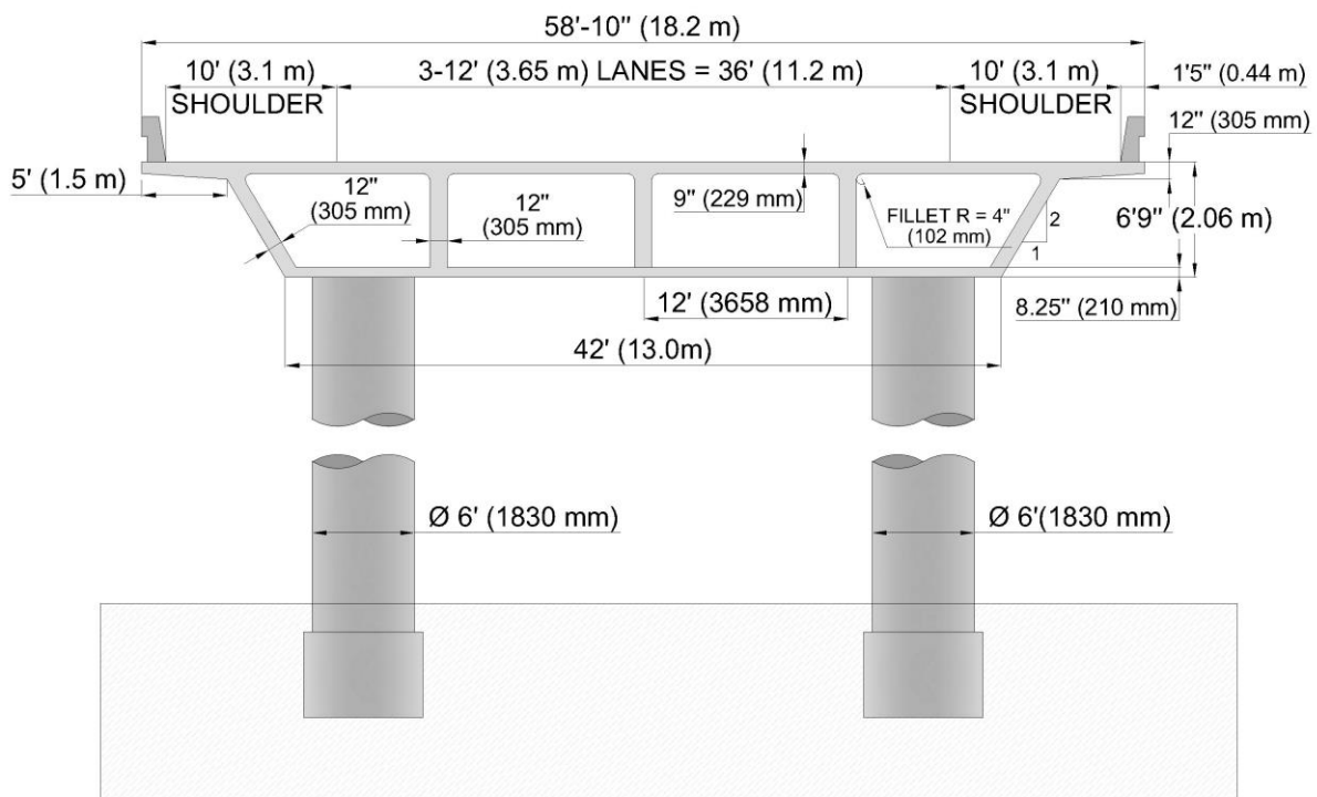
Figure 2 —Cross-section of the bridge.
