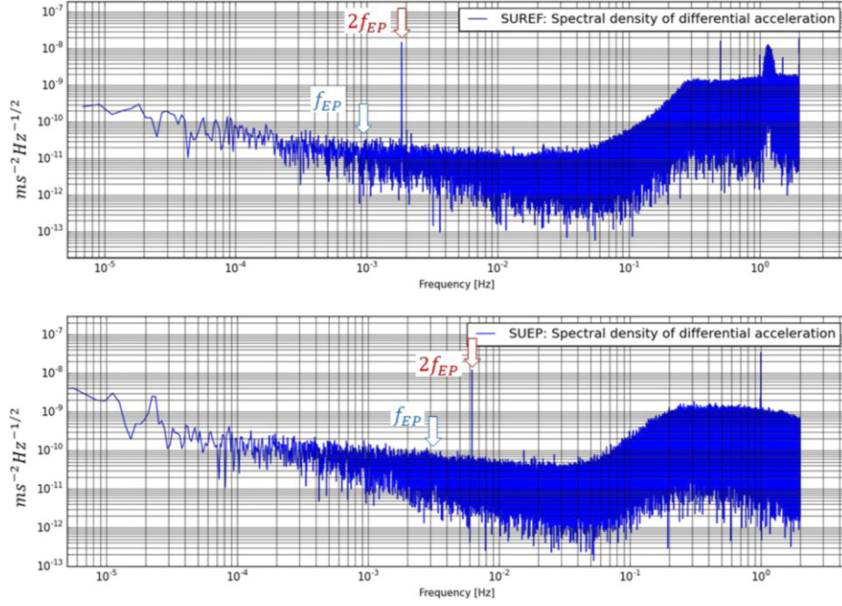
Figure 6. Amplitude spectral density of the sensor differential acceleration along the X -axis for SUREF during session 176 (upper panel) and for SUEP during session 236 (lower panel). Note the peak at frequency 2f_{EP} coming from the Earth's gravity gradient due to the offcentring of the two test masses.
