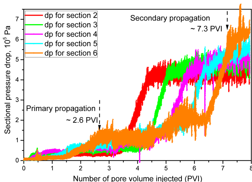
Figure 8—Sectional pressure drops vs. PVI upon injection of pre-generated foam into a Bentheimer core at S_{ow} , with model oil comprising 80 wt% C_{16} and 20 wt% OA. dp denotes sectional pressure drop, with sections 1 ~ 6 numbered from core inlet to outlet. The injection and initial conditions are listed under EXP-04 in Table 2.
