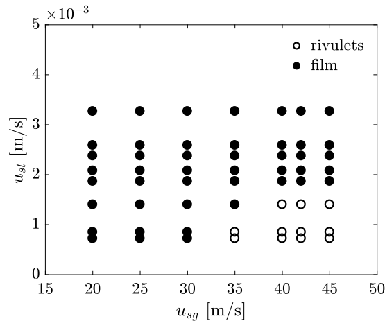
Figure 3.13: Flow map for the experimental parameter space, indicating the regions where a full film and rivulets occur in the smooth pipe.
