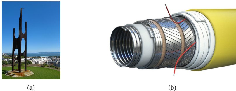
Figure 1.1: (a) Aeolian harp near San Francisco, USA (source: www.kalw.org ). (b) Schematic structure of a flexible riser (source: www.spe.org ).
