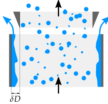
Figure 3.8: Schematic representation of the slit used to remove the film from the pipe wall. \delta D indicates the gap width between the inner pipe wall and the slit edge, which is 2 mm at each side.
