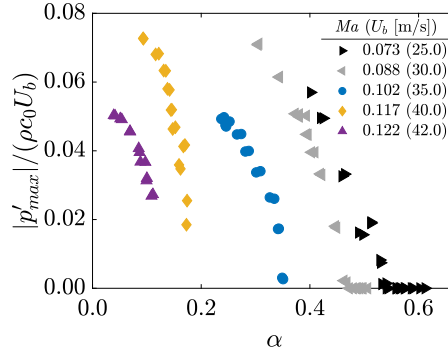
Figure 4.15: Dimensionless whistling amplitude as a function of the liquid filling fraction \alpha , for geometry D, with water injection.
