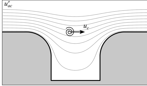
Figure 4.2: Schematic representation of the acoustic streamlines over a cavity structure, with a coherent vortex traveling in the cavity mouth with velocity u_c . The interaction of the vortex with the acoustic field is a source of sound.
