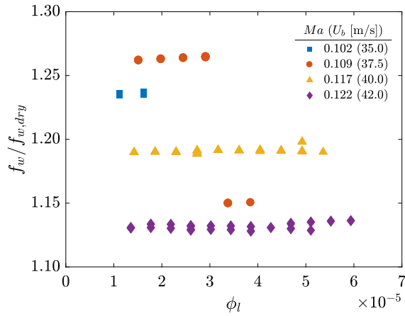
Figure 2.10: The change in whistling frequency relative to the dry whistling case as a result of liquid injection. Largest jump is observed for Ma = 0.109 ( U_b = 37.5 m/s). The symbols are as defined in Figure 2.9
