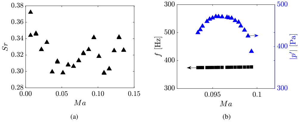
Figure 2.8: (a) Strouhal ( Sr ) versus Mach ( Ma ) number plot for dry whistling in the corrugated pipe. (b) Dry whistling amplitude as a function of Mach number at a single frequency plateau. Whistling frequency is displayed by ■, whistling amplitudes by ▲. The parameter range is indicated with a dashed rectangle in Figure 2.7.
