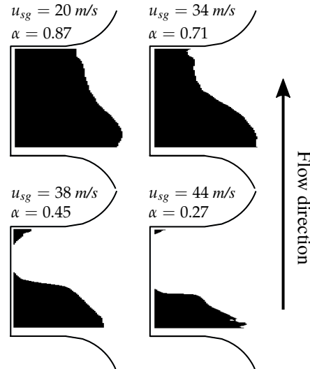
Figure 3.20: Liquid cavity filling profile, measured with the PLIF method described in Section 3.2, for the four different cases indicated in Figure 3.19a. Flow is from bottom to top and dark regions are regions of liquid accumulation. u_{sl} = 0.11 cm/s for all cases.
