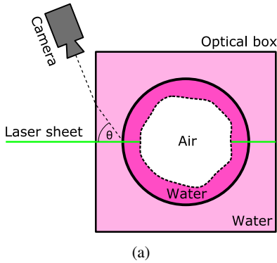
Figure 3.5: (a) Schematic of the PLIF set-up used for the film thickness measurements, seen from the top. The water at the interior of the pipe is dyed with 150 \mu\text{g/L} rhodamine WT, water in the optical box with 50 \mu\text{g/L} . (b) Example images obtained using an inverse ray-tracing technique for \theta of 75^\circ , with (A) the image obtained by the sensor (the dashed line indicates the actual gas-liquid interface), and (B) the results obtained with and without using the line detection method.
