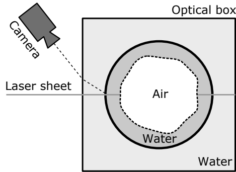
Figure 2.3: Schematic of the PLIF set-up used in the visualization measurements, as seen from the top. The water in the interior of the pipe is dyed with 125 \mu\text{g/L} rhodamine, water in the optical box with 50 \mu\text{g/L} .
