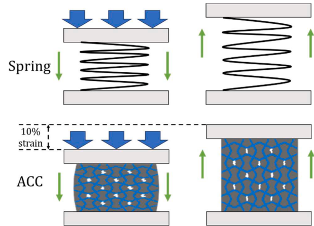
Fig. 9. Schematics of the deformation mode of ACC and a spring under certain pressure, both exhibit recoverable deformation, for the ACC in this work at least 10% of cyclic strain is reached, compared to conventional cementitious mortar 10 % deformability is significantly higher.
