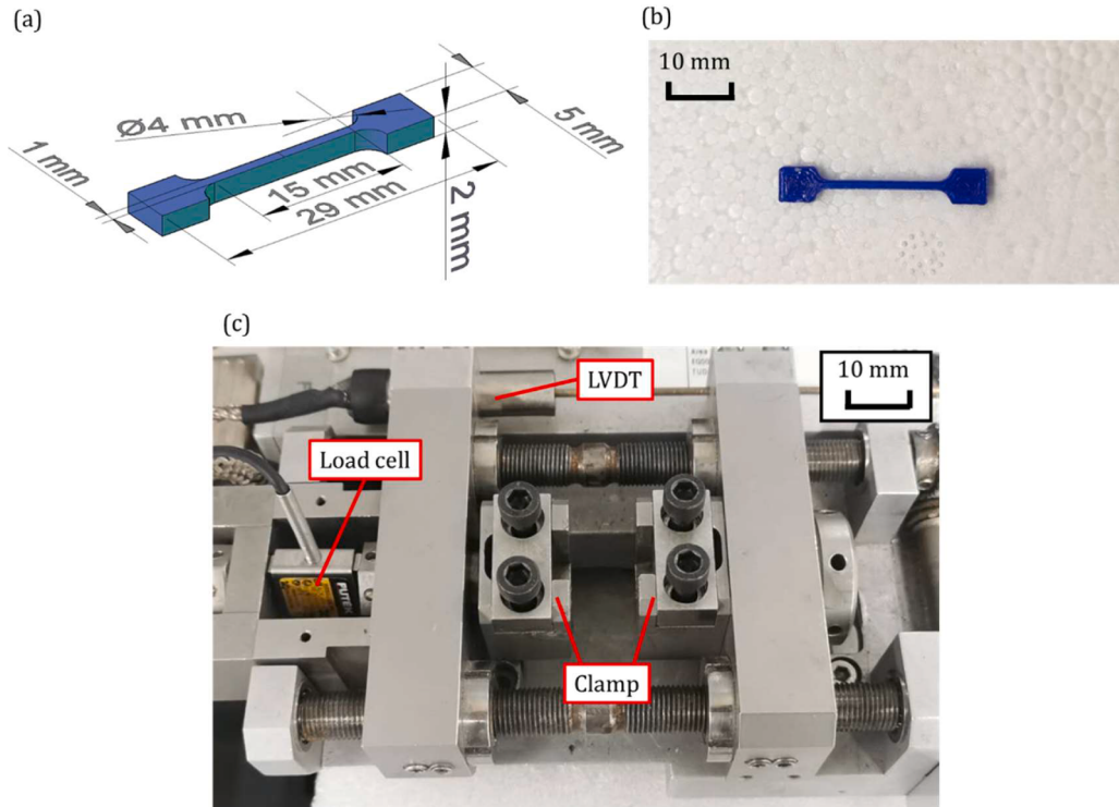
Fig. 2. (a) Schematics of the designed dog-bone shape specimen for understanding the constituent properties of the TPU material; (b) the 3D printed dog-bone specimen; (c) micro compression-tension test machine used for the mechanical tests of the TPU dog-bones.
