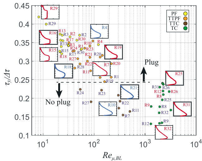
Figure 17. Nondimensional yield stress parameter as a function of boundary layer Reynolds number for all the runs. Inset plots are velocity profiles of the runs obtained from the first (blue) and the second (red) UVP probes. Circles represent where each run is situated within the plot. The run numbers are shown next to each circle and represent the data from the first (blue) or the second (red) UVP probes. The yellow, orange, brown, and green colors represent the flow type corresponding to each run. The horizontal line separates the regions where a plug exists from where it does not. The line is dashed to convey that this boundary may be a sloping or a curved line. PF = plug flow; TTPF = top transitional PF; TTC = transitional turbidity current; TC = turbidity current.
