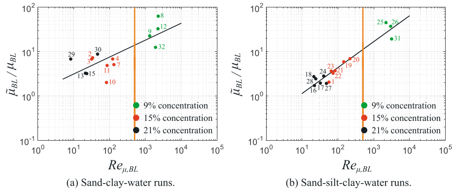
Figure 9. \bar{\mu}_{BL} / \mu_{BL} versus Re_{\mu,BL} for the data gathered from the second Ultrasonic Doppler Velocity Profiler probe for (a) sand-clay-water runs and (b) sand-silt-clay-water runs. The vertical orange line indicates Re_{\mu,BL} = 500 . Dots indicate where different runs are situated in this plot. Run numbers are placed next to their corresponding dots. Runs with 21% sediment concentration are shown in black, runs with 15% sediment concentration are shown in red, and runs with 9% sediment concentration are shown in green. The black line is a least squares fit to the data.
