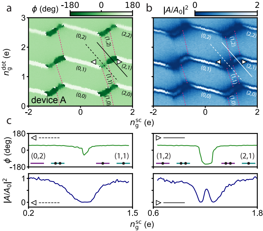
Figure 4.2: Spin-dependent tunneling between a QD and a SC. a and b Charge stability diagram of device A measured in phase a and amplitude b . The charge states are labeled with (n^{\text{SC}}, n^{\text{QD}}) with respect to the state (N, M) with N and M even. Dashed pink lines: expected locations of the lead-island transitions. c Linecuts of the phase (green) and amplitude (blue) along the interdot transitions. The linecut crosses the states (0,2) and (1,1) in the left panel (dashed line) and (1,2) and (2,1) in the right panel (continuous line). A pronounced different resonator response is observed for the two transitions. For the |e(\text{ven}), S(\text{inglet})\rangle to |o(\text{dd}), D(\text{oublet})\rangle transition between (0,2) and (1,1) (left panel), both spin channels are available, while only one spin channel contributes to the |o, S\rangle to |e, D\rangle transition between (1,2) and (2,1) (right panel).
