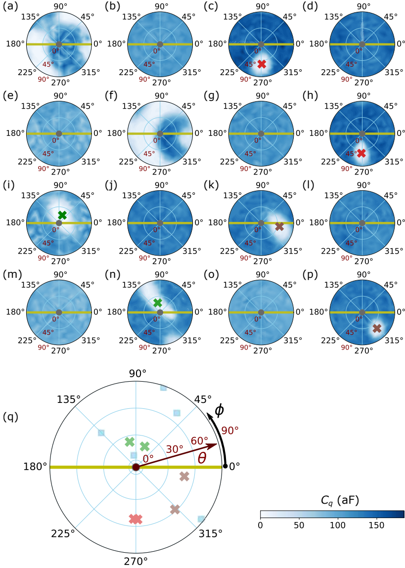
Figure 5.5: (a-p) The external magnetic field angle map of C_{q,max} ( 0^\circ \leq \theta \leq 90^\circ , with |\vec{B}| = 50 mT) for 16 neighboring ICTs, with their extracted \vec{B}_{SO} directions marked by colored crosses. These ICTs are labeled with the corresponding charge occupations (n'_L, n'_R) with respect to even charge numbers (N'_L, N'_R) . (q) Summary of the extracted \vec{B}_{SO} directions for the even-occupied ICTs under study. Crosses in the same color correspond to the ICT pairs with the same valence orbital. Squares mark the ICTs when the other ICT from a pair is not measured.
