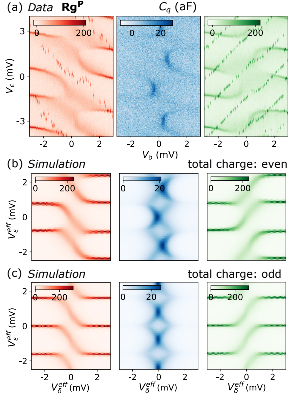
Figure 7.9: Reasons on assuming even total charge number for the hybrid triple dot. (a) The charge stability diagram for another measured regime Rg^P . (b) The simulation result when assuming even-occupied system. The data in (a) show a much closer qualitative resemblance to (b) than to (c), particularly in relation to the signal recorded through the SIP resonator. (c) The simulation result when assuming odd-occupied system.
