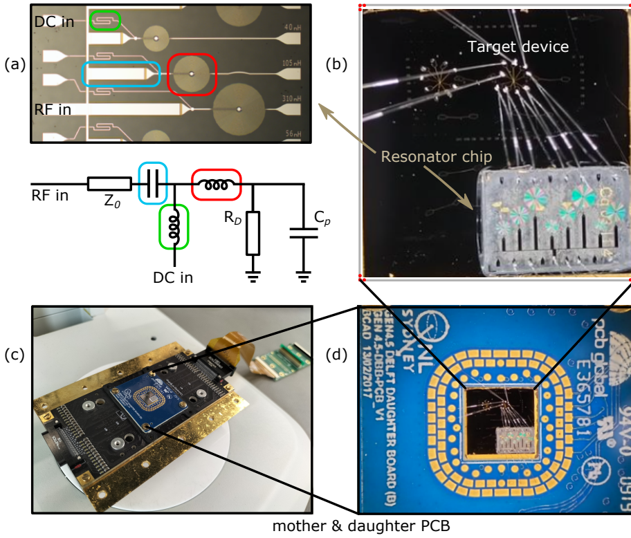
Figure 3.5: Prepare the sample chip for cryogenic measurements. (a) The photo of a section of the MUX resonator chip fabricated on a sapphire substrate using superconducting niobium (top), and the corresponding circuit (bottom). The frequency multiplexing is achieved by the different inductances, labelled on the right side of the MUX resistor chip. (b) The resonator chip is glued on the sample chip, with the target device connected by bonding wires. (c) The daughter board is screwed to the mother board. After covering the daughter board with a cotton cap, the sample chip is ready to be loaded into the probe for electrical measurements. (d) The sample chip is glued on a daughter PCB, whose metal pads are connected to both the resonator chip and the device by aluminium bonding wires.
