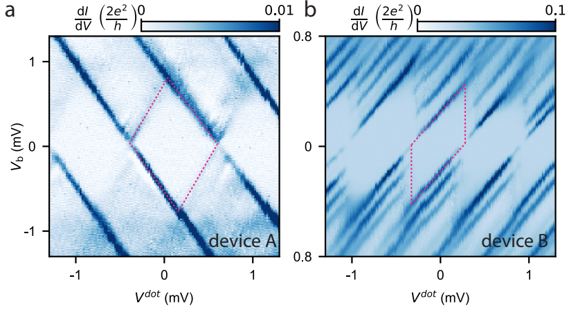
Figure 4.5: Coulomb blockade measurements on the quantum dots. a For device A, the conductance is calculated from the numerical derivative of the measured current. We extract E_C^{\text{QD}} \approx 300 \mu\text{eV} , \delta = 50 - 150 \mu\text{eV} , and \alpha^{\text{QD}} = 0.8 . b For device B, we obtain E_C^{\text{QD}} \approx 200 \mu\text{eV} , \delta = 100 - 170 \mu\text{eV} , and \alpha^{\text{QD}} = 0.72 .
