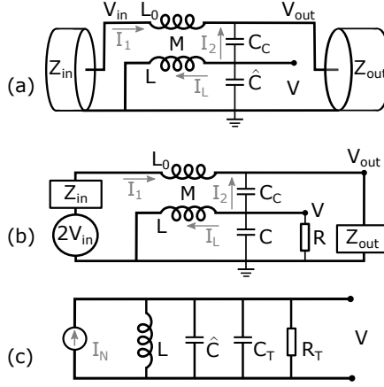
Figure 2.6: Measurement setups on transmission lines with its equivalent circuits. (a) A schematic illustrates the setup for measuring resonators, incorporating both inductive and capacitive coupling. The setup also includes transmission lines with mismatched characteristics. (b) The equivalent circuit with the complex capacitance \hat{C} in (a) is separated into a capacitive part ( C ) and a resistive part ( 1/\omega R ). (c) The Norton equivalent circuit for (b), with V denoting the voltage across the capacitor. This diagram helps with getting the expression of Norton equivalent conductance G_N and current I_N .
