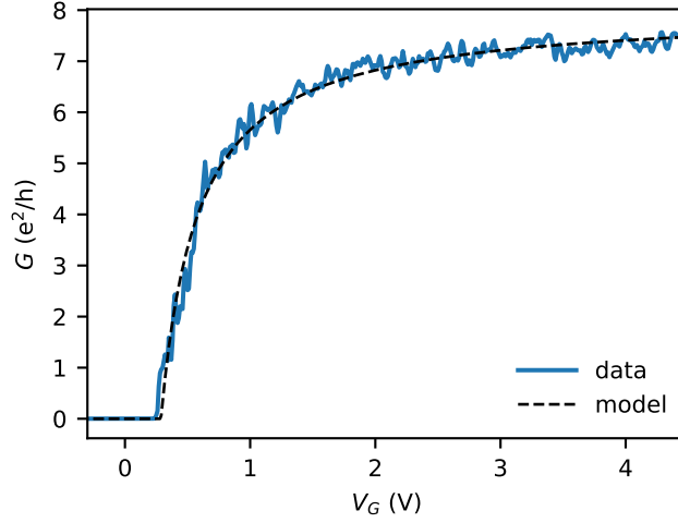
Figure 6.10: Pinch off curve of the 500 nm InSb device, used for extraction of mobility in Fig. 6.5.
