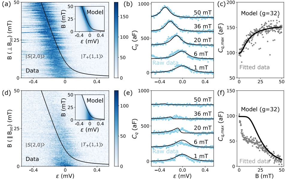
Figure 5.4: Evolution of the ICT in external magnetic field \vec{B} for (a-c) \vec{B} \perp \vec{B}_{SO} , and (d-f) \vec{B} \parallel \vec{B}_{SO} . (a,d) C_q as a function of \vec{B} and \epsilon . The inset presents the numerical simulation. Black curves in both the main figure and the inset indicate the degeneracy point between |S(2,0)\rangle and |T_+(1,1)\rangle . (b,e) Line cuts of (a,d) for several magnitudes of \vec{B} . For clarity, they are separated in the C_q axis by 200 aF. Black curves come from the simulation. (c,f) C_{q,max} as a function of \vec{B} . Grey dots are extracted from a phenomenological Gaussian fit of the data. Black curves indicate the C_{q,max} taken from the insets of (a,d).
