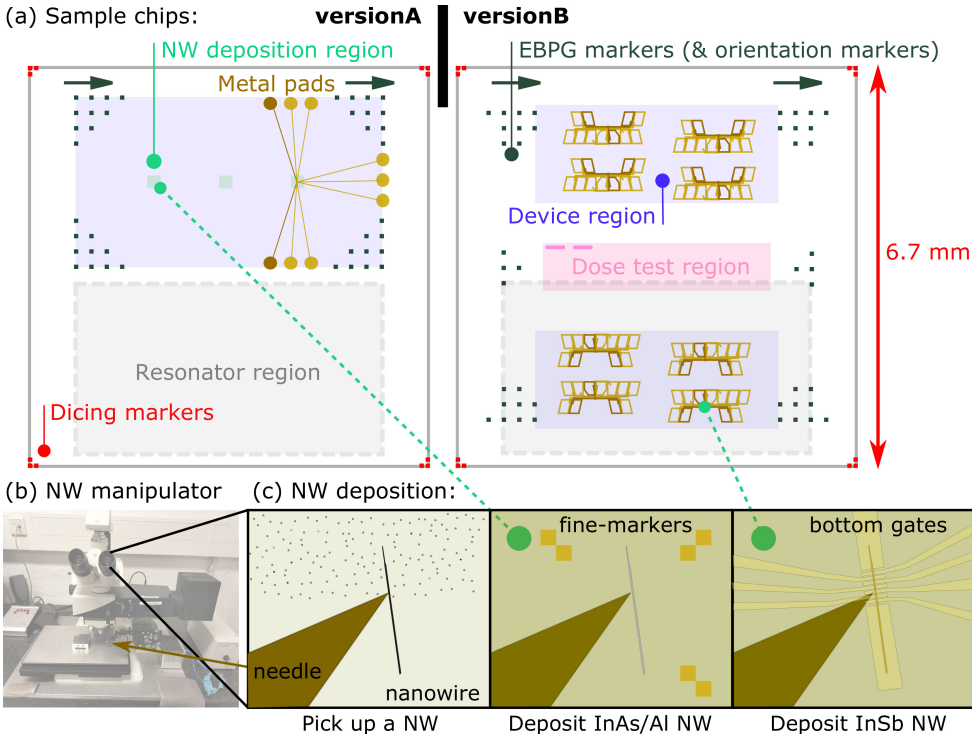
Figure 3.2: Design of sample chips and nanowires deposition. (a) There are two versions of diced sample chips: Version A has one device region, which can hold three devices, and one resonator region, which is ready to attach an off-chip resonator. Version B has two device regions, each capable of accommodating many devices, and a region for dose test, maximising the use of a single chip. The device region with fewer operating units can be selected as the resonator region later. (b) Transferring nanowires from a growth chip to a pre-fabricated sample chip is facilitated by a nanowire manipulator machine. The three microscope images on the right showcase the process: the needle picking up a nanowire from the nanowire forest on the growth chip (left); the needle depositing the InAs/Al nanowire in the center of the marked region, identified by fine EBPG markers (middle); the needle depositing the InSb nanowire on the previously placed bottom gates (right).
