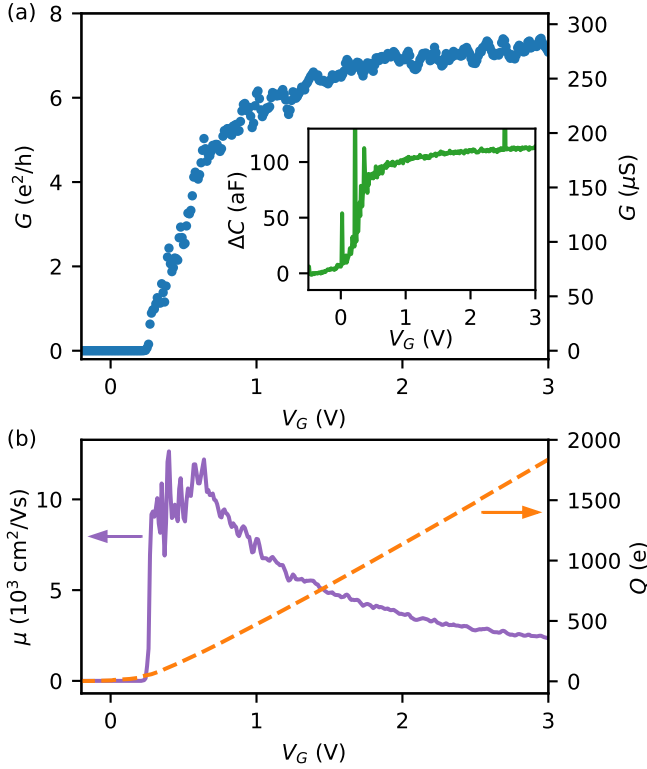
Figure 6.5: (a) Conductance G as a function of gate voltage V_G in an InSb nanowire device with 500-nm-wide bottom gate. (inset) Added capacitance \Delta C as a function of gate voltage V_G . (b) Mobility of the nanowire device and charge in the conductive channel versus gate voltage V_G .
