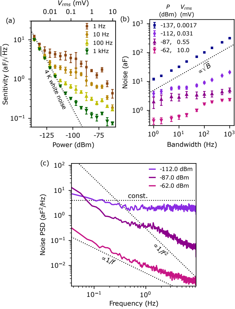
Figure 6.3: (a) The measured sensitivity of the capacitance measurement. The dotted line indicates the sensitivity limit due to the amplifier noise ( T_{\text{noise}} \approx 4 K). (b) The standard deviation of the gate capacitance measurement vs vector network analyzer bandwidth. The dotted line indicates the scaling of the noise \propto \sqrt{B} , expected for white noise such as Johnson-Nyquist noise. (c) The capacitance noise spectrum, for a measurement bandwidth of 50 Hz.
