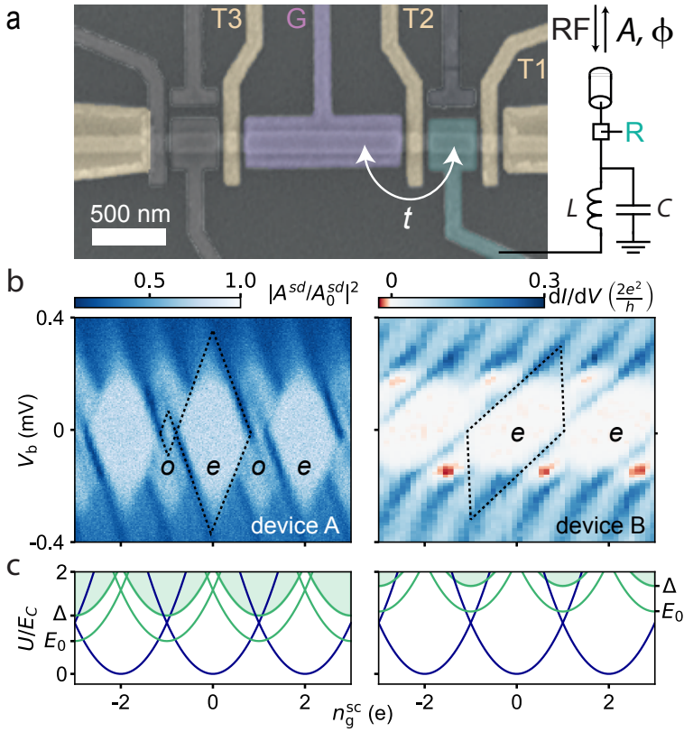
Figure 4.1: Experimental setup and sample characterization. a False-colored electron micrograph of a nominally equivalent hybrid double dot. The plunger gate of the QD (island) is colored cyan (purple). A LC resonator is capacitively coupled via the gate of the QD. Its phase \phi and amplitude A response are monitored at a constant probe frequency. b Coulomb blockade measurement of the SC. Left: for device A measured using RF reflectometry off the source (circuit not shown in a ). The even-odd pattern indicates that E_0 < E_C^S . Right: for device B measured using standard lockin techniques. The doubling of the period at low bias V_b illustrates that E_0 > E_C^S . c Energy dispersion of the superconducting island for device A (left) and device B (right). The even (odd) energy levels are shown in darkblue (green). The odd parity sector consists of a discrete subgap state at E_0 and a continuum of states above \Delta .
