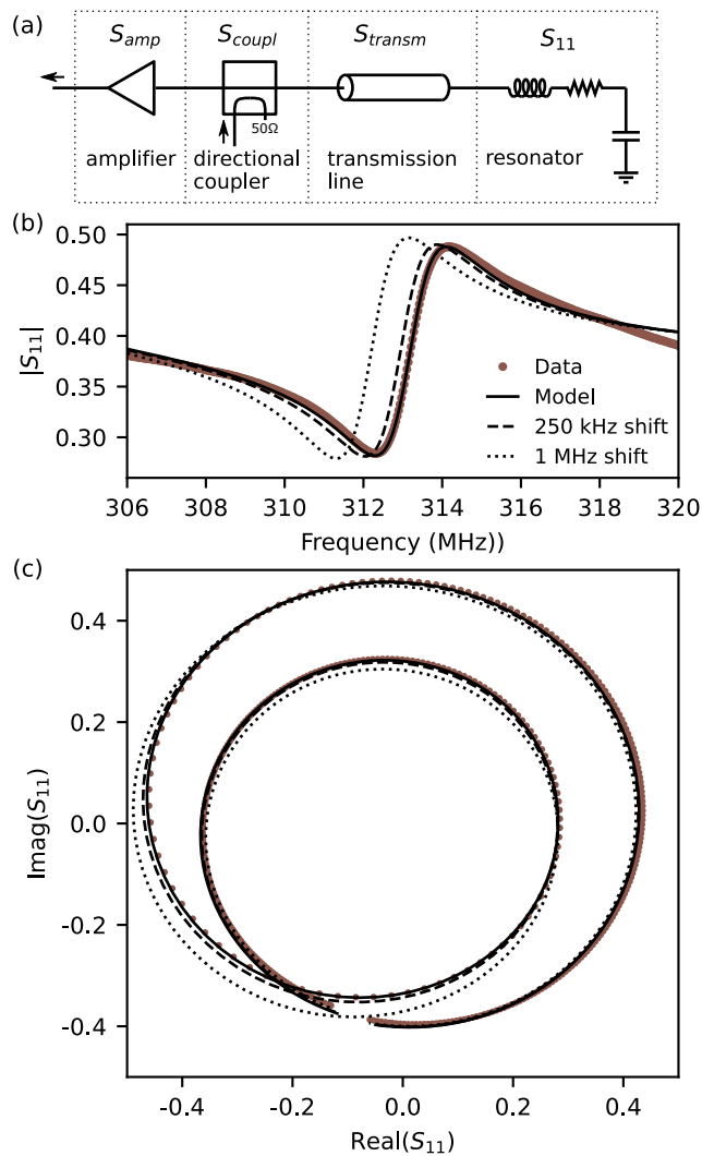
Figure 6.6: (a) Circuit schematics employed to model the resonance asymmetry of the resonator used for characterization of the performance in Sec. 6.4. (b) Absolute value of S_{11} and (c) parametric plot of real and complex part. Solid line indicates the fit of Eq. (6.15) to the data. Dashed and dotted line indicate the predicted signal in case the resonance frequency is lowered by 250 kHz and 1 MHz, respectively.
