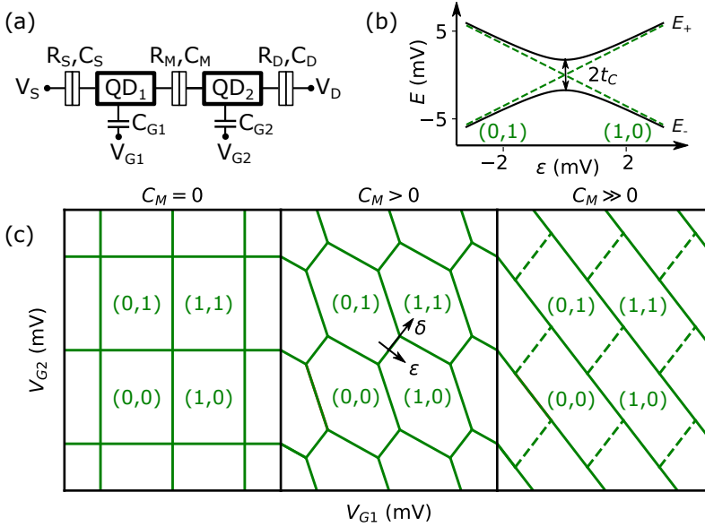
Figure 2.2: Double quantum dot (DQD). (a) The equivalent circuit model of a DQD system, in which the two QDs are coupled in series. (b) The hybridization spectrum of the two charge states (N_1 + 1, N_2) and (N_1, N_2 + 1) arises from interdot coupling t_C . (c) The charge stability diagrams that depict the equilibrium electron numbers corresponding to (N_1, N_2) in the gate space defined by V_{G1} and V_{G2} , as the mutual capacitance C_M is varied. Here, N_{1(2)} represents the charge number of QD 1(2). When C_M = 0 , the two QDs are completely decoupled. The horizontal and vertical lines indicate the gate settings at which the number of electrons in the ground state changes. When C_M is finite, interdot transitions appear, making the charge numbers in two QDs interdependent. When C_M is large enough, the two QDs are not distinguishable, such that the system is equivalent to a single QD that is gated by both V_{G1} and V_{G2} .
