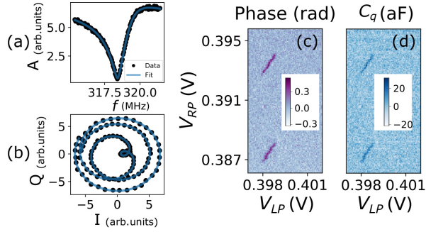
Figure 5.2: (a) The magnitude of the reflection signal as a function of probing frequency, as an example of the reference data. The black dots represents the raw data, while the blue curve shows the fitting result. (b) Parametric plot of the resonator reflection measurement in I-Q plane, and the corresponding fit result. (c) The reflected phase signal of the entire CSD. (d) The corresponding color maps of C_q values.
