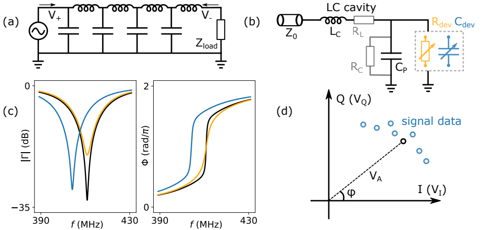
Figure 2.4: Impedance and reflections. (a) Schematic of an equivalent lumped element circuit. The output signal V_+ comes from the high frequency generator, is transmitted through the line and results in a reflected portion V_- when it reaches the load. (b) Schematic of a reflectometry circuit used to measure a variable resistor or a variable capacitor. The device to be measured is inserted into an LC cavity consisting of an inductor and a capacitance C_p to match the characteristic impedance Z_0 of the line. The resistance R_L models ohmic losses in the inductor, and R_C models the dielectric losses in the capacitor. Ideally for good matching network, R_L is at its maximum and R_C at its minimum. (c) The magnitude and phase spectrum of the reflection coefficient |\Gamma| for a bare resonator couple to a resistor R_0 = 60 \text{ k}\Omega (black), comparing with the case when it couples to additional resistive device (orange) or a reactive device (blue). The resonator has an inductance of 500 nH, with R_L = 20 \text{ }\Omega , R_C = 100 \text{ M}\Omega , C_p = 0.3 \text{ pF} . The resistance introduced by the resistive device R_{\text{dev}} = 20 \text{ k}\Omega , while the capacitance introduced by the reactive device C_{\text{dev}} = 10 \text{ fF} .
