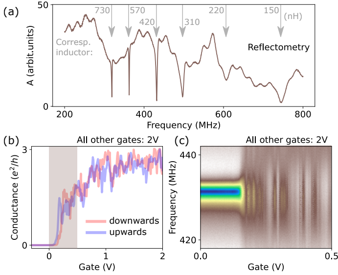
Figure 3.6: Basic characterization prior to measurements. (a) Reflectometry test result when six resonators on the MUX resonator chip are bonded to the target device. The corresponding inductor of each resonator is labelled above. It shows that the higher inductance gives a lower resonance frequency and a sharper dip in the amplitude signal. Those resonances at higher frequency range can be identified by comparing two results with different gate settings. (b) The conductance measured by lock-in amplifier when sweeping one single gate from 2 V to -0.3 V (red) and from -0.3 V to 2 V (blue). It indicates the nanowire can be opened with all gates set to 2 V and reaches the conductance of about 3 e^2/h , and the sweeping gate has limited hysteresis while pinching off the conductance successfully. (c) The conductance pinch-off of the same gate as the shadowed area in (b) can be detected by a resonator coupled to the contact lead, where the open wire significantly changes the reflectometry signal. It suggests that rf conductance measurements can replace transport measurements for characterisation.
