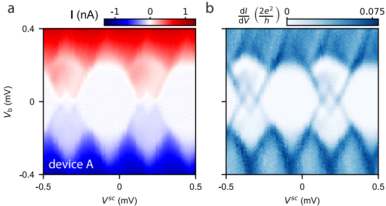
Figure 4.6: Coulomb blockade measurements of the superconducting island in device A. Left panel: current data, right panel: differential conductance obtained by taking the numerical derivative of the current data.
