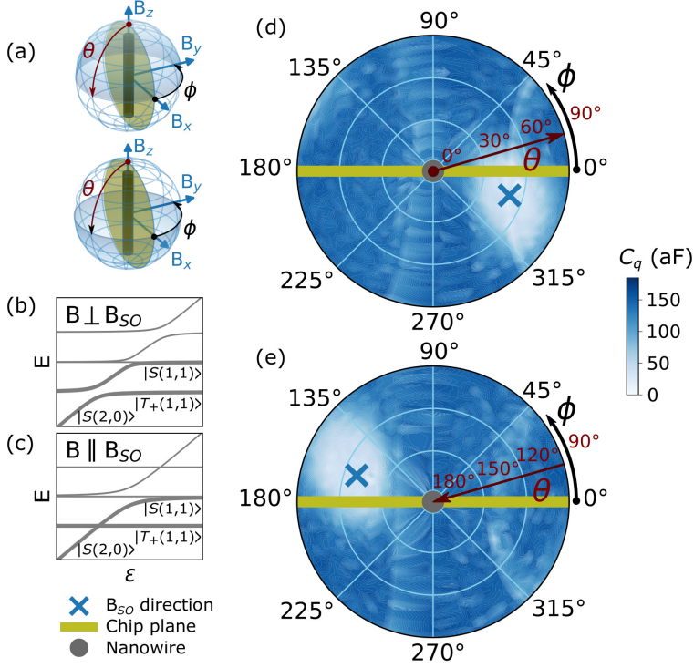
Figure 5.3: (a) Illustration of spherical coordinates with respect to the nanowire and the substrate. The top and bottom panel correspond to (d) and (e) respectively. (b-c) Schematic energy diagrams of a DQD for (b) \vec{B} \perp \vec{B}_{SO} and (c) \vec{B} \parallel \vec{B}_{SO} . The (avoided) crossing between the two lowest states are highlighted. C_{q,max} = 0 when they cross, due to the flat shape of |T_+(1,1)\rangle . (d-e) The extracted C_{q,max} values plotted on an external magnetic field angle map. Polar projection of the map is shown in (d) when 0^\circ \leq \theta \leq 90^\circ , and (e) when 90^\circ \leq \theta \leq 180^\circ . The blue crosses mark the characterized \pm \vec{B}_{SO} orientations, which is the center of the region where C_{q,max} is suppressed.
