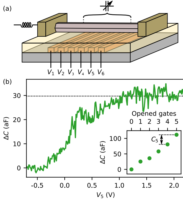
Figure 6.4: (a) A schematic of the InSb nanowire device with six parallel 80-nm-wide bottom gates, spaced by 60 nm. The coil symbol indicates the drain contact connected to a rf resonator. (b) Capacitance added to the circuit as a function of the voltage V_5 on one of the gates. (inset) Values of the added capacitance with 0 to 5 of the bottom gates in the open state. Error bars in the measured capacitance values are smaller than the marker size.
