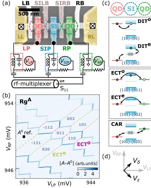
Figure 7.1: Device and the charge tunneling processes within the hybrid triple dot. (a) A false-colored SEM image of the device with gates labeled. The RF multiplexer concurrently transmits reflected gate sensing signals from resonators linked to each hybrid dot's plunger gate. (b) The charge stability diagram of the floating system, measured by the SIP resonator, is depicted in terms of |A - A^0| , representing the measured amplitude relative to that in the Coulomb blockade regime (indicated by the black square). The dot-island charge transitions (DIT) are clearly presented, with elastic cotunnelings (ECTs) not directly visible but indicated by dashed lines. The relative charge numbers of each dot n_i ( i = L, SC, R ) are annotated in the corresponding charge state regions as n_L n_{SC} n_R . (c) Illustrations of all relevant charge tunneling processes are provided, encompassing the DITs and ECTs with the island occupied by an even or odd number of charges, as well as crossed Andreev reflections (CARs). (d) A new set of axis, V_{\epsilon} and V_{\delta} , is illustrated in relation to the V_{LP} and V_{RP} axis. These axis will be utilized for the subsequent figures.
