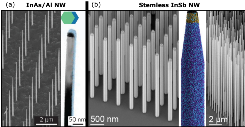
Figure 3.1: Nanowire (NW) growth chips. Tilted SEM images illustrating the nanowire growth chips, depicting InAs/Al nanowires with Al covering two facets in (a), and bare InSb nanowires in (b). Figures are adopted from Ref. [1, 2]
