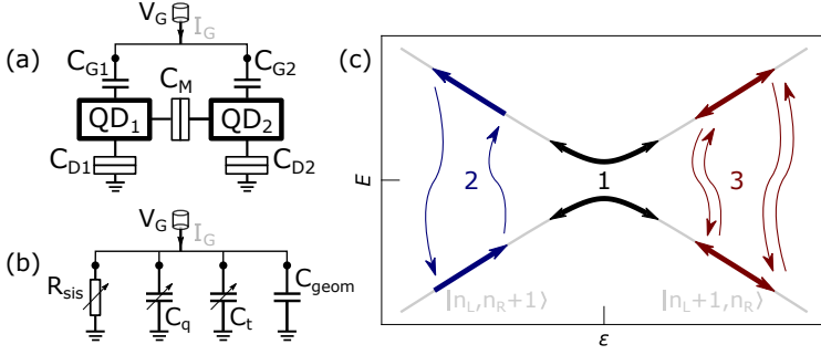
Figure 2.5: Equivalent circuit for a DQD and the relevant physical processes. (a) The DC version of equivalent circuit for a DQD seen from the gate electrode. (b) The AC version of the equivalent circuit for a DQD, including the quantum capacitance C_q , the tunneling capacitance C_t and the Sisyphus resistance R_{sis} . (c) The ground state energy and the excited state energy of the DQD as a function of the detuning. The arrows overlapping such energy states indicate the effects caused of an RF voltage source. The wiggly lines with arrows pointing down and up indicate phonon emission and absorption processes respectively. The sets of arrows labelled with numbers and different colors represent the origin of (1) C_q , (2) both R_{sis} and C_t , (3) pure C_t .
