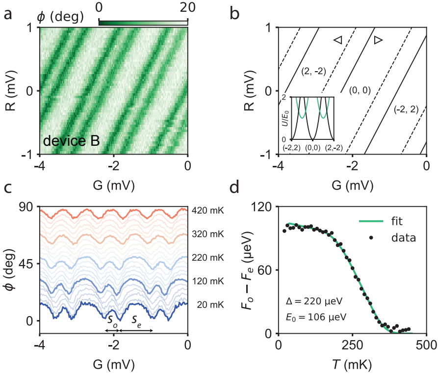
Figure 4.4: Re-enabling of single-particle tunneling in the floating regime a Charge stability diagram measured in phase in device B. The anti-diagonal lines indicate that the total charge in the system is conserved. b The calculated positions of the transitions in good agreement with the measured stability diagram. Inset: energy spectrum with the even states in black and the odd states in green showing that the even-odd pattern is caused by the parity effect even though E_0 > E_C^S . c Temperature dependence of the even-odd pattern. d The evolution of the free energy difference with temperature. The free energy difference is extracted from the even-odd pattern via F_0 - F_e = (S_e - S_0) e \alpha / 4 with \alpha = 0.9 the lever arm of G , and e the elementary electron charge.
