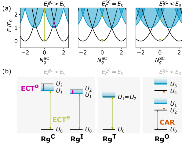
Figure 7.3: Energy spectra of the superconducting island for three typical scenarios. (a) The energy of the island, denoted as E , are determined as a function of the induced charge N_g^{SC} . The blue regions represent the continuum of states above the superconducting gap. The parabolas for the electron occupancy number N being even are shown in black. The yellow (pink) arrows depict the addition energy for introducing an extra quasiparticle to the superconducting island, depending on whether the island is occupied by even (odd) charge numbers. (b) The relative electrochemical potentials of a few superconducting island states, corresponding to the three scenarios in (a) and the four regimes in Fig. 7.2. The zero potential U_0 is defined in relation to the island being occupied by a even number of charges. The distance between the closest potentials U_{N+1} - U_N (also denoted by arrows) signifies the energy required to add an extra charge to the superconducting island. In the left panel, arrows labeled ECT e (ECT o ) depict the addition energy needed to reach the virtual state during the ECT process for even (odd) charge occupancies of the island. In the middle panel, the overlap of U_1 and U_2 implies no extra energy has to be paid for ECT o . In the right panel, with U_2 lower than U_1 , CARs become more energetically favorable, as indicated by the arrows.
