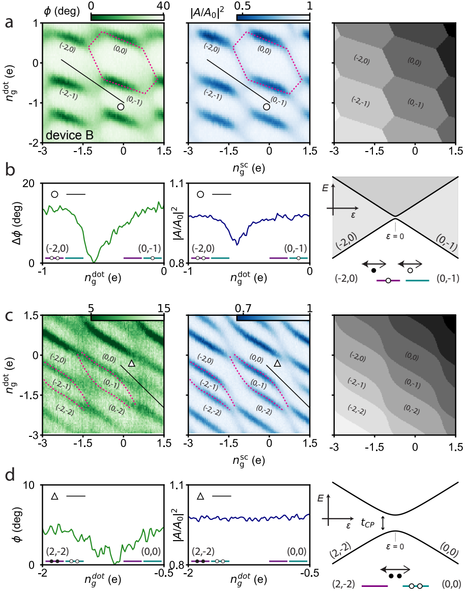
Figure 4.3: Cooper-pair tunneling in a hybrid double dot. a Charge stability diagram measured in phase (left) and amplitude (middle) along with a simulation of the charge ground state (right) in the weakly coupled regime. The charge states are labeled with (n_g^{SC}, n_g^{QD}) with respect to the state (N, M) with N even. Dashed pink lines: locations of the transitions from the (0,0) state as a guide to the eye. The gray scale in the simulation indicates the sum of the charge in the combined system. b Linecuts of the phase (green) and amplitude (blue) along the (-2,0) to (0,-1) interdot transition. This transition involves a reservoir with a continuous spectrum, indicated by the shaded region above the lowest available energy state. The schematic shows how these states couple via crossed Andreev reflection. c Same as in a for the strongly coupled regime. Dashed pink lines: locations of the lead transitions from the (-2,-1) and (0,-1) states as a guide to the eye. d Linecuts of the phase (green) and amplitude (blue) along the (-2,-2) to (0,0) interdot transition. These states couple via coherent Cooper-pair tunneling. All data is measured in device B.
