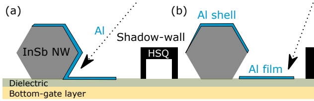
Figure 8.1: Shadow-wall technique on achieving (un)grounding superconducting segments. Cross-section of the InSb nanowire with (a) a small-angle deposition of aluminium, which allows either the grounding of the superconducting segment or the connections between individual islands along the nanowire. The shadow-wall is fabricated using a hydrogen silsesquioxane (HSQ) bilayer approach, which makes it easier to leave openings while reducing the geometric capacitance. (b) a large-angle deposition of aluminium that provides ungrounded islands. Here a single layer of HSQ shadow-wall is utilized.
