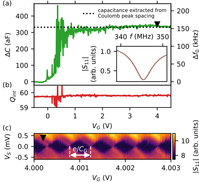
Figure 6.2: (a) Frequency shift, \Delta f , and a corresponding capacitance change, \Delta C , as a function of the plunger gate voltage V_G for 2- \mu\text{m} long InSb device. Dotted line indicates the gate capacitance extracted from Coulomb blockade measurement at V_G = 4 V, indicated with a triangular marker. Inset: |S_{11}| versus frequency at V_G = -0.5 V (solid line) and 4 V (dotted). (b) Internal quality factor Q_{int} of the resonator. (c) Rf Coulomb diamonds measurement. The periodicity of Coulomb blockade provides an independent measure of the gate capacitance.
