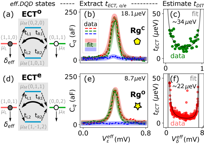
Figure 7.5: Tunneling strength of ECTs and DITs. (a) Schematic of an odd-island ECT process in Rg^C , with all relevant charge states labeled. The associated DIT processes are denoted as t_{L(R)1(2)} . The tunneling strength t_{ECT}^0 can be estimated by considering the system as an odd-occupied double quantum dot. (b) The data extracted from the linecuts with the pentagon marker in Fig. 7.4 (a). Fitting with the effective double dot interdot transition model in Eq 7.1, we estimate t_{ECT}^0 in Rg^C . The raw C_q data extracted from the three resonators are shown in dashed curves, while the fitted curves are represented by solid, slightly transparent curves of the same color. (c) The set of t_{ECT}^0 values plotted against V_\epsilon^{eff} , allows us to estimate the magnitude of t_{DIT} . The fitting curve follows Eq 7.2 is shown in grey. (d) Schematic of an even-island ECT process in Rg^O , similar to (a) but to consider the system as an even-occupied double quantum dot. (e) Similar to (b), but this time the data is extracted from the linecuts marked by the pentagram in Fig. 7.4 (a). Here, we estimate t_{ECT}^e in Rg^O . (f) Similar to (c), but focusing on fitting t_{ECT}^e in Rg^O .
