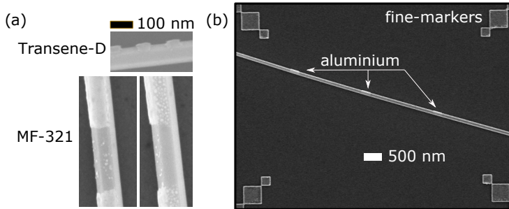
Figure 3.3: Aluminium etching. (a) SEM images of aluminium etching results using either Transene-D or MF-321. (b) SEM image of a nanowire that has undergone aluminium etching, leaving three aluminium sections behind.
