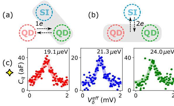
Figure 7.6: Tunneling strength of CARs. (a) When using the LP gate for sensing, the hybrid system is analogous to the left quantum dot being connected to an effective quantum dot comprising the middle island and the right quantum dot. The unit of charge transfer is 1e . (b) When using the SIP gate for sensing, the hybrid system is akin to the middle island being linked to an effective quantum dot consisting of the two outer dots. The unit of charge transfer is 2e . (c) The linecuts of a CAR detected by the LP, SIP and RP resonators as marked in Fig. 7.2 (d), with the corresponding estimated t_{CAR} values annotated. The data points depict the raw C_q data, while the solid transparent curves denote the fitting outcomes.
