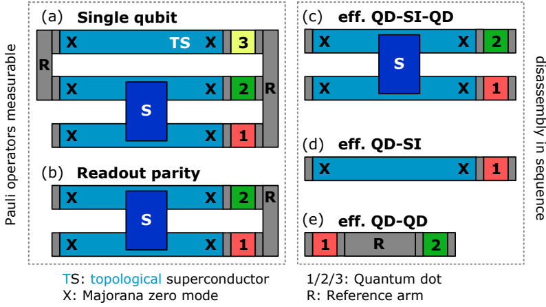
Figure 1.1: Majorana box qubit and its sequential disassembly. (a) Single Majorana box qubit for readout of all Pauli operators and full one-qubit control. (b) Interferometer that allowing parity readout of one pair of Majorana zero modes near quantum dot 1 and 2, equivalent to measure one Pauli operator \sigma_z . (c) By removing the reference arm, the structure effectively becomes a dot-island-dot system, leaving only one path for the charges to tunnel compared to (b). (d) Removing quantum dot 2 results in an effective dot-island system. (e) The other path for the charges to tunnel, as in (b). This is effectively a double quantum dot.
