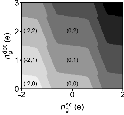
Figure 4.7: Simulation of the charge stability diagram of Fig. 2 of the main text. The gray scale indicates the total charge in the hybrid double dot.
