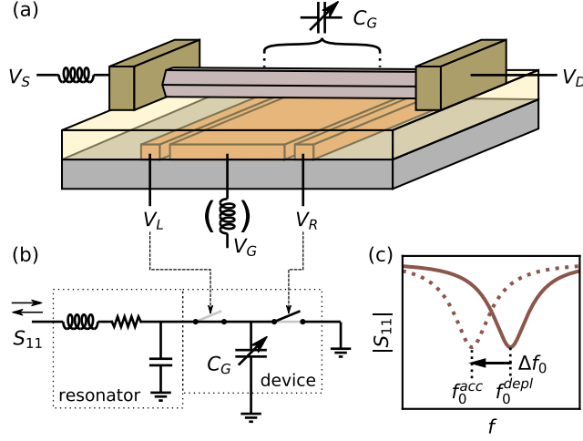
Figure 6.1: (a) Schematic of a bottom-gated nanowire device in a FET configuration. A source-drain voltage V_{SD} = V_S - V_D can be applied to measure the conductance of the device. Gate voltages V_{L/G/R} control the electron density in the semiconductor. C_G symbolizes the variable capacitance between the gate and the segment of the nanowire tuned by the gate voltage V_G . Coil symbols indicate contacts that can be connected to an rf resonator to perform capacitance measurements. (b) Schematic of the circuit for the capacitance measurement with the resonator attached to the device source contact. A lossy resonator is represented as an RLC circuit. The device is represented as two switches (tuned by gate voltages V_{L/R} ) and a variable capacitor. For a capacitance measurement the gate voltage V_L is set to accumulate charge carriers, while V_R is set to deplete them. (c) Illustration of the resonance frequency shift, measured in reflectometry, resulting from the accumulation of electrons in the nanowire. In the measured nanometer-scale devices the frequency shifts are typically much smaller than the resonance linewidth.
