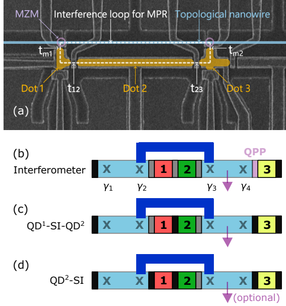
Figure 8.2: Parity readout measurements. (a) The SEM image of an achieved interferometer for parity readout, adopted from Ref. [8]. (b-d) An interferometer geometry for parity readout realized on a single nanowire, with the characterization of each component implemented by closing different barrier gates. The black (grey) barriers indicate that charge transitions are blocked (allowed). The grounding line is optional, depending on the purpose of the experiments. (b) An example of measuring a floating interferometer system based on a nanowire, equivalent to (a) and the schematic in Fig. 1.1 (b). The rightmost quantum dot is used for the purpose of studying quasiparticle poisoning, such that the barrier gate functions as a switch. (c) An example for measuring a floating dot-island-dot system. With a grounded superconductor, we obtain a minimal Kitaev chain connects to zero lead. (d) An example for measuring a floating dot-island system. When the superconductor is grounded, the quasiparticle poisoning rate can be detected.
