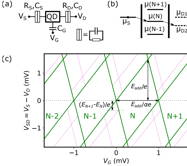
Figure 2.1: Single quantum dot (QD). (a) The equivalent circuit model of a single QD involves connections to the source ( V_S ) and drain ( V_D ) reservoirs through tunnel barriers. These barriers are represented in the model as a resistor R_{S(D)} in parallel with a capacitor C_{S(D)} . The gate voltage V_G is capacitively coupled to the QD through a capacitor C_G to adjust its electrochemical potential, thereby regulating the facilitation of charge transport at specific bias voltages. (b) The schematic of charge tunneling between the reservoirs through a QD. At zero bias, where \mu_S = \mu_{D1} , the transport is blockaded when the electrochemical potential \mu of the QD is misaligned with the Fermi level of the reservoir. At a finite bias, where \mu_S > \mu_N > \mu_{D2} , the single charge state begins facilitating the transport of charges through the QD. (c) By sweeping the voltages across multiple charge transitions, the Coulomb blockade regions manifest on the bias voltage V_{SD} versus V_G map as Coulomb diamonds. The addition energy E_{add} and the lever arm \alpha are indicated in relation to the width and height of the Coulomb diamonds. The transport through excited states is represented by pink lines. The energy spacing (E_{N+1} - E_N) can be determined by analyzing the height of their intersection with the boundary of the Coulomb diamonds.
