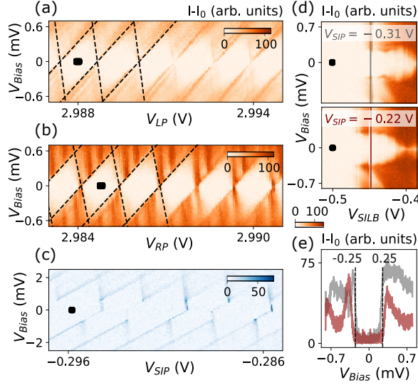
Figure 7.8: Coulomb diamonds of each hybrid quantum dot and the characterization of the superconducting island. (a) The Coulomb diamond of the left quantum dot, measured in the relative in-phase values ( I - I_0 ) via the resonator couple to the left lead. The black square marks where the in-phase value of the Coulomb blockade regime ( I_0 ) is selected and averaged. (b) The Coulomb diamond of the right quantum dot, similar to (a) but measured via the resonator couple to the right lead. (c) The Coulomb diamond of the middle superconducting island, similar to (a) but measured via the SIP resonator (therefore plotted in blue colormap). (d) Tunneling spectroscopy from the left side of the island with V_{SIP} = -0.31 V and -0.22 V, measured by the lead resonator. The vertical cuts with grey and brown colors corresponds to the V_{SILB} gate at -0.448 V. (e) The linecuts of (d) when V_{SILB} = -0.448 V, illustrating clearly a hard gap for a relatively large range of V_{SIP} , at least between -0.31 V and -0.22 V. The estimated gap size is slightly over 0.25 meV, as marked by the verticle lines.
