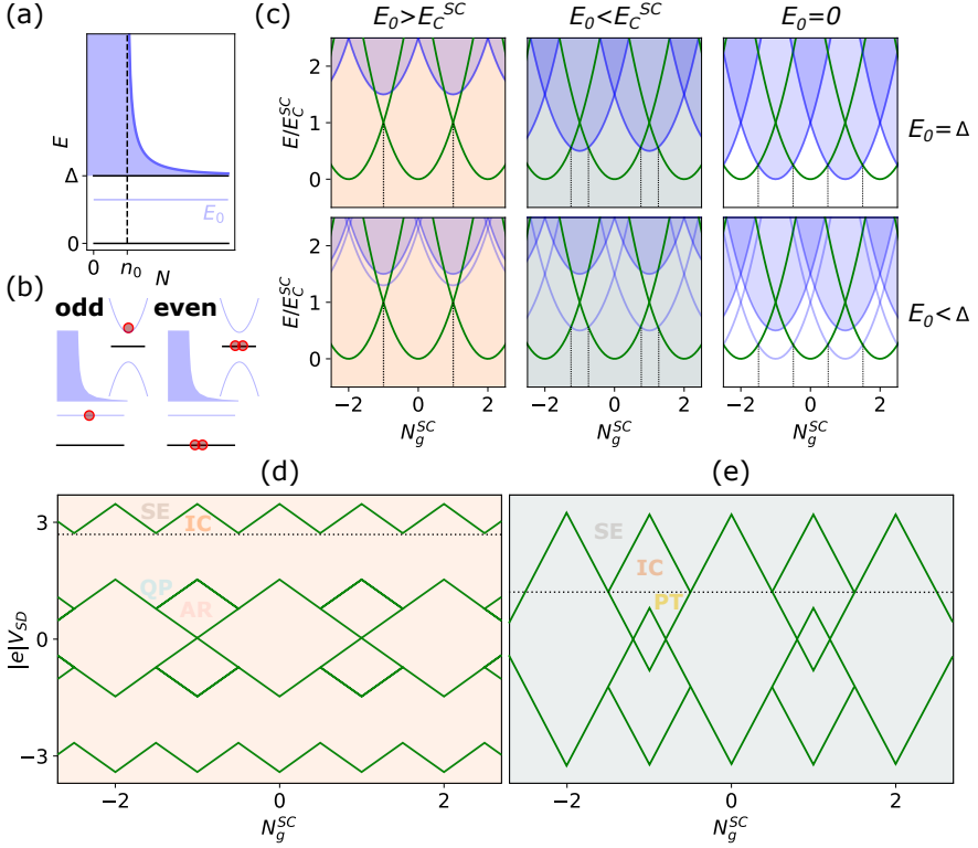
Figure 2.3: Single superconducting island. (a) Density of states in superconductors. When E < \Delta , all states below the gap in a normal metal are shifted to higher energy levels above the gap in a superconducting state, unless the gap is "soft" and there exist subgap states. We expect a sharp increase in state density just above E = \Delta , and N(E) \approx n_0 when E \gg \Delta , meaning it gets close to the density of electron states for a normal metal. (b) A schematic showing the different cases when odd or even electrons stay in a superconducting island. (c) The energy dispersions of a single superconducting island, exhibiting the parity effect. The top (bottom) row corresponds to the island with (without) subgap states. The left column represents when E_0 > E_C^{SC} , there we obtain a 2e-periodic ground state with only Cooper pairs allowed to transfer. The middle column represents when E_0 < E_C^{SC} , there the even or odd charge states can be distinguished from the alternating spacing of the ground state. The right column represents when E_0 = 0 , there we obtain a 1e-periodic ground state with single quasi-particles tunneling permitted. The Coulomb diamonds for a superconducting island with transport regimes, (d) for E_0 > E_C^{SC} , and (e) for E_0 < E_C^{SC} . The black dashed lines mark the energy equals to 2\Delta . For the sake of simplicity, processes involving three or more electrons are neglected.
