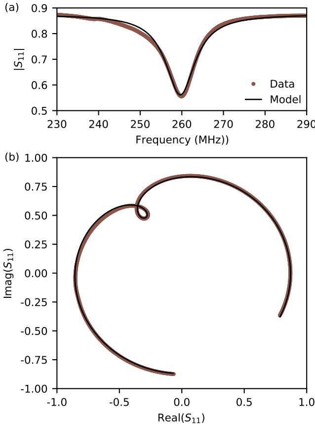
Figure 6.9: (a) Magnitude of the reflection around the self-resonance frequency of the surface mount inductor. (b) Parametric plot of the real and imaginary part of the reflection around the self resonance-frequency. Black lines indicate the fit to the data.
