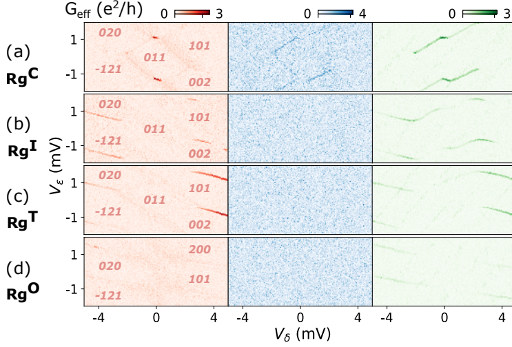
Figure 7.7: The Sisyphus dissipation of the tunneling processes. The effective conductance G_{\text{eff}} is extracted to show the Sisyphus dissipation on the charge stability diagrams of the four regimes. Larger G_{\text{eff}} indicates larger losses for the corresponding charge tunneling process.
