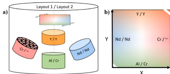
Fig. 1. a) schematic drawing of the sputter coater with the orientation of each source with respect to film orientation. Two layouts were used to acquire the desired concentration gradients. A mask was used on Cr for films with a low Cr concentration. b) The orientation of the films for each measurement with colour gradients to indicate the expected concentration gradient for each element.
