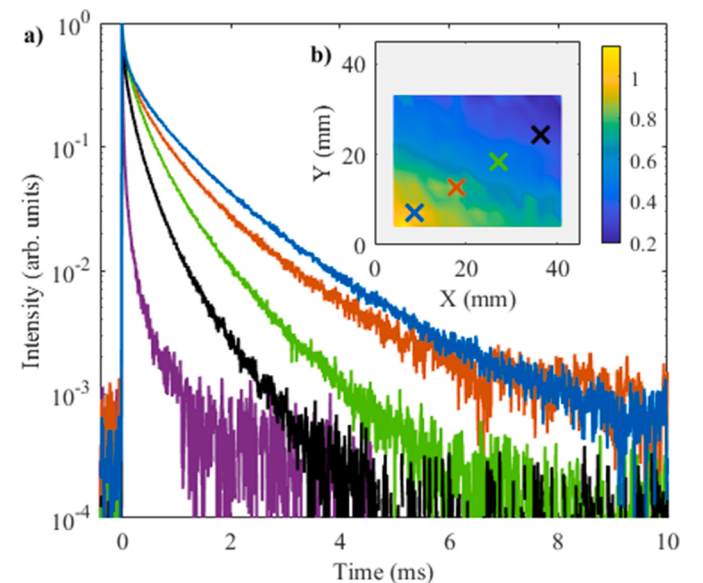
Fig. 9. a) Cr^{3+} lifetime measurements for \lambda_{em} = 707 nm with \lambda_{ex} = 430 nm of CR02 taken at the position indicated by the marker with their corresponding color in b). One measurement of the Cr^{3+} lifetime in CR03 is shown in purple, where the Cr content is 1.5 at.%. b) heat map of the radiative lifetime across the film.
