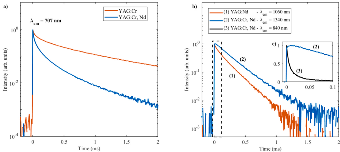
Fig. 11. a) Radiative lifetime of the \text{Cr}^{3+} R-line + ( \lambda_{\text{em}} = 707 nm) in single doped YAG: \text{Cr}^{3+} and double doped YAG: \text{Cr}^{3+} , \text{Nd}^{3+} with \lambda_{\text{ex}} = 620 nm. b) Radiative lifetime of the \text{Nd}^{3+} ^4\text{F}_{3/2} manifold ( \lambda_{\text{em}} = 1060 and 1340 nm) in single doped YAG: \text{Nd}^{3+} and double doped YAG: \text{Cr}^{3+} , \text{Nd}^{3+} with \lambda_{\text{ex}} = 588 nm and \lambda_{\text{ex}} = 620 nm respectively. c) A shorter timeframe that includes the radiative lifetime of the broad \text{Cr}^{3+} emission around 840 nm in YAG: \text{Cr}^{3+} , \text{Nd}^{3+} with \lambda_{\text{ex}} = 620 nm. All measurements were taken at locations with a YAG stoichiometry of x = 0.05 as shown in Fig. 2c.
