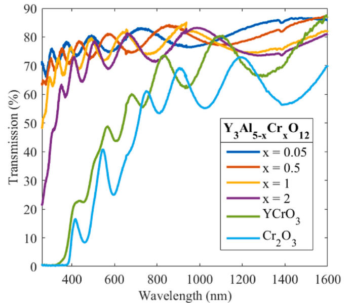
Fig. 5. Transmission spectra taken from samples CR04-CR09. The specific positions on the films of the measurements for CR04-CR07 are shown via the vertical markers in Fig. 2e–h. At wavelengths 655 and 933 there are discontinuities due to artefacts caused by an intense sharp peak from the deuterium light source and combining the spectra from two separate spectrometer respectively.
