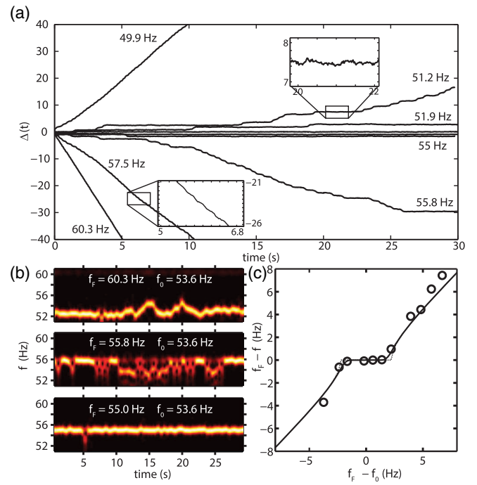
FIG. 2 (color online). Experimental data for one data set. The same cell is subject to an external flow A_F = 5 \mu\text{m} and f_F = 49.9 –60.3 Hz. (a) Time variations of the phase difference between the flagella and the external flow for separate recordings. Inset for f_F = 57.5 Hz shows a stepwise decay of \Delta(t) . Inset for f_F = 51.2 Hz shows fluctuations during phase locking. (b) Spectrograms of flagellar motion for different f_F . Black (white) correspond to a low (high) amplitude in the frequency spectrum. From top: no synchrony ( f_F = 60.3 Hz), partial locking ( f_F = 55.8 Hz), and complete phase locking ( f_F = 55.0 Hz). (c) f_F - f as a function of f_F - f_0 : Symbols, experimental data; solid line, f is computed from Eq. (4) with the fitted values for f_0 , \epsilon_0 , and T_{\text{eff}} ; dotted line, f is computed from Eq. (4) in the limit of zero noise.
