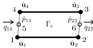
Fig. 7. Element schematic that contains pressures DoFs.
