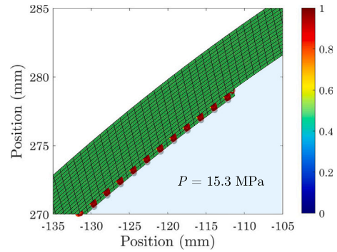
(b) Zoomed failure regions in the bottom 90° ply at 13.3 MPa.
