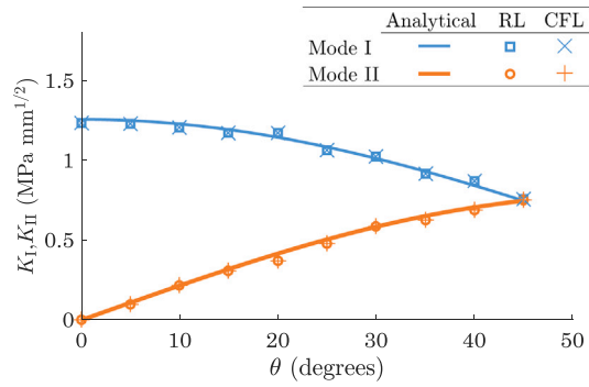
(b) Comparison between remote loading (RL) and crack face loading (CFL) for slant cracks.
