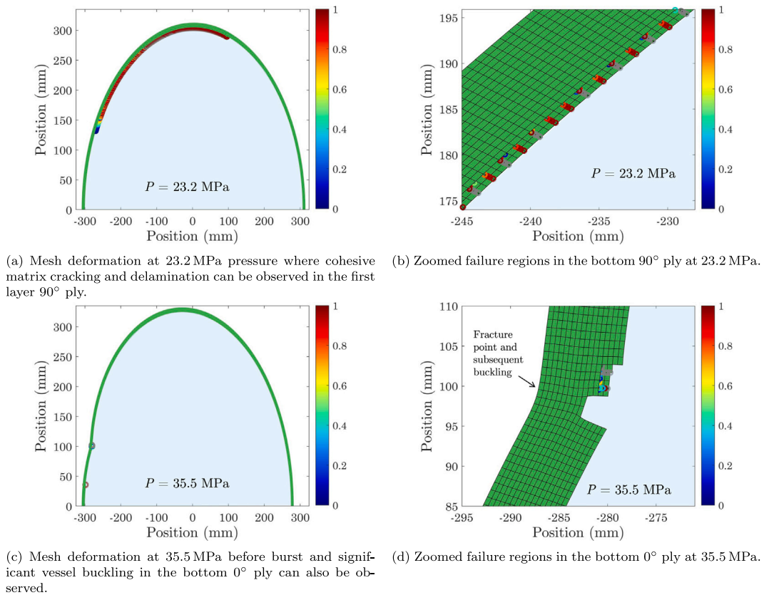
Fig. 21. Deformations and cohesive failure for the thick pressure vessel with 300 mm radius and 1 mm ply thickness; damage of the cohesive zones is presented with a colour bar (failed cohesive zones are shown with grey colour).
