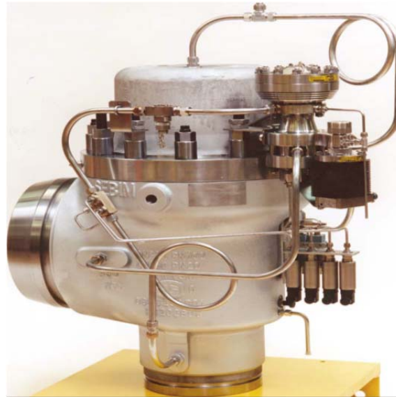
Figure 18: Tandem valve (IAEA, limited distribution a)
