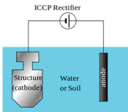
Figure 20: Cathodic protection (Wikipedia, 2018c)
