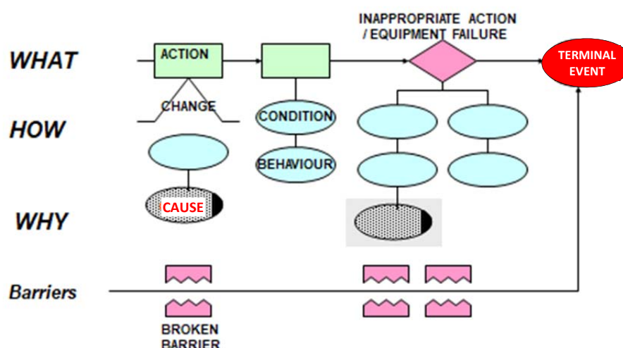
Figure 22: Event and causal factor charting (JRC, 2018)
