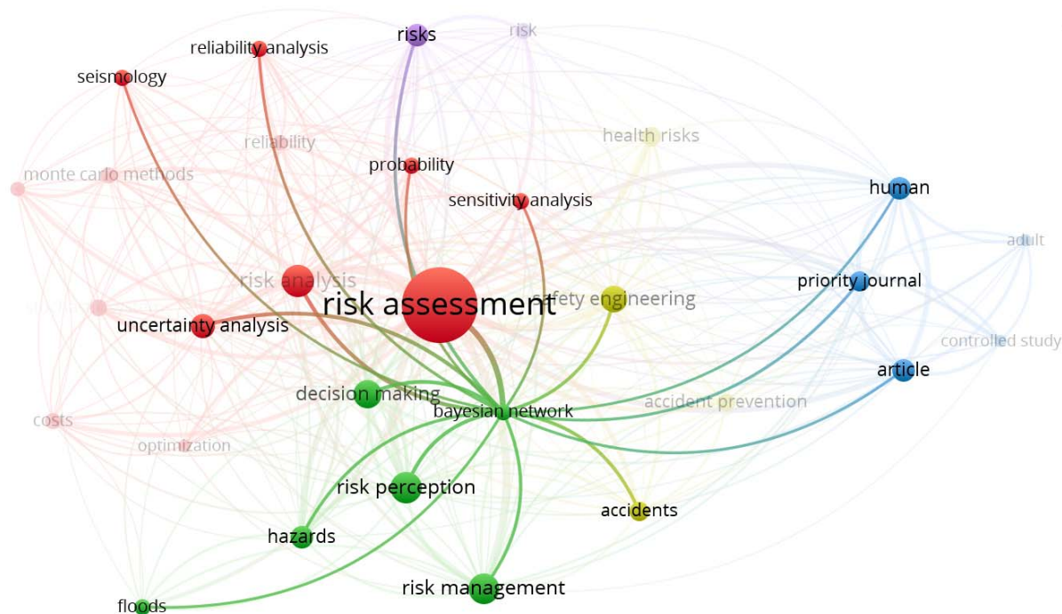
Figure 33: Most occurrences of keywords associated with "risk assessments" in engineering publications (top 30 occurrences among 2000 most relevant publications, based on data from the website www.scopus.com )
