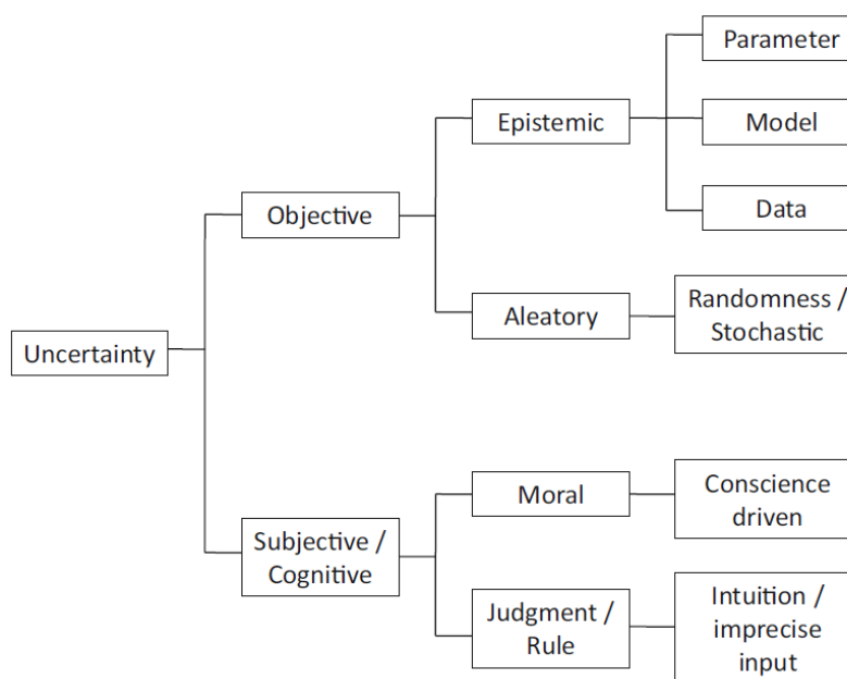
Figure 4: Taxonomy of uncertainty adopted for IRBE (Varde and Pecht, 2018)
