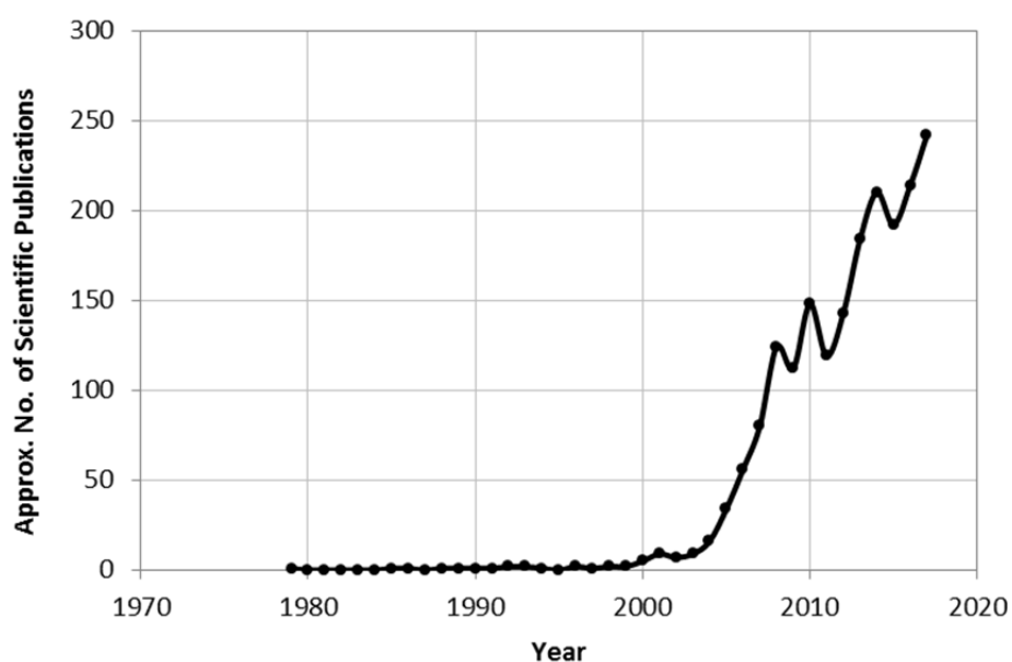
Figure 32: Approximate trend of publications of Bayesian networks used in engineering risk analysis contexts (based on data from the website www.scopus.com )
