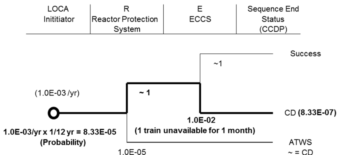
Figure 25: Conditional Core Damage Probability (CCDP)
