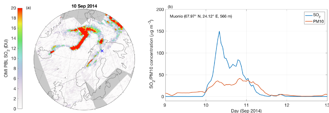
Figure 7. (a) Detection of \text{SO}_2 emissions from the Holuhraun (Iceland) eruption by the OMI very fast delivery (VFD) system on 10 September 2014. (b) Ground-based \text{SO}_2 measurements and breathable aerosols ( \text{PM}_{10} ) over Muonio measurement station (Finland; location indicated by a cross on the VFD image) from 9 September up until and 13 September 2014.
