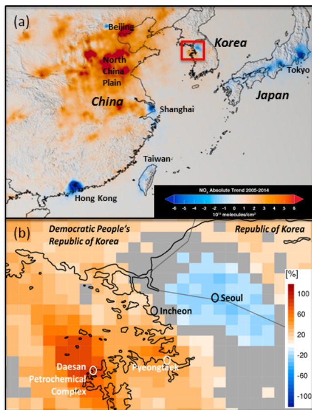
Figure 2. The world shows intriguing spatial heterogeneity and changes in air pollution from 2005 to 2014 in OMI NO 2 (Duncan et al., 2016), a common pollutant from power plants and automobiles. (Top panel) emission controls were implemented before 2010 in Japan, Taiwan, Beijing, Shanghai and Hong Kong, which led to decreasing trends in these regions and cities. Rapid growth until about 2011 in China's manufacturing heartland, the North China Plain, led to increases. Since 2011, levels there have begun to decrease following the gradual introduction of emission controls. The area outlined in red, the Seoul metropolitan area, is expanded in the bottom panel. (Bottom panel) ongoing retrieval algorithm work allows for unprecedented detail, including to sub-urban scales. The Seoul metropolitan area illustrates complex changes in OMI NO 2 from 2005 to 2014, which are likely associated with pollution emission controls in Seoul (decreases) and ambitious infrastructure development (increases) of the Incheon Free Economic Zone, Incheon International Airport, and the Daesan petrochemical complex.
