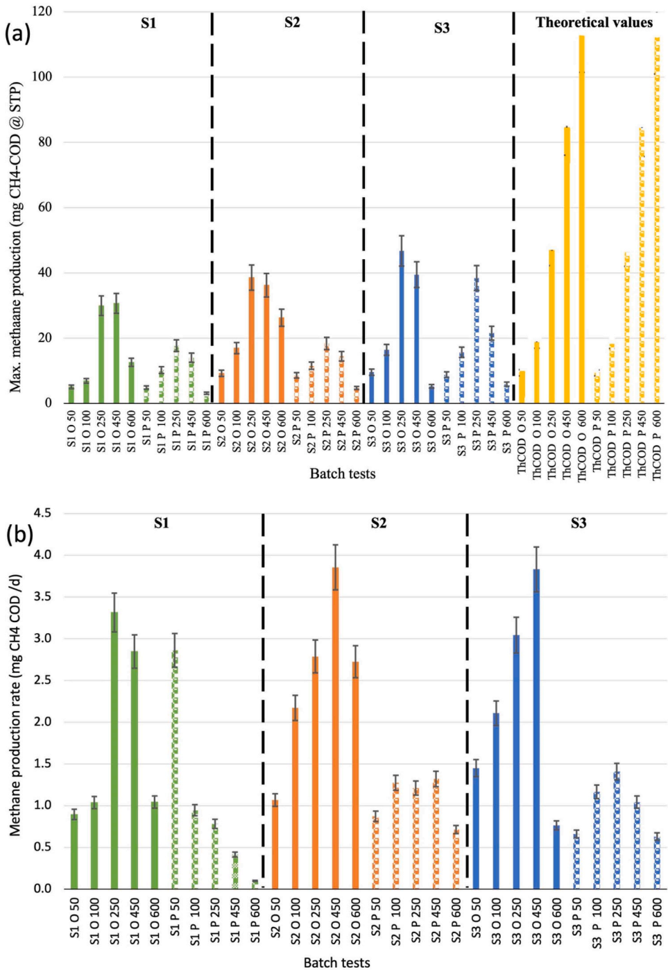
Fig. 2. (a) Maximum cumulative methane productions assessed with the PI sludge samples. S1: green; S2: orange; S3: blue. The solid color shows the experiments carried out with oleate, while the dashed color with palmitate. In yellow, the theoretical maximum cumulative methane productions based on the COD balance are shown; (b) Methane production rates for the PI sludge samples. S1: green; S2: orange; S3: blue. The solid color indicates oleate as the substrate, while the dashed color indicates palmitate. Average values are presented; the maximum standard deviation was 10% (not shown in the Figure).
