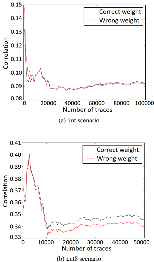
Figure 13: The correlation of correct and wrong weight hypotheses on different number of traces targeting the result of multiplication operation stored as different variable type: (a) int, (b) int8
