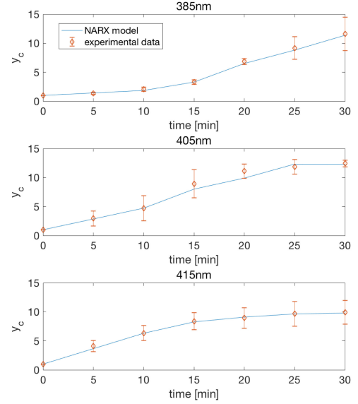
Fig. 3. The NARX model predicting the measured relative ROS concentrations in C. albicans from the 385, 405 and 415 nm light irradiation experiment, respectively.
