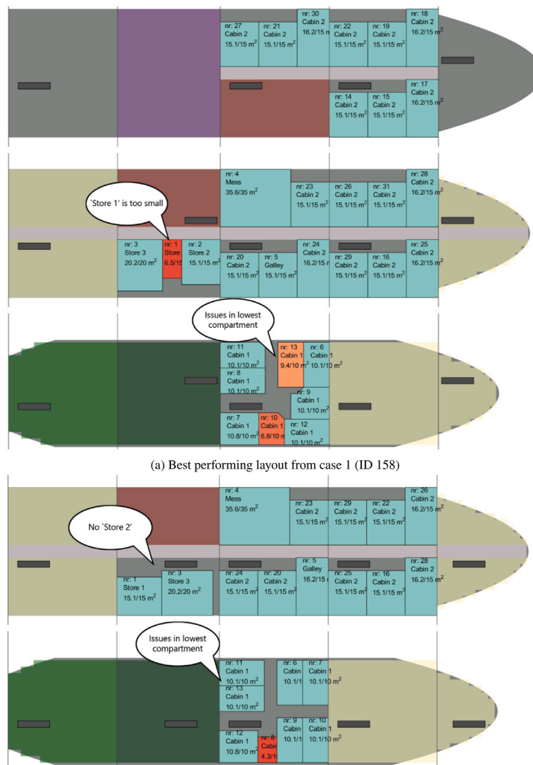
(b) Lowest two decks of the best performing layout that misses one space from case 1 (ID 55). The upper deck is arranged similarly as layout 158, Figure 15a.
