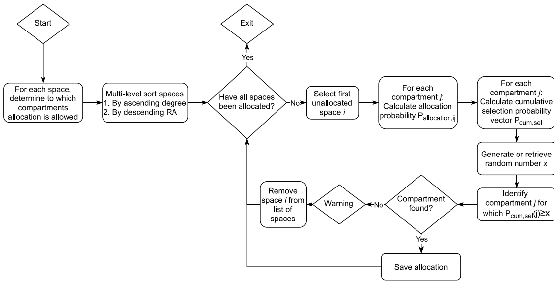
Fig. 7. Flow chart of the allocation of spaces to compartments.
