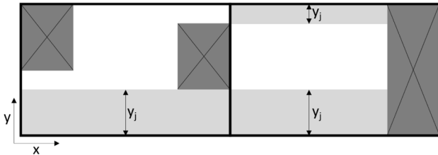
Fig. 2. Top view of a two compartment example on main passageway selection. Legend: dark grey, black cross: blocked area. light grey: available area for main longitudinal passageway. two-headed arrow indicate feasible y_j .
