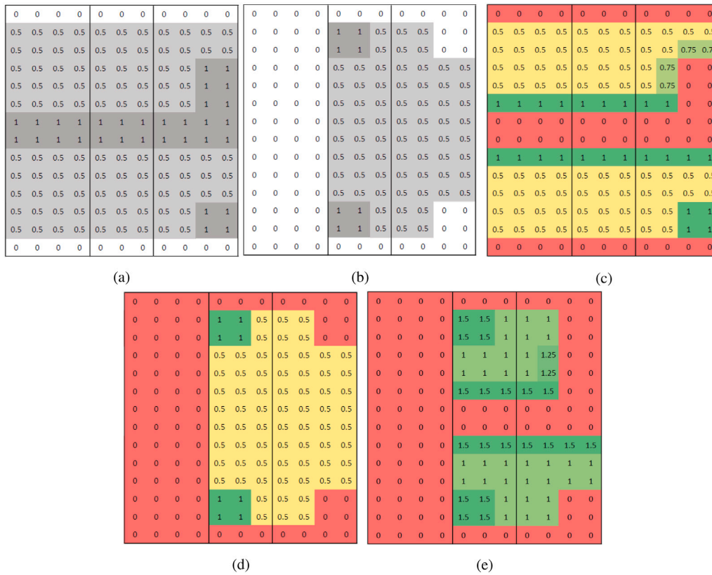
Fig. 4. Creating a staircase positioning matrix for a two-deck, three-compartment test case. (a) Deck 1 with an L-shape passageway and a small lobby. (b) Deck 2 with an irregular shape and two lobbies. (c) SPM_1 for deck 1. (d) SPM_2 for deck 2. (e) Aggregated FSPM for the two decks, where higher values represent more preferred positions for staircases.
