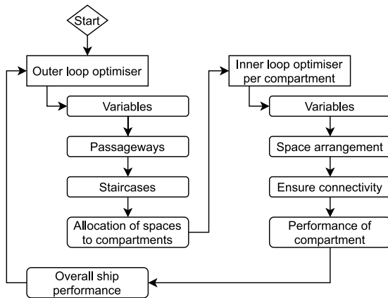
Fig. 12. Organisation of WARGEAR's mathematical methods inside a nested optimisation approach.
