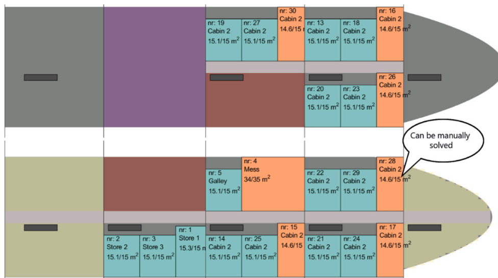
Fig. 16. Upper two decks of the best performing layout from case 2 (ID 58). The lowest deck was properly arranged.
