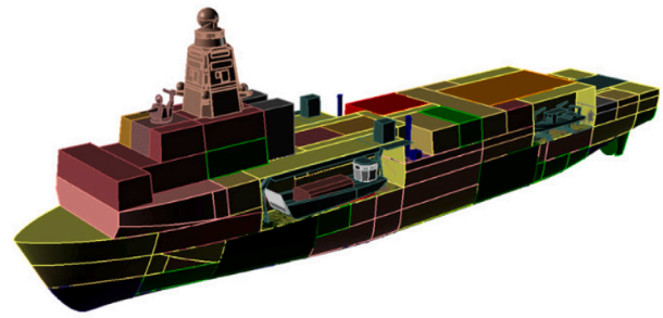
Fig. 1. An example of a functional arrangement (Van Oers, 2011a).
