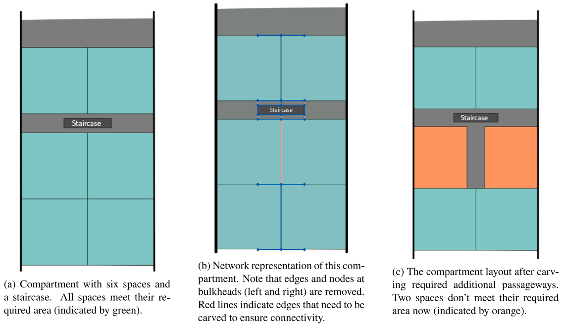
Fig. 11. Visual explanation of the carving process for a compartment with six spaces and a staircase.
