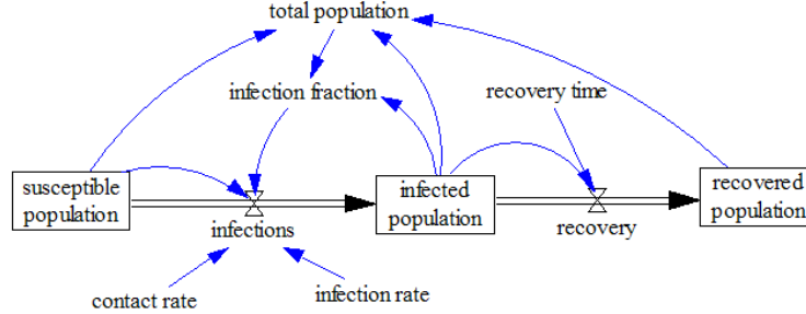
Figure 14: A SFD representing a SD simulation model
