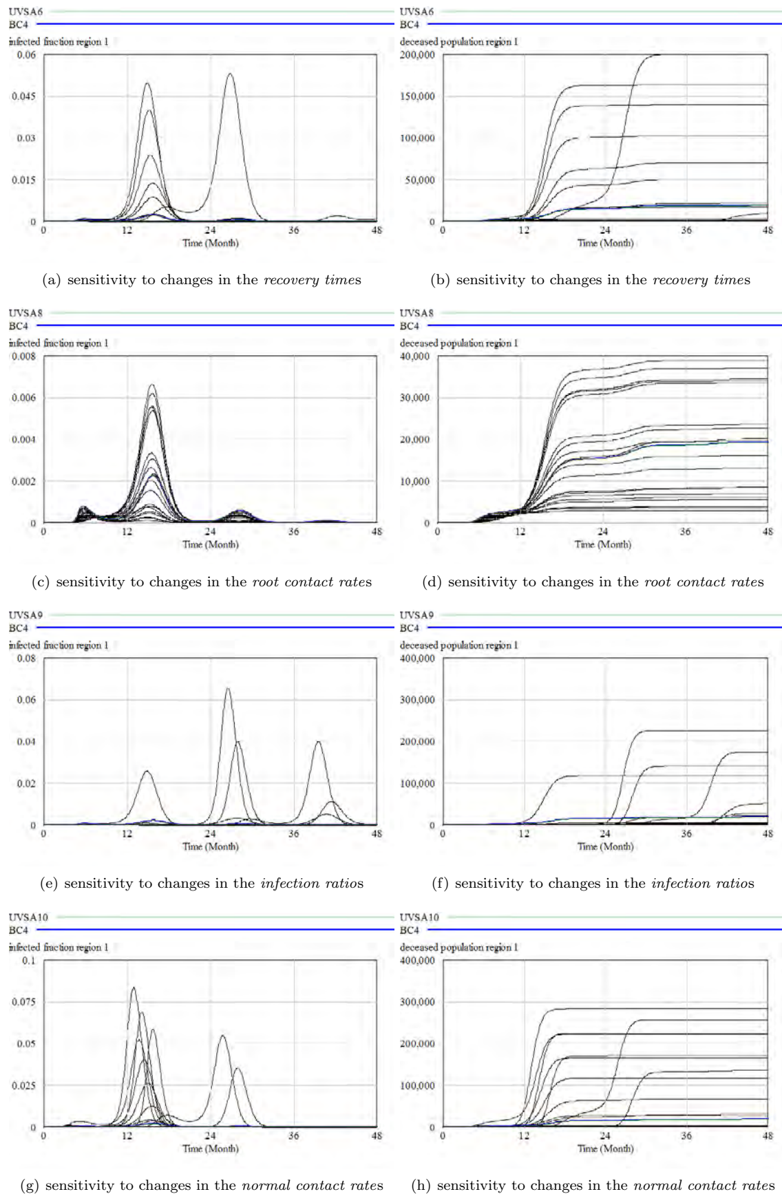
Figure 5: Univariate sensitivity analyses (2/2)
