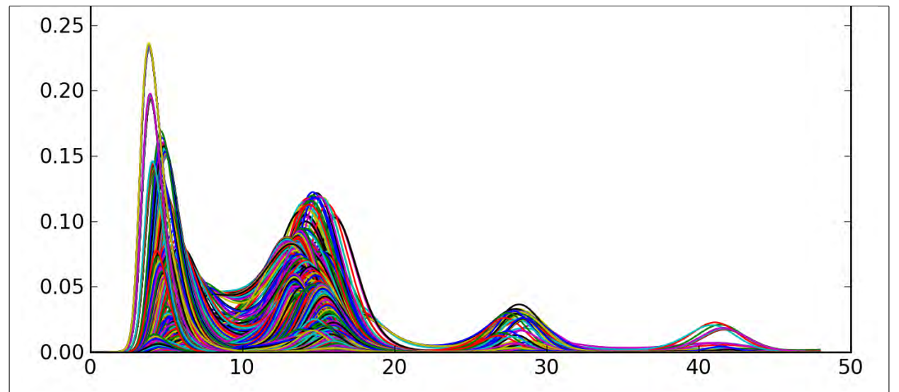
Figure C.2: Detail of the infected fraction (region 1) for infection rates of 0.10 (both regions 1 and 2)
