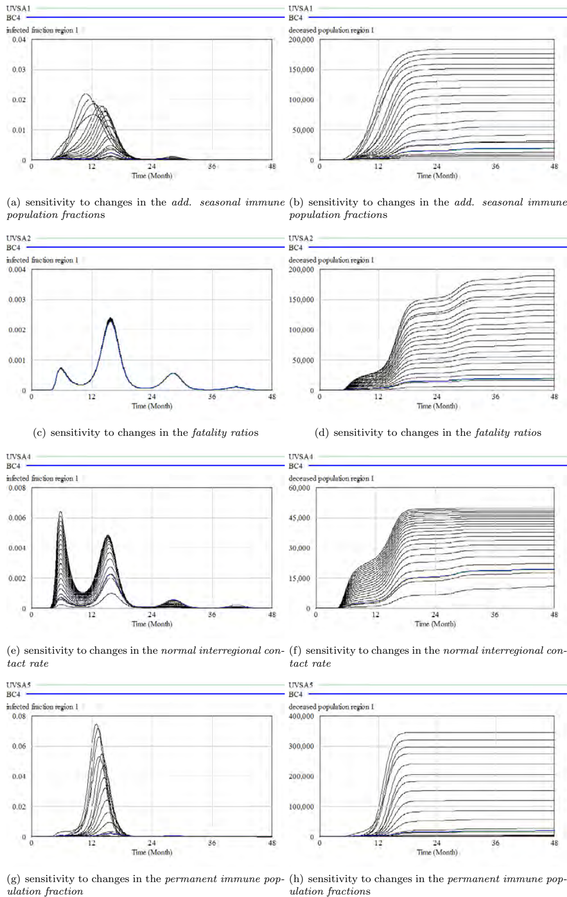
Figure 4: Univariate sensitivity analyses (1/2)
