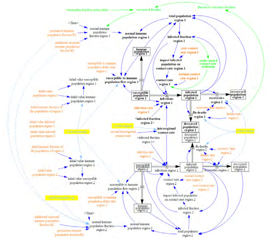
Figure 16: Stock-flow diagram of the ESD two-region flu model with the core structure for region 1 in bold (basic variables are displayed in black connected by dark blue arrows, initial values and parameters in orange, switches to turn structures of/off in light blue and yellow, and policy structures in green)
