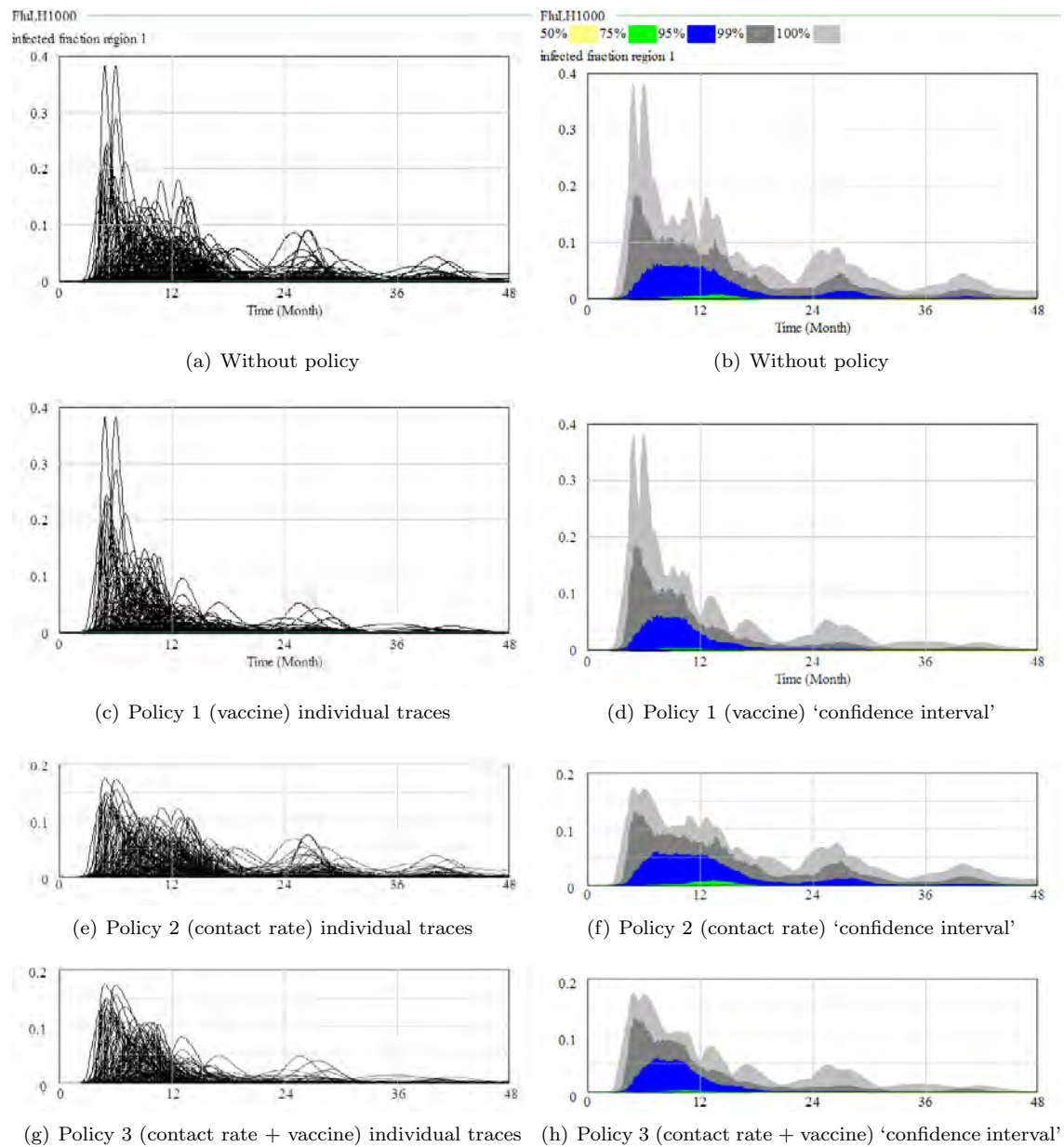
Figure 9: Quick and dirty ESD policy analysis of 3 dynamic policies
