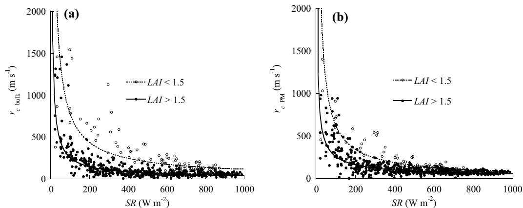
Fig. 7 Correlations of a r_{c \text{ bulk}} and SR b r_{c \text{ PM}} and SR in different rice-growing stages
