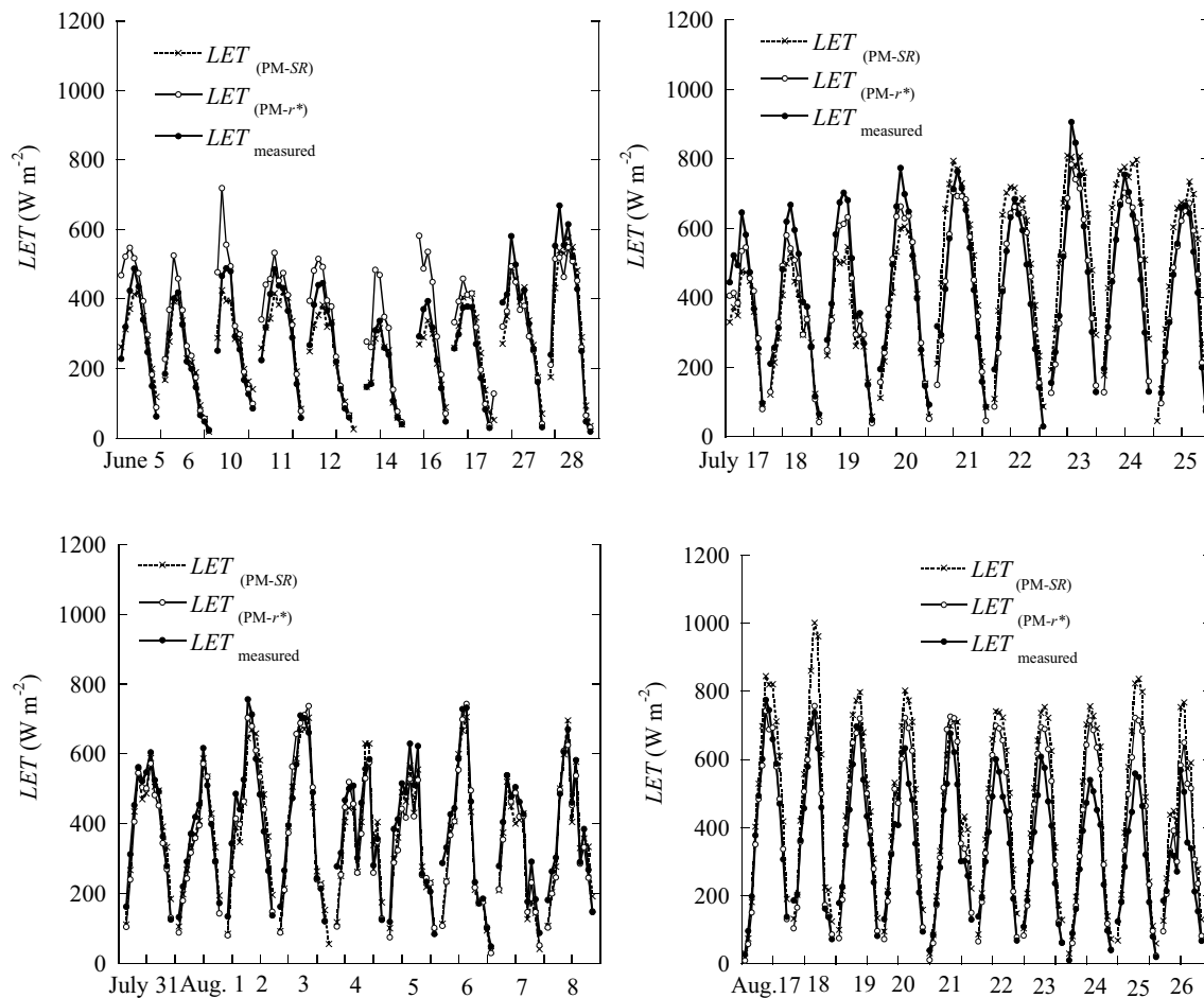
Fig. 9 Hourly variations of measured and modeled LET for paddy rice field; LET_{(PM-SR)} represents LET calculated from the Penman–Monteith equation with canopy resistance modeled by SR, while
