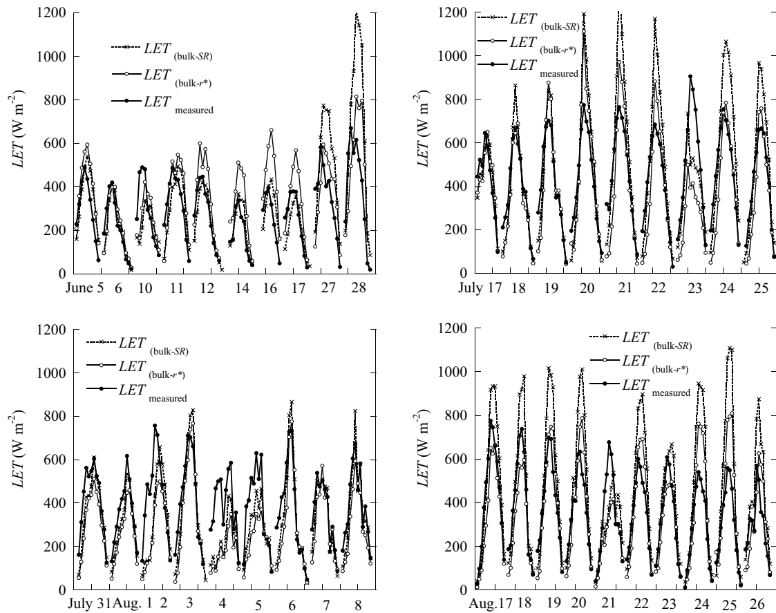
Fig. 8 Hourly variations of measured and modeled LET for paddy rice field; LET_{(bulk-SR)} represents LET calculated from the bulk transfer equation with canopy resistance modeled by SR, while LET_{(bulk-r^*)} represents LET calculated from the bulk transfer equation with canopy resistance modeled by r^* , and LET_{measured} represents LET measured by Bowen ratio–energy balance method
