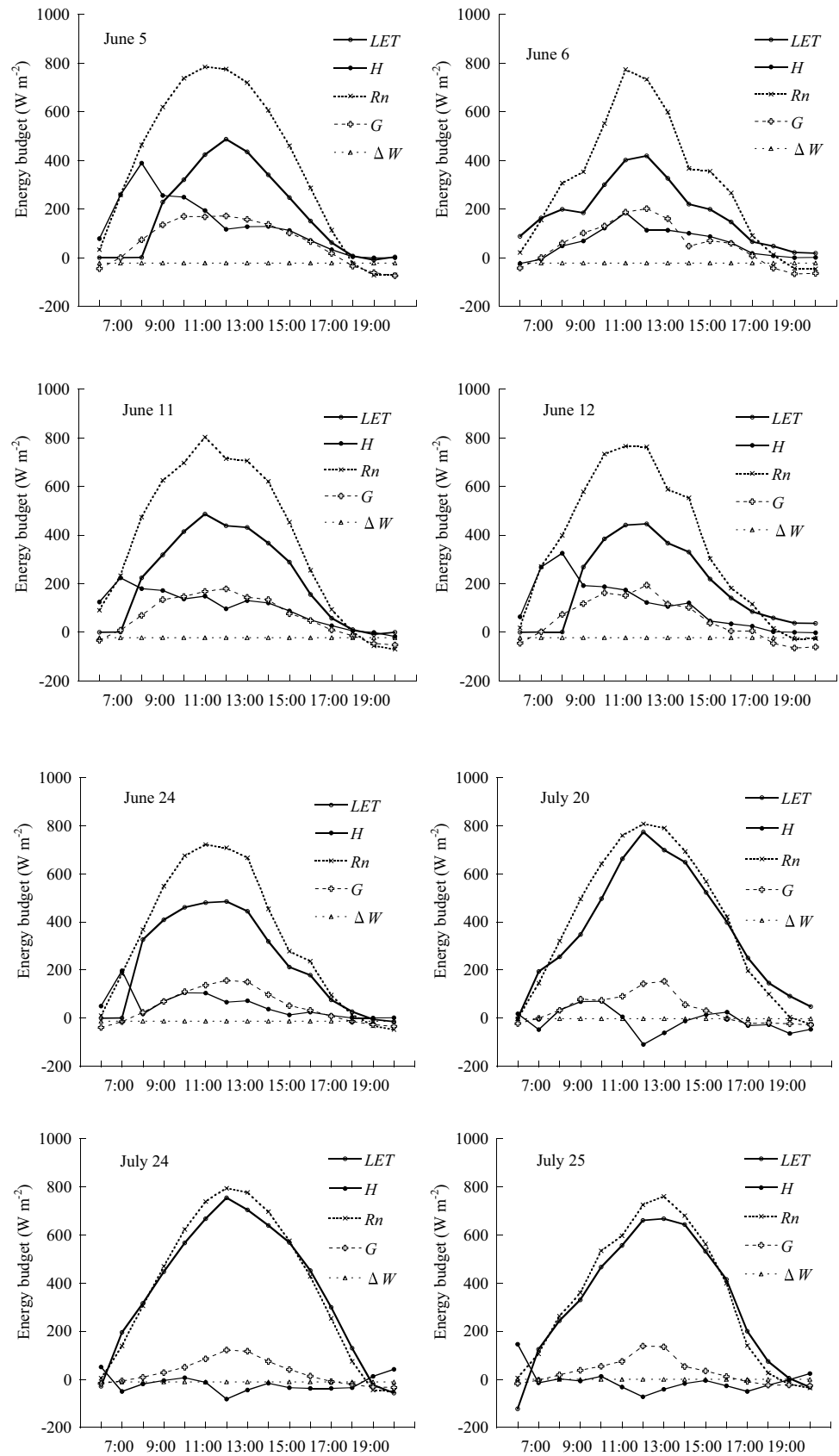
Fig. 3 Variations of energy partitioning for different growing stage of paddy rice
