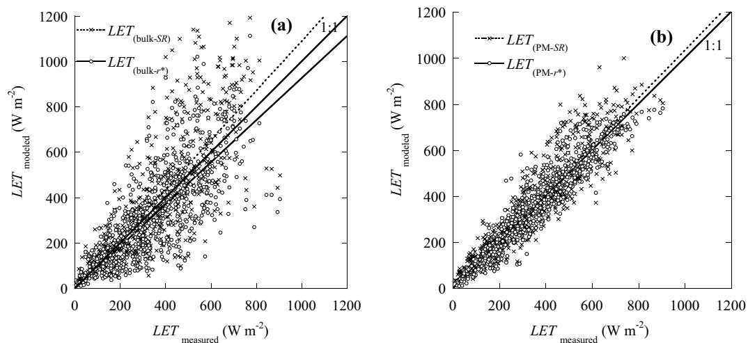
Fig. 10 Comparisons of a measured LET and modeled LET by the bulk transfer equation with canopy resistance from SR and r^* of rice paddy field, b measured LET and modeled LET by the Penman–Monteith equation with canopy resistance from SR and r^* of rice paddy field
