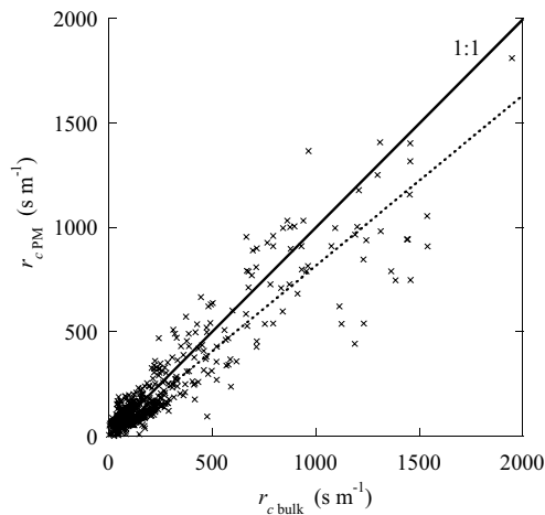
Fig. 4 Comparison of canopy resistance calculated by the Penman–Monteith ( r_{c\text{ PM}} ) and bulk transfer equation ( r_{c\text{ bulk}} )
