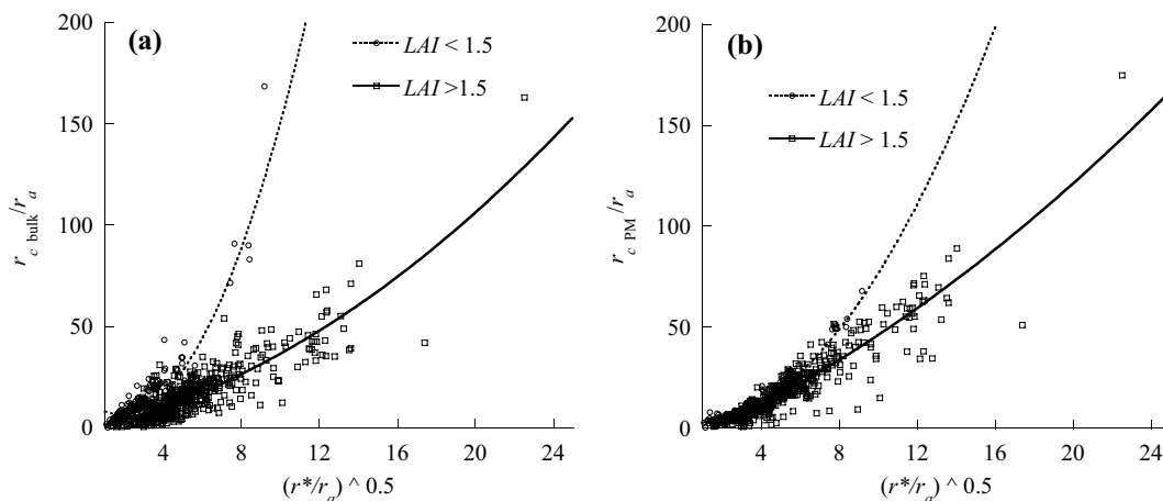
Fig. 6 Diurnal variation of experimental values of a r_{c \text{ bulk}}/r_a versus r^*/r_a , and b r_{c \text{ PM}}/r_a versus r^*/r_a on an hourly basis at paddy rice field, r_{c \text{ bulk}} and r_{c \text{ PM}} represent canopy resistance r_c calculated by the bulk transfer and Penman–Monteith methods, respectively
