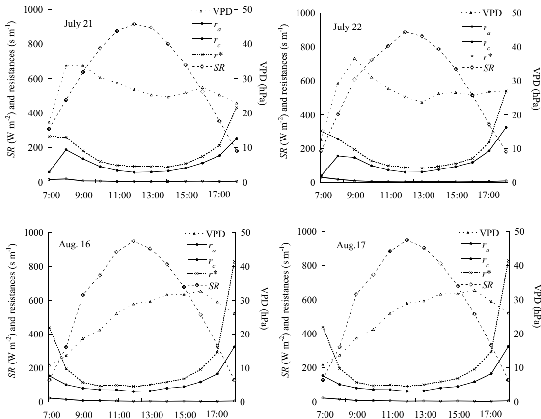
Fig. 5 Variations of aerodynamic resistance ( r_a ), canopy resistance ( r_c ), climatic resistance ( r^* ), SR and VPD at paddy rice field in four typical days (July 21–22, August 16–17)
