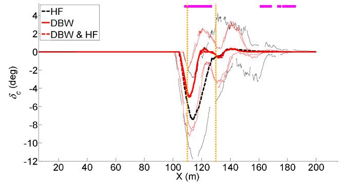
Fig. 8. Correcting angle \delta_c : medians (thick lines), and 5th and 95th (thin lines) percentiles. Vertical lines ( x=110 m and x=130 m) mark the first and last pylon that had to be avoided. Bars are visible on top when HF versus DBW & HF (magenta) and DBW versus DBW & HF (red) are statistically significant (only magenta bars are visible here).
