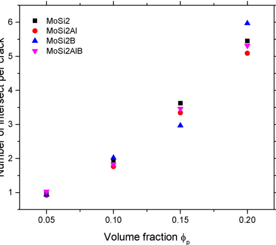
Fig. 8. Quantified crack – particle incidents as a function of volume fraction of particles having different chemical compositions embedded in YPSZ matrix.
