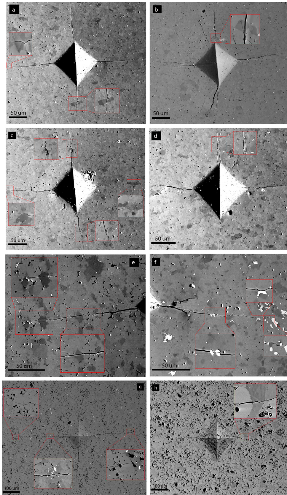
Fig. 6. SEM images of cracks propagating through bulk composite SPS samples containing: (a–b) 5, (c–d) 10, (e–f) 15 and (g–h) 20 vol.% of \text{MoSi}_2 . Insets show magnified areas where cracks pass through the particles.
