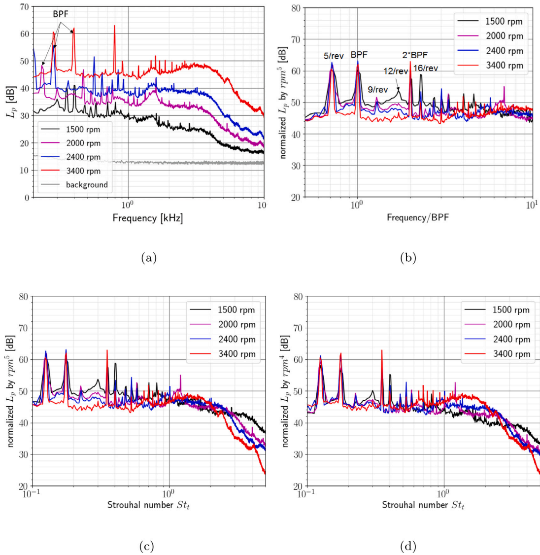
Fig. 9. Directivity results obtained at UdeS. (a) SPL of the antenna most-centered microphone at various rotational speeds. (b) Normalized SPL by \text{rpm}^5 versus frequency normalized by BPF. Normalized SPL by (c) \text{rpm}^5 and (d) \text{rpm}^4 versus the Strouhal number based on the tip chord.
