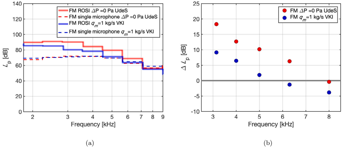
Fig. 13. Comparisons between the VKI FM-case operating at q_m = 1 \text{ kg s}^{-1} and the FM UdeS-case working at \Delta P = 0 Pa. (a) Integrated spectra (solid lines) and the single-microphone spectra (dashed lines); (b) relative differences of the reconstructed L_p by ROSI and that recorded by the microphone aligned with the center of the fan.
