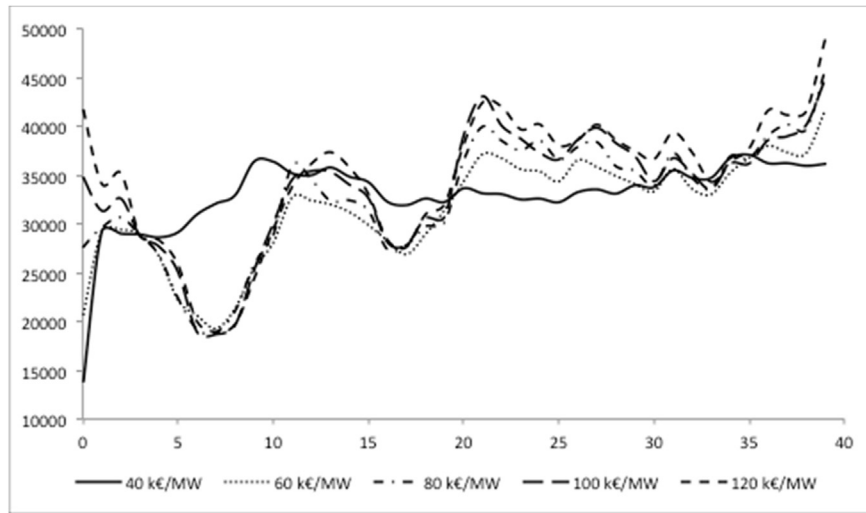
Fig. 18. Average capacity clearing prices in scenarios with different capacity price caps.
