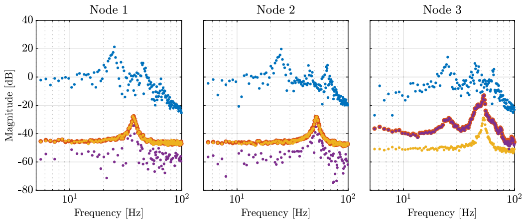
Fig. 9. Nonlinearity detection in the three-mass-spring-damper system using the node-to-node dynamics. The spectra of the node signals y_i(\omega_k) (•), the total distortion levels \sigma^2_{r,i}(\omega_k) (•), the distortions due to noise \sigma^2_{v,i}(\omega_k) (•), and the nonlinear distortions \sigma^2_{x,i}(\omega_k) (•), are depicted. Dominant nonlinear dynamics are observed at the third node since the nonlinear distortion is larger than the noise distortion.
