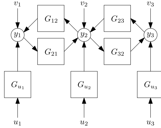
Fig. 1. A dynamic network consisting of three nodes, indicated with y_i , which are interconnected by dynamic subsystems G_{ij} and G_{u_i} . The node signals are calculated by summing all incoming signals. The exogenous incoming signals consist of the external inputs u_i and process noise contributions v_i .
