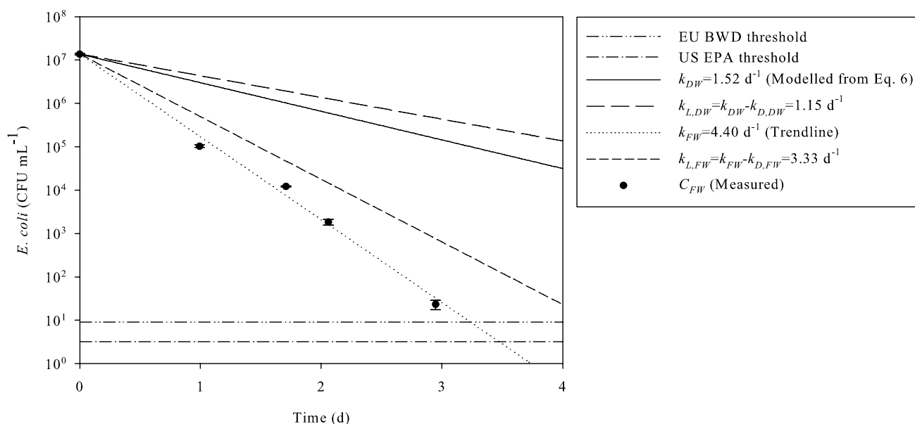
Fig. 3 The concentration of E. coli in artificial floodwater ( C_{FW} , with decay rate k_{FW} ) measured in the reactor, compared to the theoretical curve for demineralised water with k_{DW}=1.52\text{ d}^{-1} calculated from Eq. 6 for 150\text{ mg TSS L}^{-1} . The decay rates without the effect of dark inactivation for the two water qualities ( k_{L,FW} and k_{L,DW} , respectively)
