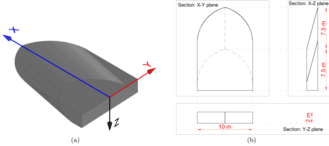
Figure 2: Geometric details of SHIELD (a) 3-D view and (b) cross-sections.
