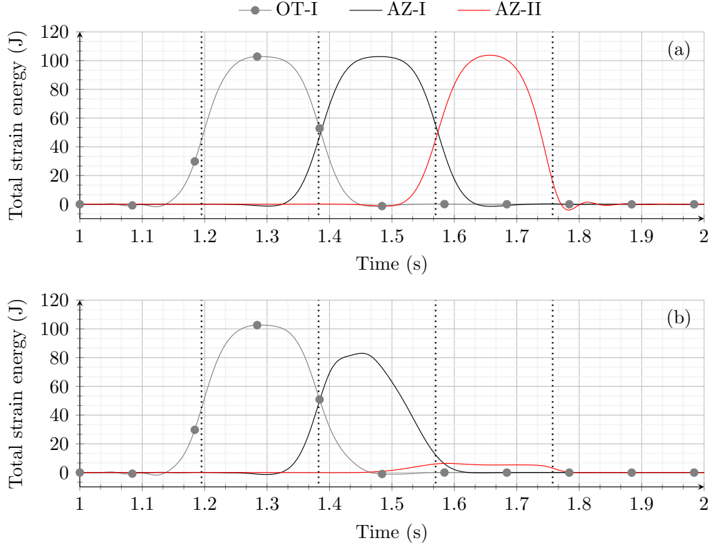
Figure 5: Time history of the total strain energy in the subgrade layer for a standard embankment-bridge transition (a) without and (b) with SHIELD.
