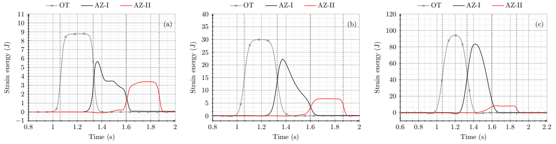
Figure 7: Time history of the total strain energy in the (a) ballast, (b) embankment and (c) subgrade layer for a standard embankment-bridge transition (equipped with SHIELD) without ballast layer over the bridge.
