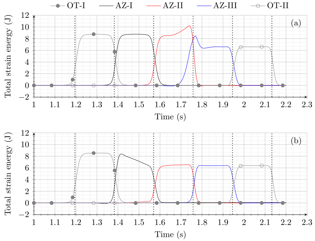
Figure 3: Time history of the total strain energy in the ballast layer for a standard embankment-bridge transition (a) without and (b) with SHIELD.
