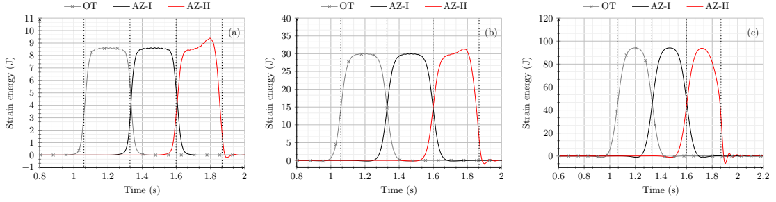
Figure 6: Time history of the total strain energy in the (a) ballast, (b) embankment and (c) subgrade layer for a standard embankment-bridge transition with ballast layer discontinued over the bridge.
