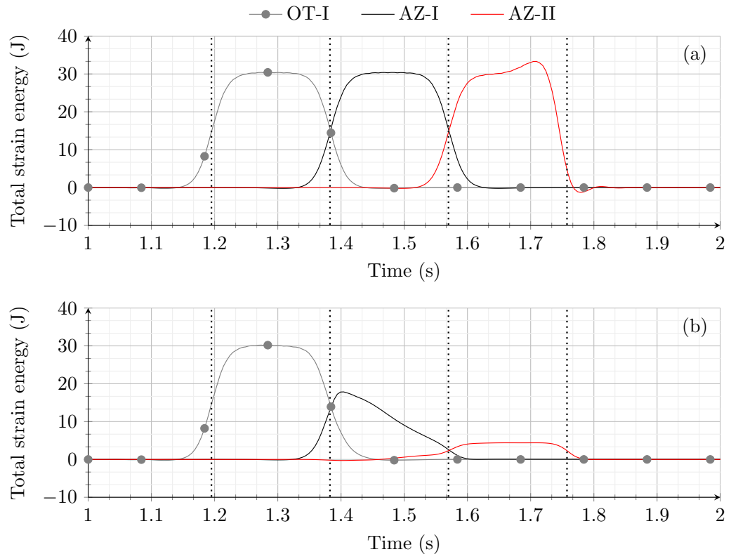
Figure 4: Time history of the total strain energy in the embankment layer for a standard embankment-bridge transition (a) without and (b) with SHIELD.
