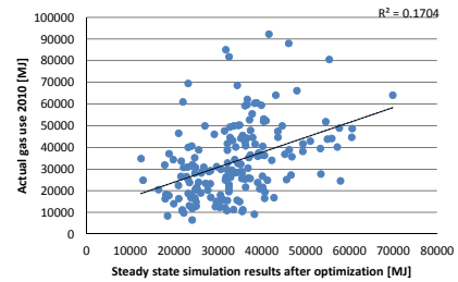
FIG. 5.24 Regression actual energy use versus dynamic simulated energy use after optimisation on control group
