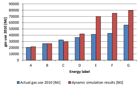
FIG. 5.6 Actual versus Theoretical gas consumption calculated with dynamic simulation method
