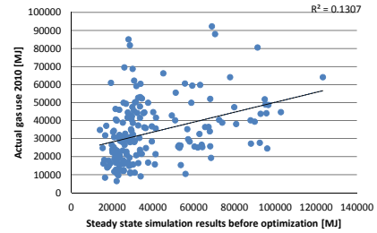
FIG. 5.22 Regression actual energy use versus dynamic simulated energy use before optimisation on control group
