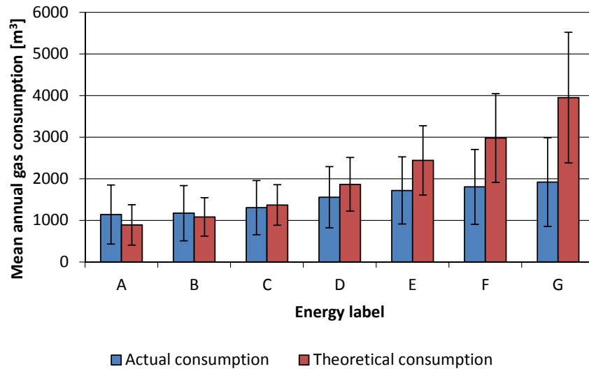
FIG. 5.1 Actual and theoretical gas per m 2 of dwellings consumption per energy label (Majcen et al., 2013) [4]
