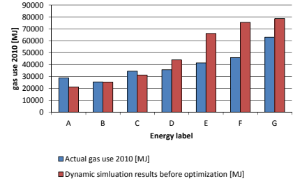
FIG. 6.11 comparison actual versus simulated gas consumption before optimisation (calculated with dynamic simulation method) , based on data from WoON energiemodule 2012
