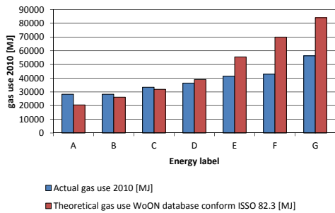
FIG. 5.5 Actual versus Theoretical gas consumption calculated with steady state simulation method
