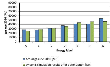
FIG. 6.13 comparison actual versus simulated gas consumption after optimisation (calculated with dynamic simulation method) , based on data from WoON energiemodule 2012
