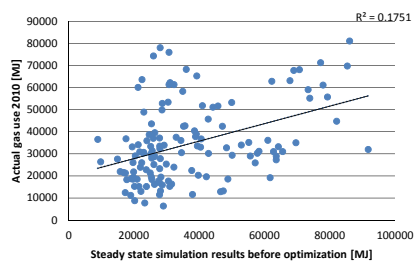
FIG. 5.9 Regression actual energy use versus steady state simulated energy use before optimisation on sample
