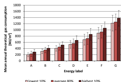
FIG. 6.3 comparing lowest, average and highest gas consuming groups actual consumption based on data SHAERE and CBS database 2014
