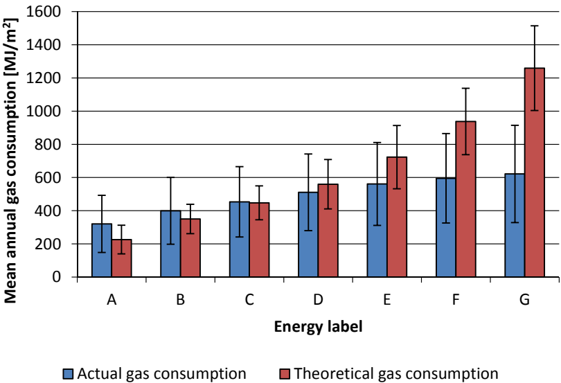
FIG. 6.1 Actual versus theoretical gas consumption per energy label based on data SHAERE database 2014
