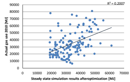
FIG. 5.12 Regression actual energy use versus dynamic simulated energy use after optimisation on sample
