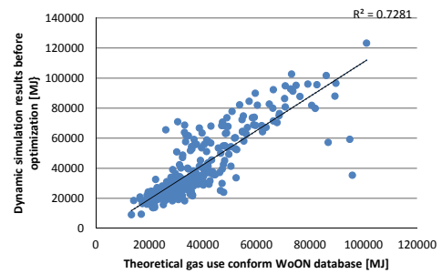
FIG. 5.4 Linear regression Theoretical energy use WoON database versus results dynamic simulation model
