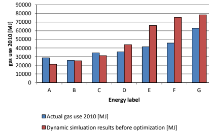
FIG. 5.14 Actual versus theoretical gas consumption calculated with dynamic simulation method before optimisation - sample
