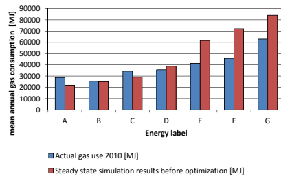
FIG. 5.13 Actual versus theoretical gas consumption calculated with steady state simulation method before optimisation - sample
