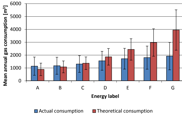
FIG. 1.2 Actual and theoretical gas per m 2 of dwellings consumption per energy label (Majcen et al., 2013)
