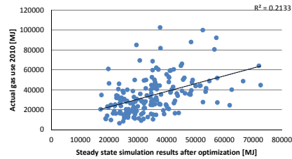
FIG. 5.23 Regression actual energy use versus steady state simulated energy use after optimisation on control group
