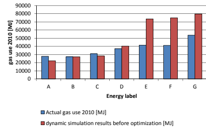
FIG. 5.18 Actual versus theoretical gas consumption calculated with dynamic simulation method before optimisation – control group
