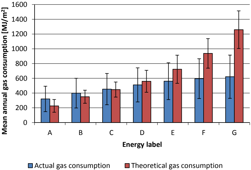
FIG. 2.1 Comparison of actual versus theoretical gas consumption per m2 (error bars show 1sd).
