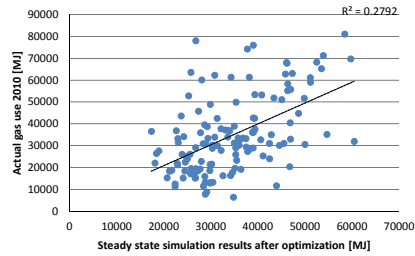
FIG. 5.11 Regression actual energy use versus steady state simulated energy use after optimisation on sample
