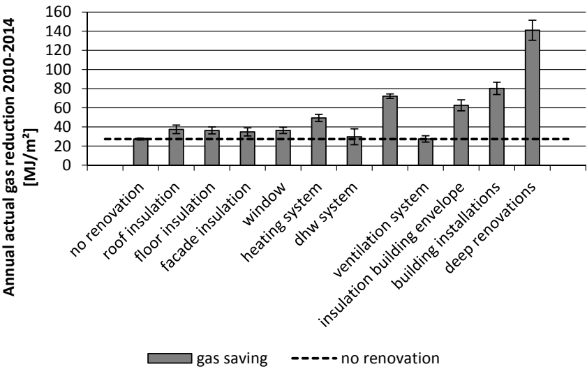
FIG. 6.4 Average energy saving per thermal renovation measure (including confidence interval 0.05), based on data SHAERE and CBS database 2010-2014 Note: Dashed line is actual difference in gas reduction between 2010–2014 for non-renovated houses.
