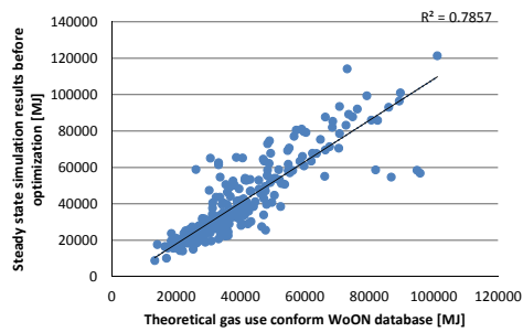
FIG. 5.3 Linear regression Theoretical energy use WoON database versus results steady state simulation model
