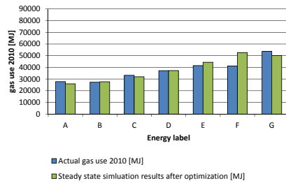
FIG. 5.19 Actual versus theoretical gas consumption calculated with steady state simulation method after optimisation – control group
