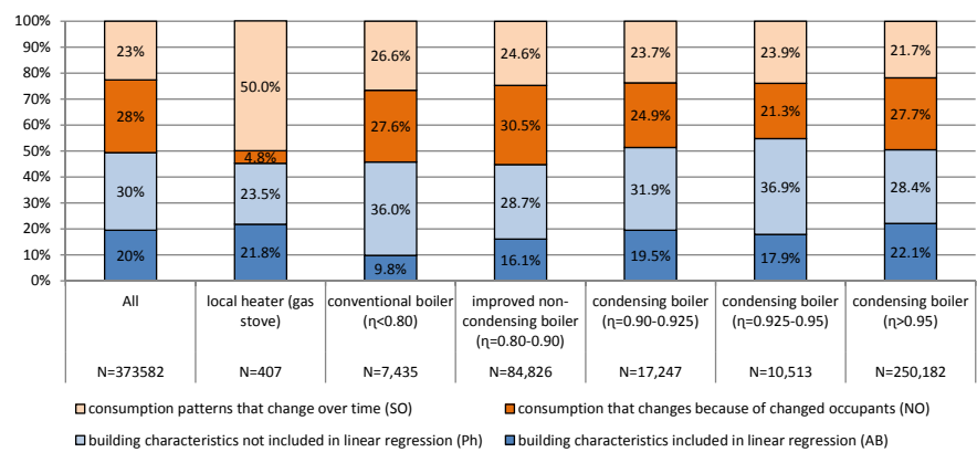
FIG. 4.8 Comparison of influence of building characteristics and occupants on variance energy consumption - Dutch data heating system
