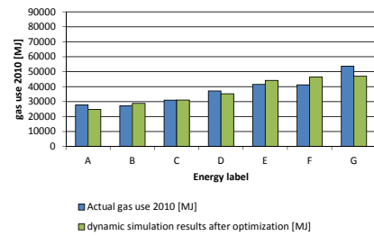
FIG. 5.20 Actual versus theoretical gas consumption calculated with dynamic simulation method after optimisation – control group
