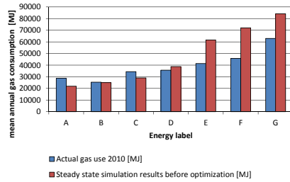
FIG. 6.10 comparison actual versus simulated gas consumption before optimisation (calculated with steady state simulation method) , based on data based on data from WoON energiemodule 2012
