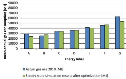
FIG. 5.15 Actual versus theoretical gas consumption calculated with steady state simulation method after optimisation – sample
