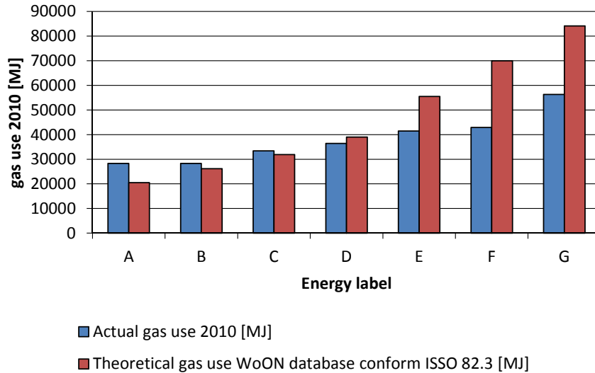
FIG. 5.2 Comparison of actual versus theoretical gas use in buildings based on the WoON database selected sample 313 cases (2012)
