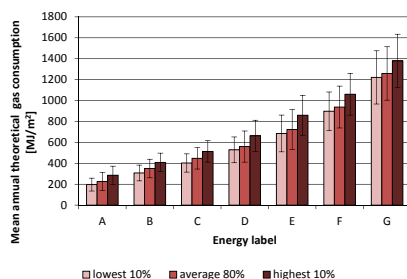
FIG. 2.4 Comparison of highest, average and lowest mean theoretical gas consumption per energy label.
