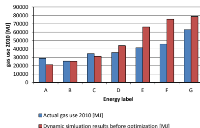
FIG. 6.8 comparison actual versus simulated gas consumption (calculated with dynamic method), based on data from WoON energiemodule 2012
