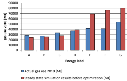
FIG. 5.17 Actual versus theoretical gas consumption calculated with steady state simulation method before optimisation – control group
