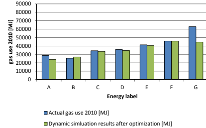
FIG. 5.16 Actual versus theoretical gas consumption calculated with dynamic simulation method after optimisation – sample
