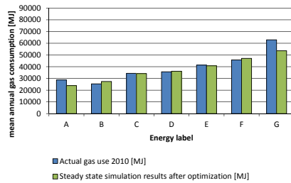
FIG. 6.12 comparison actual versus simulated gas consumption after optimisation (calculated with steady state simulation method) , based on data based on data from WoON energiemodule 2012
