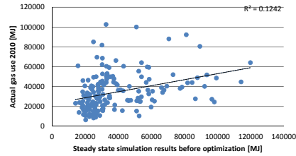
FIG. 5.21 Regression actual energy use versus steady state simulated energy use before optimisation on control group
