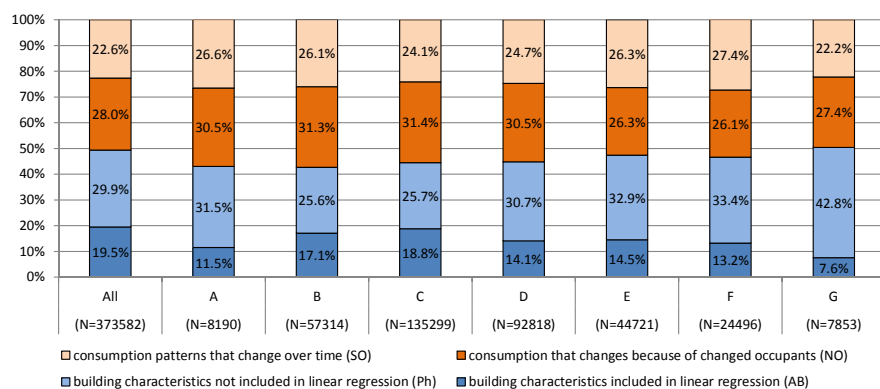
FIG. 4.3 Comparison of influence of building characteristics and occupants on variance energy consumption - Dutch data energy label
