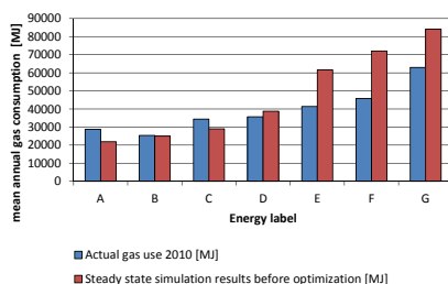
FIG. 6.7 comparison actual versus simulated gas consumption (calculated with steady state method), based on data from WoON energiemodule 2012)
