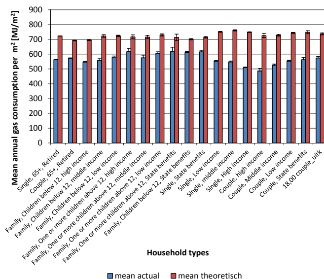
FIG. 2.3 Comparison of mean actual versus theoretical gas consumption per household group – energy label E.
