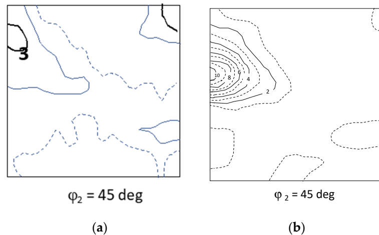
Figure 2. \varphi_2 = 45^\circ sections of (a) Ti-IF steel and (b) Mn-alloyed Ti-IF steel after austenitic hot rolling, partially below the T_{nr} temperature. ODFs extracted from [15].
