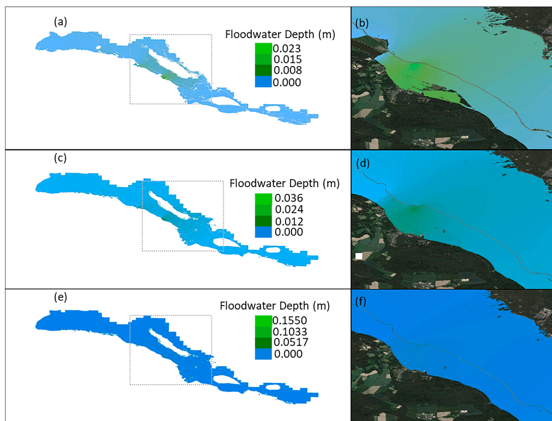
Fig. 6. Flood inundation/depth extents results for the historical (a and b), near-future (c and d), and far-future (e and f) under RCP 8.5. The results are showing the maximum flood depths reduced by the presence of NbS at midstream (b, d, f).
