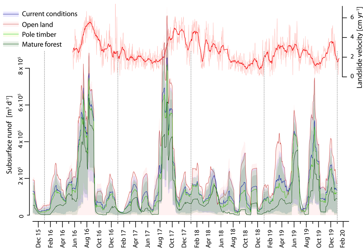
Fig. 3. Time series of simulated cumulated (30-day running sum) water surplus for different vegetation scenarios (pole timber, mature forest, current conditions and open land) in the catchment of OAL-AT and time series of landslide velocity (light red colour refer to daily measurements and the vibrant red to a 20-day moving average).
