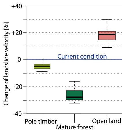
Fig. 4. Boxplots indicating expected changes in landslide velocity regarding different forest cover scenarios.
