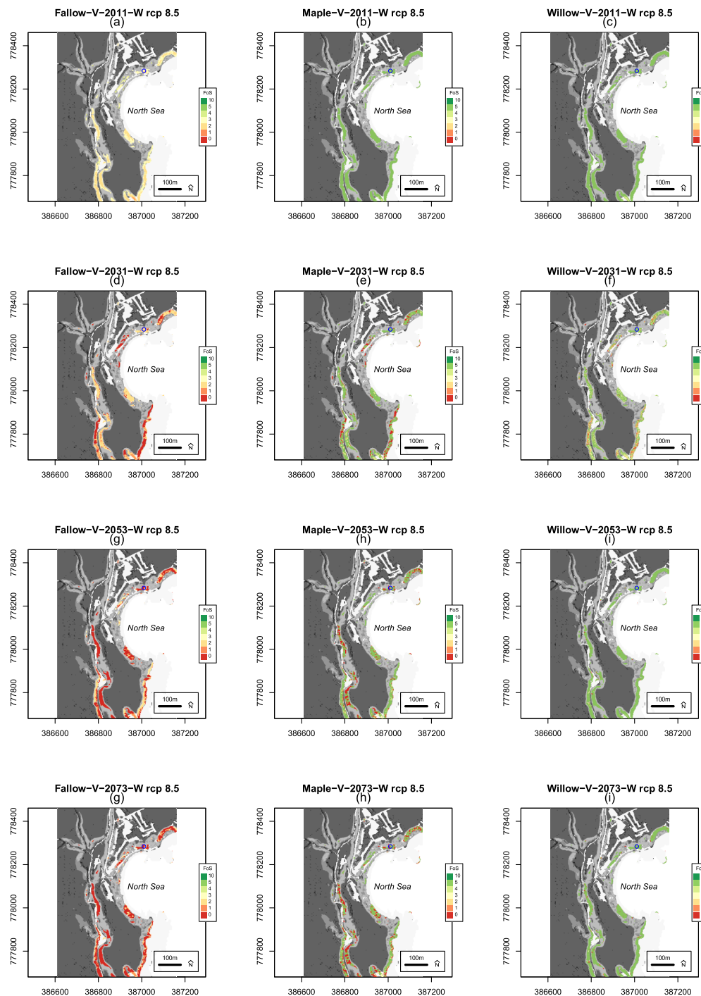
Fig. 8. Model outputs for the Factor of Safety (FoS) at 100–200 mm below ground level (b.g.l.) for fallow, maple and willow groundcovers during the growing season and under wetting cycles for selected rainfall events predicted under the climate change scenario RCP8.5 for the years 2011, 2031, 2053 and 2073 (Table S1). Pixels in red denote landslides, whilst green pixels indicate that the slope is stable. Grey zones are zones where the model was not evaluated as they are not prone to landslides. The FoS profiles for the data point marked in blue are shown in Fig. 10.
