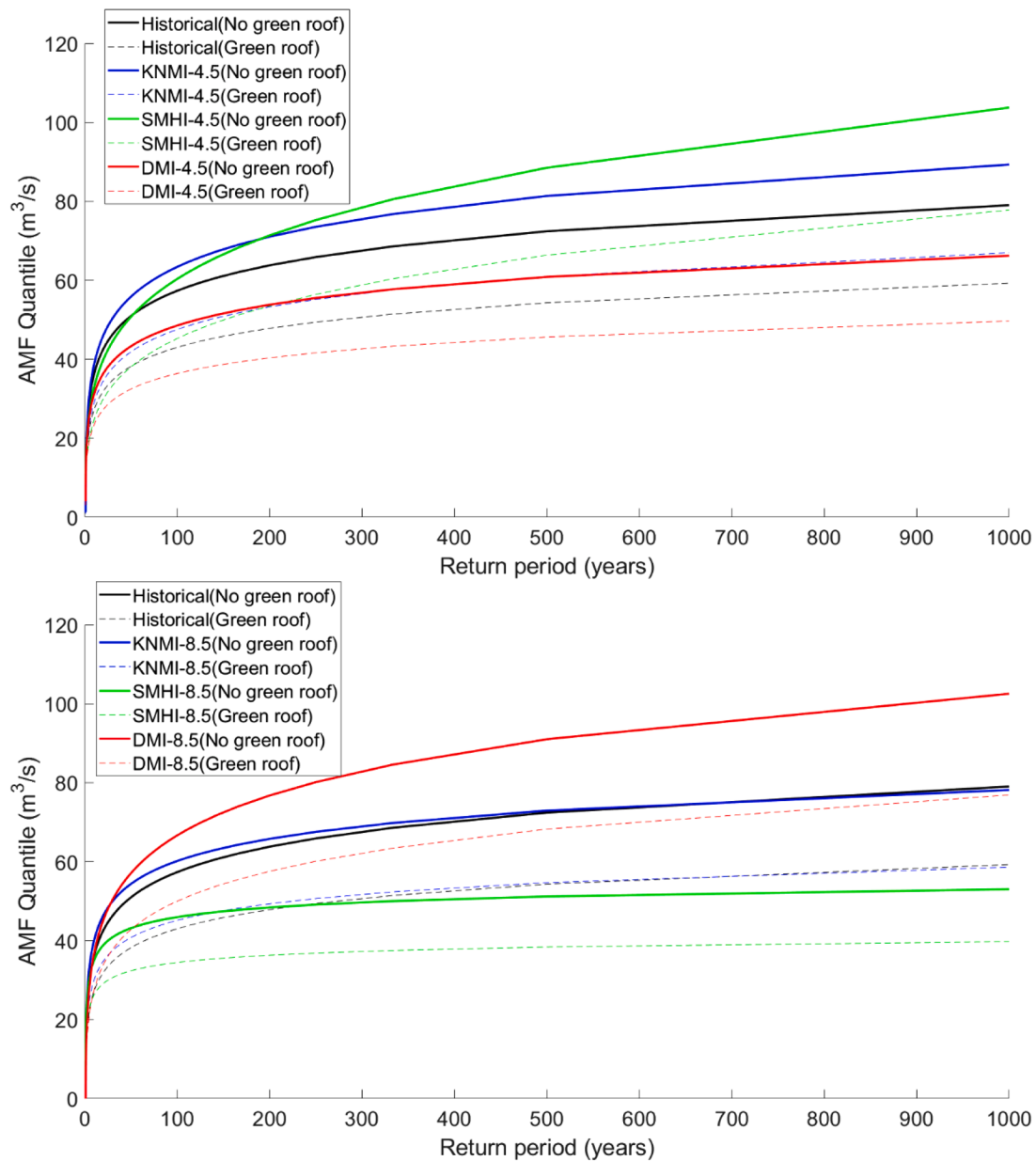
Fig. 7. Quantile plot of annual maximum flows using GEV distribution for the historical and future climate change scenarios (RCP4.5 top, and RCP8.5 bottom), with and without the 160 hypothetical green roofs.
