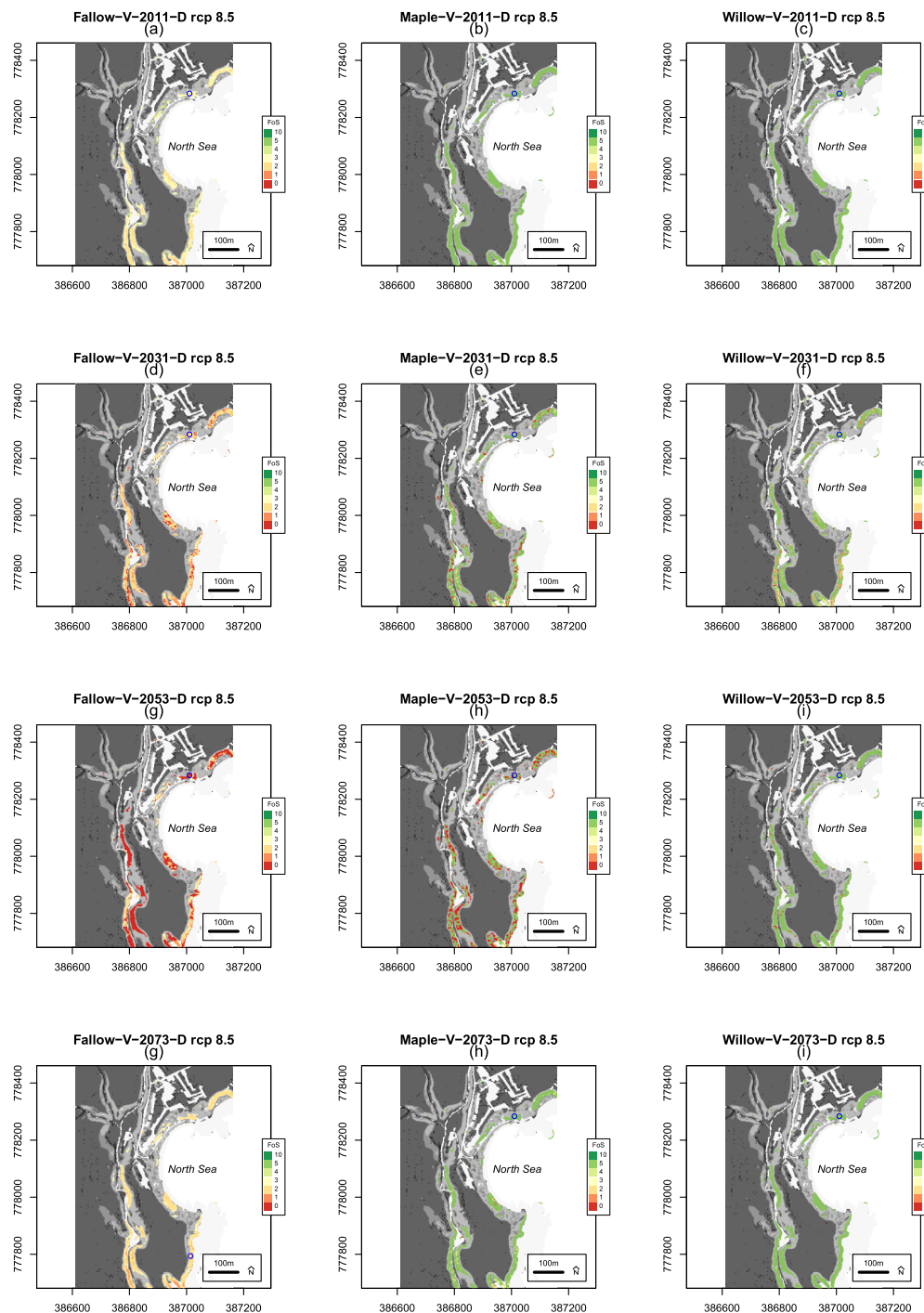
Fig. 9. Model outputs for the Factor of Safety (FoS) at 100–200 mm below ground level (b.g.l.) for fallow, maple and willow groundcovers during the growing season and under drying cycles for selected rainfall events predicted under the climate change scenario RCP8.5 for the years 2011, 2031, 2053 and 2073 (Table S1). Pixels in red denote landslides, whilst green pixels indicate that the slope is stable. Grey zones are zones where the model was not evaluated as they are not prone to landslides. The FoS profiles for the data point marked in blue are shown in Fig. 10.
