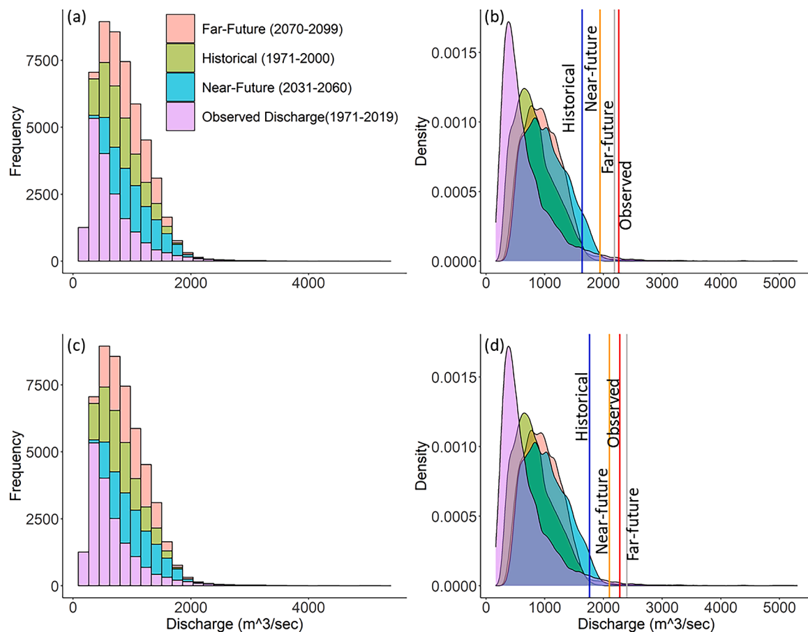
Fig. 5. Distribution of discharges (a and b) Wittenberg (upstream) and (c and d) Neu-Darchau (midstream) of Elbe River basin. The vertical solid lines are showing a 99 % percentile threshold used to extract extreme flood events from the whole time series of discharge and used as a boundary condition in the 1D and 2D hydraulic models.
