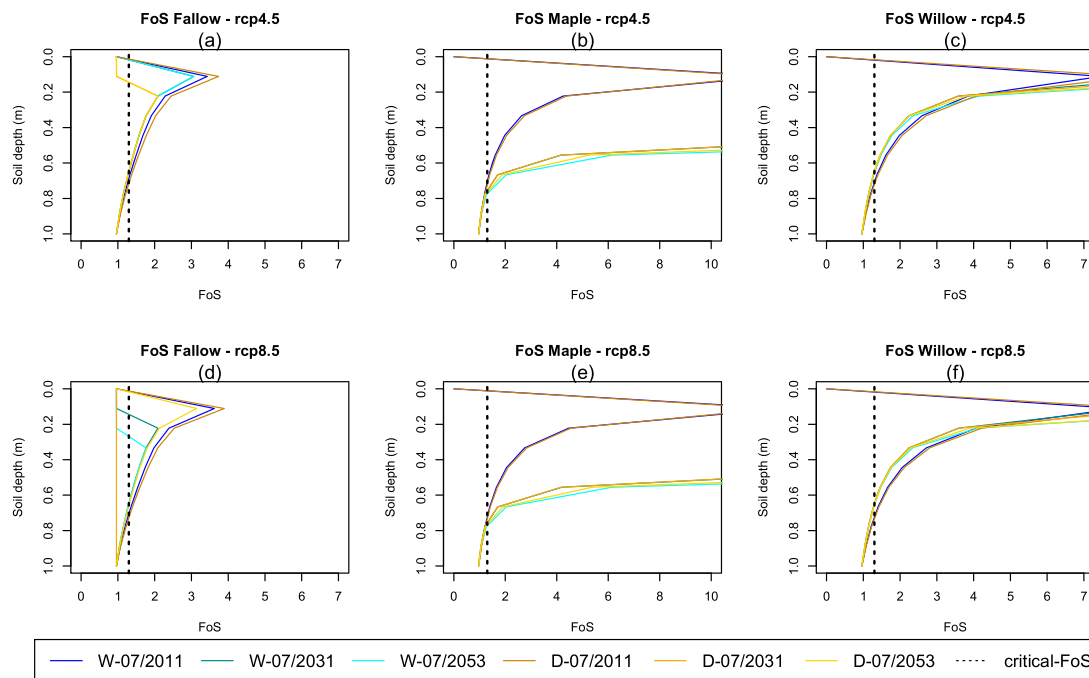
Fig. 10. Factor of Safety (FoS) profiles over the uppermost 1 m, deep soil profile retrieved from the data point shown in Fig. 11 following wetting (W) and drying (D) cycles during the vegetative season predicted with the climate change scenarios RCP4.5 and RCP8.5 for the years 2011, 2031 and 2053 (see Table S1). Slope stability was assessed using the factor of safety (FoS), which is the ratio of driving to resting forces on the slope, denoting stability when FoS is above 1.3 and landslide when FoS is below 1.3.
