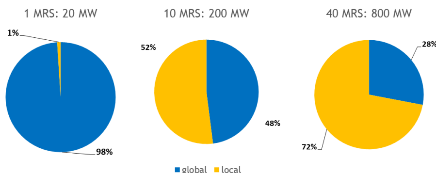
Figure 5. Contribution to downtime from global and local failures for scenarios 1-3.
