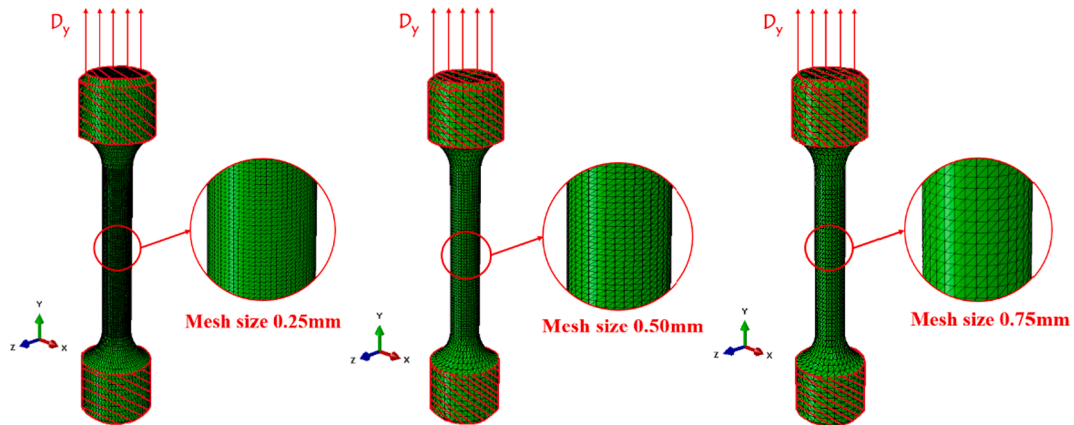
Fig. 2. Mesh size of finite element model and boundary condition.
