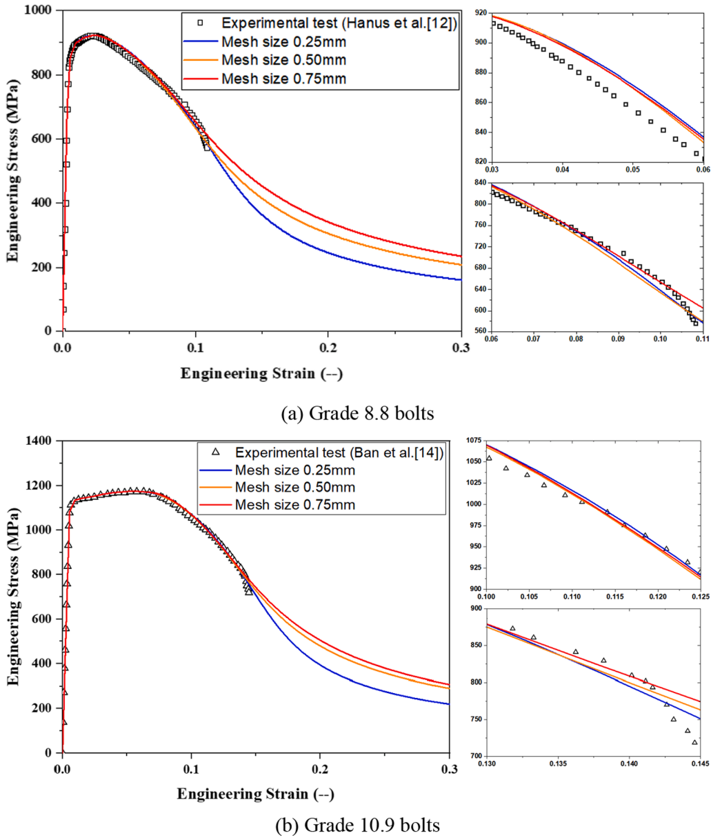
Fig. 3. Comparisons between FE (without damage) and experimental results under different mesh sizes.
