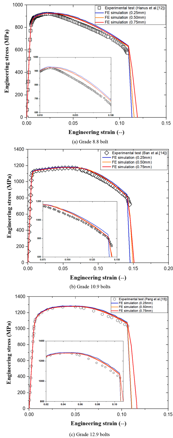
Fig. 10. Calibration of fracture strain exposed to uniaxial loading under different mesh sizes.
