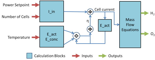
Fig. 1: electrolyzer Model
