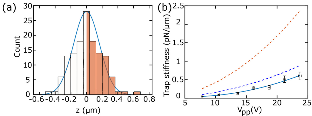
Fig. 7. (a) Example of histogram obtained with the image processing procedure and the calibration curve for trapping experiment at 7.5 \text{ MHz} and 18.7 V_{pp} with z -coordinate representing the distance away from the trap/focal plane. The hollow side of the histogram represents the mirrored data since in the measurement only absolute values are recorded. The blue line is a least squares 1D Gaussian fit to the midpoint on top of each histogram (b) experimentally obtained trap stiffness (solid blue line) for different V_{pp} . The error bars represent the uncertainty in the experimental results and the blue solid line is a second order polynomial fit to the experimental data. For comparison, we show the dashed blue line and dashed red line representing the simulation result with and without glue (glue thickness of 20 \mu\text{m} ).
