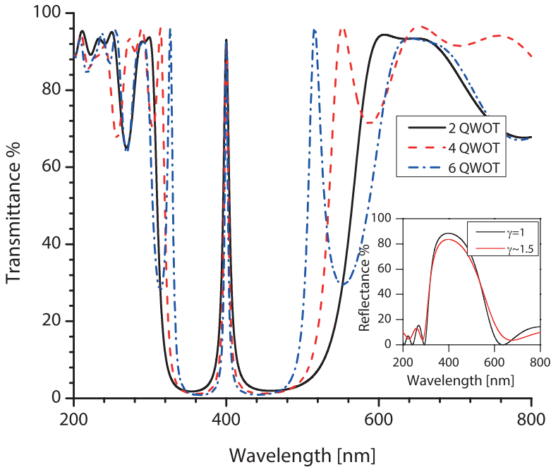
Figure 2.15: Spectral transmittance of an \text{Al}_2\text{O}_3 |airgap-based optical filter as listed in Table 2.1. Multiple resonator layer thicknesses were plotted. The Figure in the insert shows the reflectance of the top ( \gamma = 1 ) and the bottom ( \gamma = 1.5 ) DBRs.
