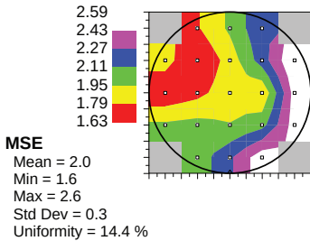
Figure 4.1: Thickness uniformity mapping of Type 1 PECVD deposited oxides measured by VASE (variable angle spectroscopic ellipsometry). The MSE distribution of the optical model used for the analysis is also shown. (The values shown in the insert are all in nanometer.)
