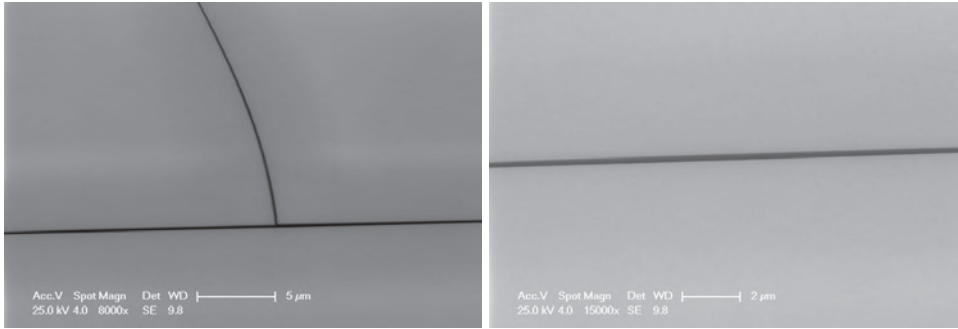
Figure 3.17: SEM micrographs of fracture propagation in 3 \mu\text{m} thick tensile PECVD oxide layers.
