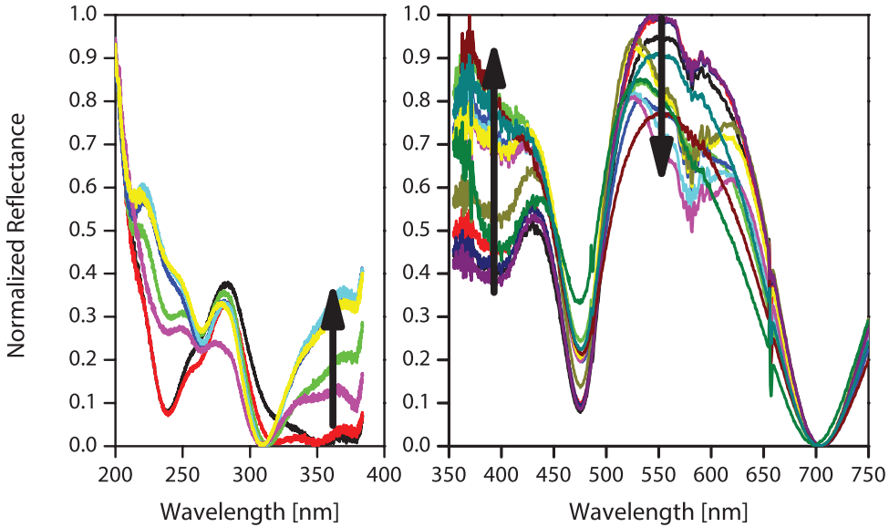
Figure 5.30: The measured reflectance spectra of design a samples. As the peak at 400 nm intensifies, the peak at about 550 nm decreases. The spectral reflectance over UV and over visible was measured using dedicated spectrometer modules and normalized separately, thus the data is not continuous in this figure.
