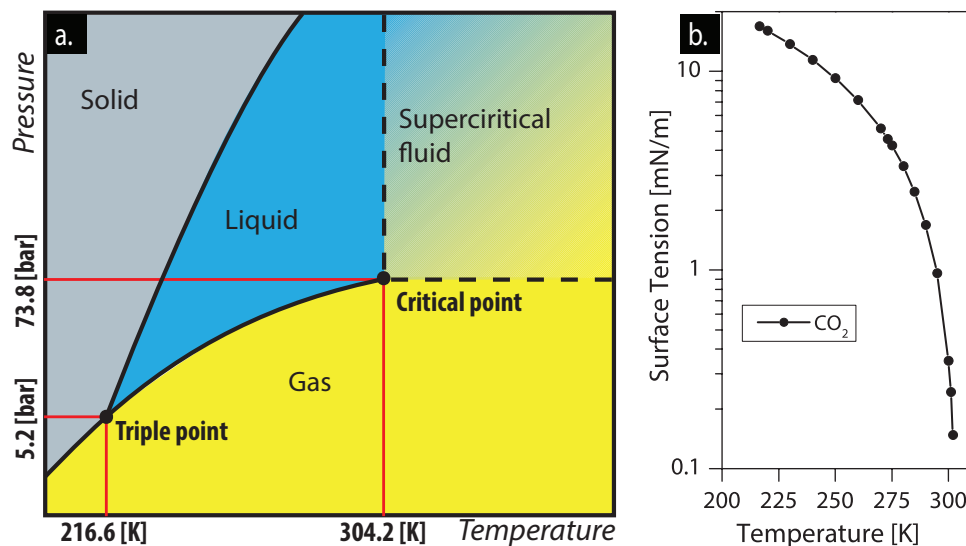
Figure 3.26: (a) Schematic representation of pressure-temperature phase diagram of \text{CO}_2 . Triple and critical point data were adapted from NIST Chemistry WebBook [46]. (b) variation of surface tension in \text{CO}_2 near the critical point obtained from [47].
