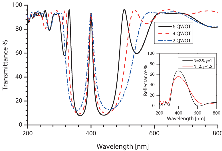
Figure 2.16: The spectral transmittance of a \text{SiO}_2 /airgap-based optical filter as listed in Table 2.1 and for different cavity length. The figure in the insert shows the reflectance of the top ( \gamma = 1 ) and the bottom ( \gamma = 1.5 ) DBRs.
