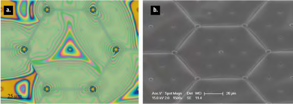
Figure 5.11: a. Microscope image of the single membrane (N=1) of Type 1 . The interference fringes indicate a stress induced deformation in the membrane. b. 45-degree tilted SEM image of the same membrane.
