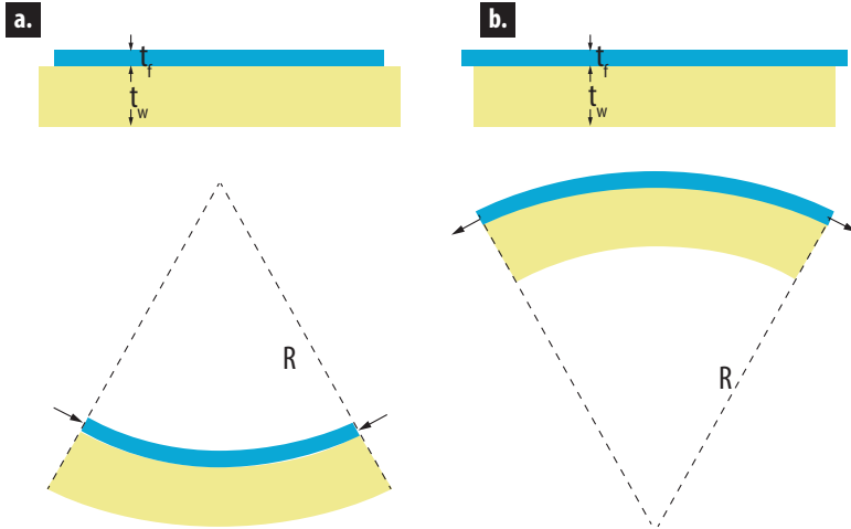
Figure 3.1: Schematic of change in wafer curvature due to the residual stress, a. Tensile stress, and b. Compressive stress
