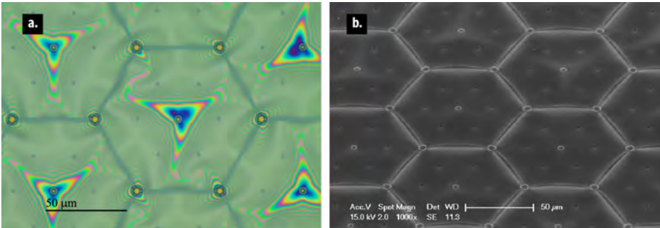
Figure 5.12: a. Microscope image of the single membrane (N=1) of Type 2 . The interference fringes indicate a stress induced deformation in the membrane. b. 45-degree tilted SEM image of the same membrane.
