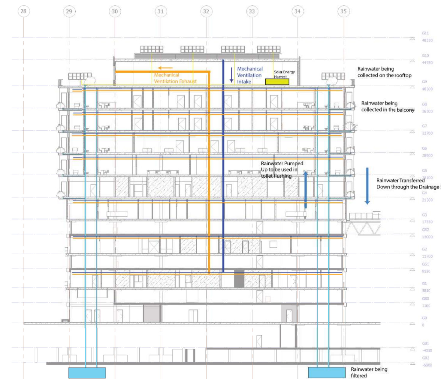
Climate Diagram
