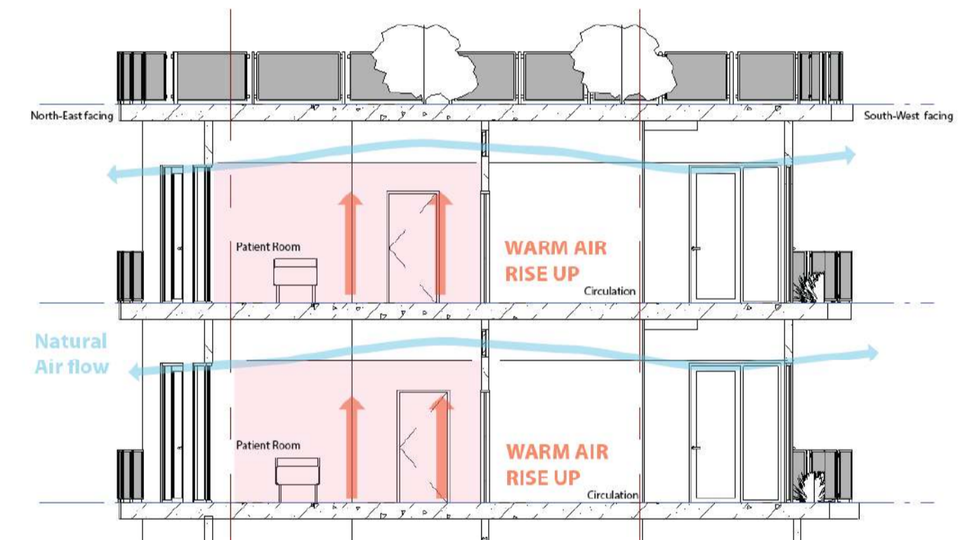
Natural Ventilation Flow on NE & SW facing facade(Patient Rooms)
