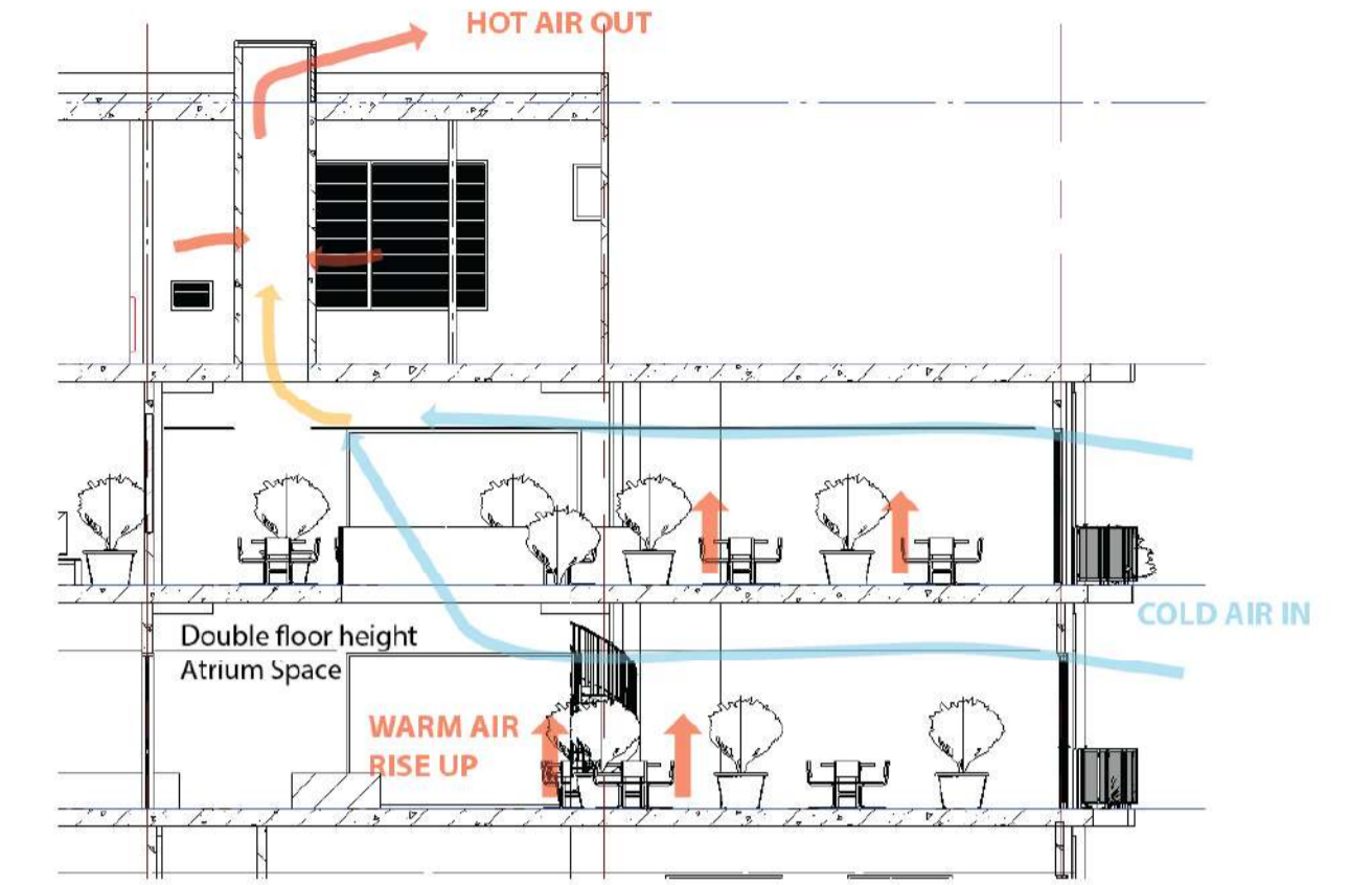
Natural Ventilation Flow on North West facing facade(Double Floor Height Atrium Space)
