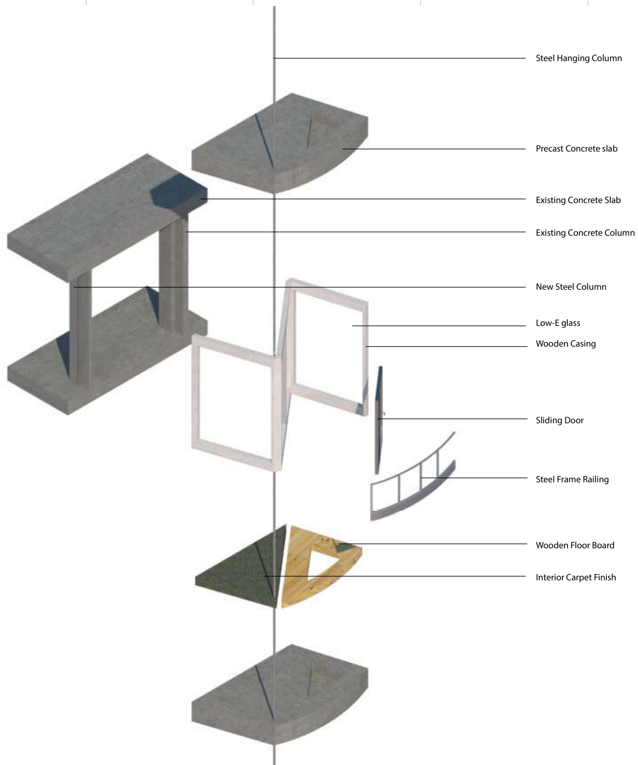
Exploded Axonometric Drawing of the Modular Balcony
