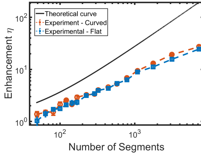
Fig. 2. Enhancement versus number of segments. The black curve is the theoretical limit, the orange circles are the enhancement for a curved sample, and the blue squares are the enhancement for a flat sample. The error bars are of the size of the markers.
