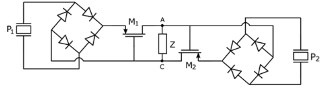
Fig. 3. Schematic of the proposed topology.
