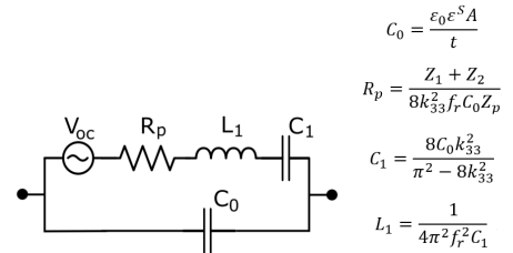
Fig. 4. Model of the electrical impedance of a piezoelectric receiver with equations for calculating the values of the passive elements.
