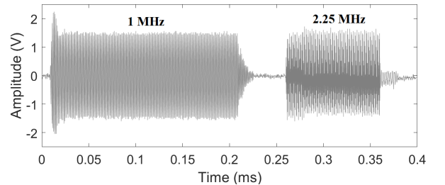
Fig. 9. Measured received 1 MHz and 2.25 MHz open-circuit voltage.
