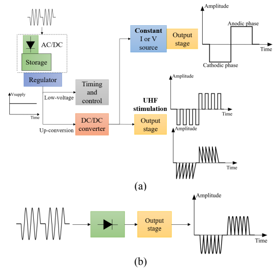
Fig. 1. General blocks scheme and shape of stimulating pulses for (a) a constant current/voltage stimulator or for a conventional UHF stimulator, and for (b) proposed UHF stimulator.
