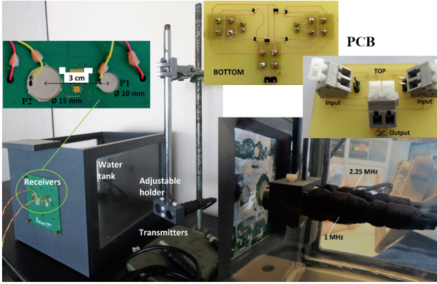
Fig. 5. On the left: setup with transducers and water tank. On the top-right: top and bottom sides of the fabricated PCB. On the bottom right: picture of the transmitters in water aligned at about 2 to 3 cm distance with the receivers on the other side of an acoustic transparent membrane.
