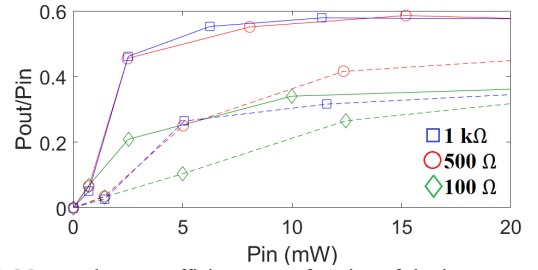
Fig. 7. Measured power efficiency as a function of the input power and for three different output loads. Solid lines are for a 1 MHz sinusoidal input, while the dashed lines are for a 2.6 MHz one.
