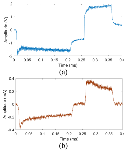
Fig. 10. Measured biphasic voltage (a) and current (b) between a pair of PtIr electrodes.
