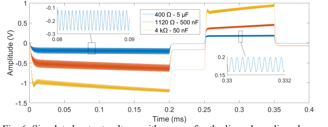
Fig. 6. Simulated output voltage with zoom of cathodic and anodic pulses.
