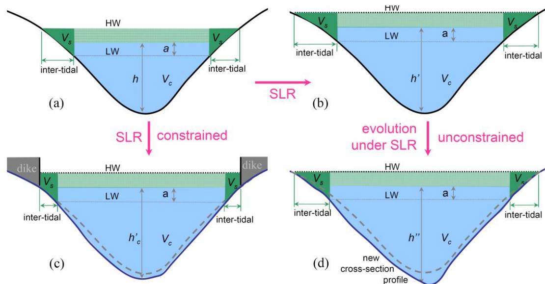
Figure 10. Sketches showing the cross-section profile changes under SLR and consequent morphological evolution: (a) initial condition; (b) under SLR, and with morphological changes under SLR in (c) constrained and (d) unconstrained tidal basin. HW and LW indicate high water and low water, respectively, and V_c and V_s are channel volume below mean sea level and inter-tidal storage volume, respectively. The dashed lines indicate the new profiles considering morphodynamic adjustment under SLR.
