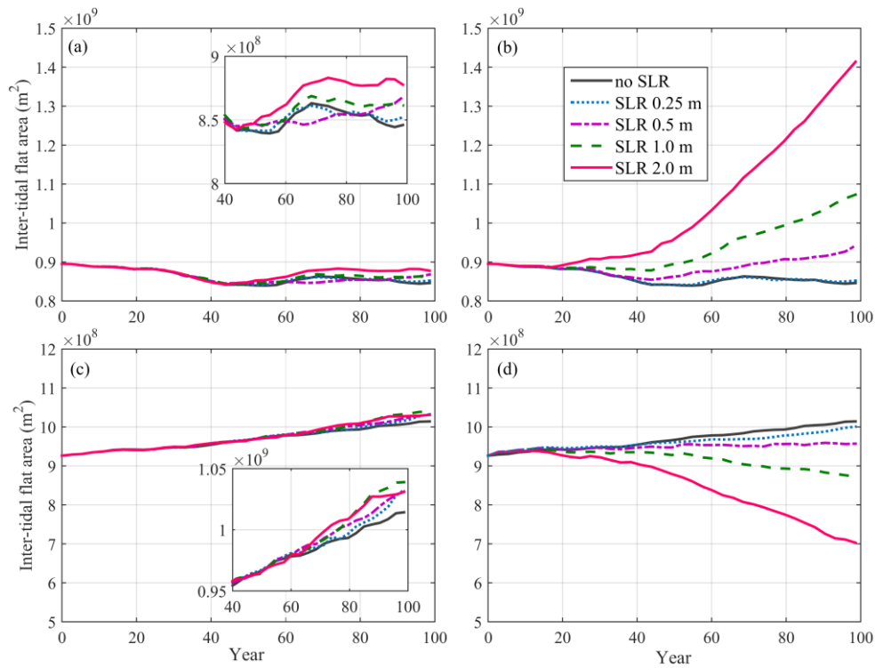
Figure 7. Inter-tidal flat area changes in the tidal basin (a, b) and in the ebb delta (c, d) with respect to a fixed tidal frame (a, c) and with respect to a moving frame of reference level following SLR (b, d). The inset plots in (a) and (c) expand the last 60 years.
