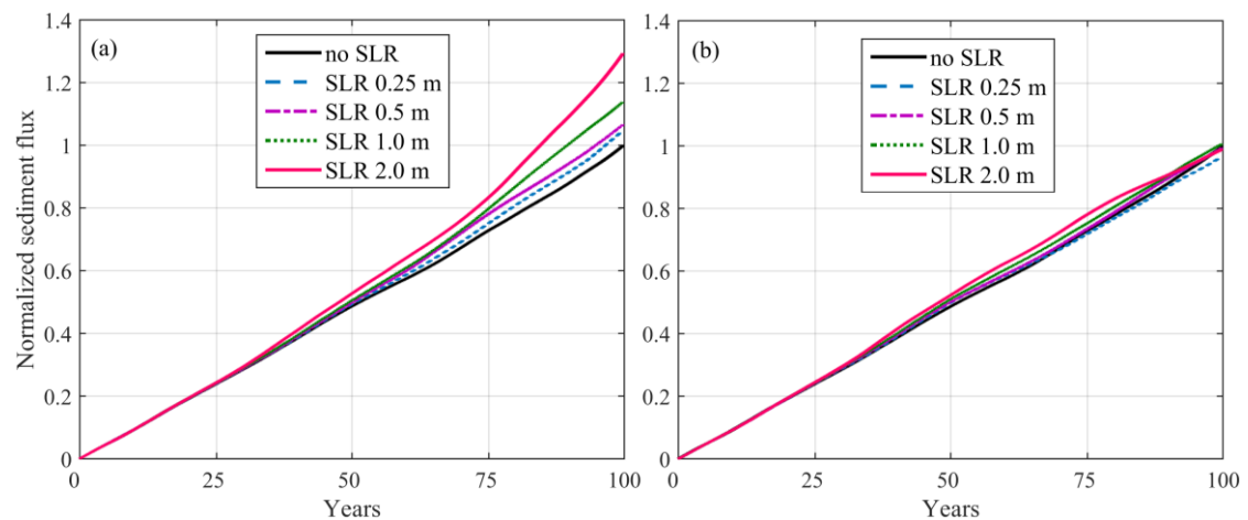
Figure 6. The cumulative sediment flux at the mouth section over the 100 years which are normalized by the cumulated flux in the no SLR scenario: (a) unconstrained tidal basin with low-lying lands, and (b) constrained tidal basin in which expansion to low-lying land is not allowed.
