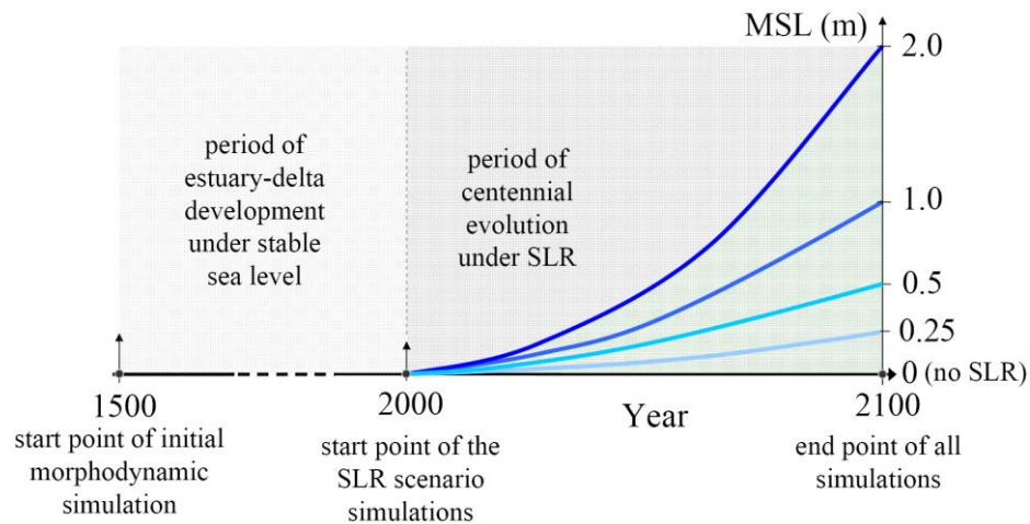
Figure 3. A sketch showing mean sea level changes in the morphodynamic time framework considering different rates of SLR. The first 500 years are squeezed in time scale as indicated by the dashed line.
