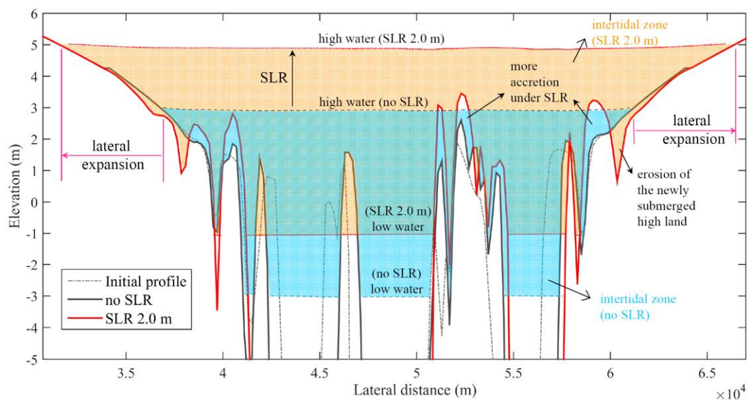
Figure 5. Changes of a cross-section profile at x=130 km (the deeper part of the channel segment is not shown) and associated high water and low water changes in the reference run and 2.0 m SLR scenario including lateral expansion and extra erosion of the newly-submerged inland zone under SLR.
