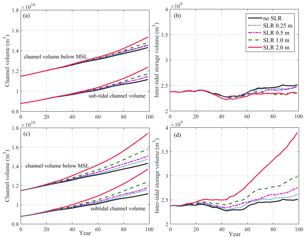
Figure 9. Changes of (a, c) channel volumes below mean sea level (MSL) and low water (subtidal), and (b, d) intertidal storage volumes inside the tidal basin. The panels (a, b) and (c, d) are the results calculated according to fixed and moving tidal frames, respectively.
