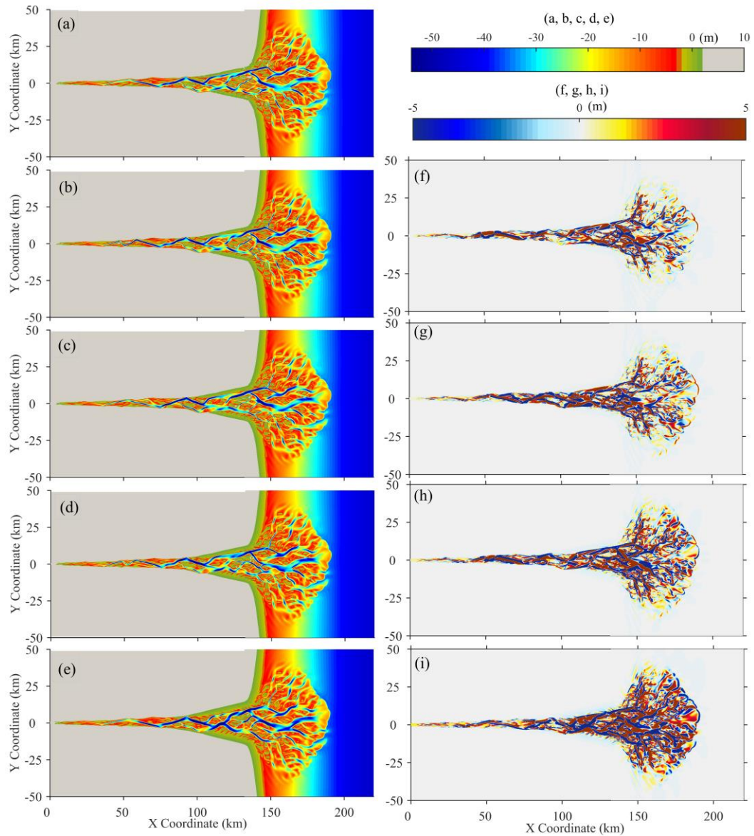
Figure 4. The morphology after 100 years considering (a) no SLR, SLR of (b) 0.25 m, (c) 0.5 m, (d) 1.0 m, and (e) 2.0 m, and accordingly bathymetry differences between the reference scenario and the scenarios with SLR of (f) 0.25 m, (g) 0.5 m, (h) 1.0 m, and (i) 2.0 m. The green shading in panels (a) to (e) roughly indicates inter-tidal zone. The dashed lines in panels (f) to (i) indicate the 2 m elevation contour in the reference scenario and the solid lines are the 2 m elevation contour in the SLR scenarios. Positive values in panels (f) to (i) indicate accretion while negative values indicate erosion in the SLR scenarios compared to the reference case. The bed elevation in panels (b) to (e) is referenced to the raised mean sea levels in the SLR scenarios, with the
