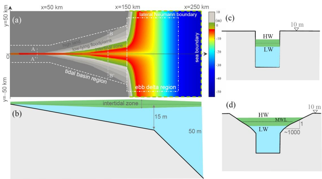
Figure 2. Sketches of the schematized model domain setting in distorted space scales: (a) the planform of the tidal basin with division between the inner basin and the outer delta regions, (b) a side view of the main channel and initial bed profile, and (c, d) cross-section profiles of A-A' and B-B', respectively. The green shading indicates the inter-tidal zone. Both the bank and the bed are erodible. The dashed and dash-doted boxes in panel (a) indicate the regions of tidal basin and the ebb delta, respectively.
