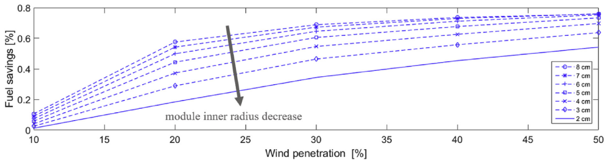
Fig. 15. Annual fuel savings for various thermal storage module inner radii.
