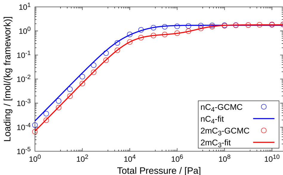
Figure 7. Pure component adsorption isotherms of n\text{C}_4 and 2m\text{C}_3 in MFI-type zeolite at 400K. Pure component adsorbed loadings calculated using GCMC for the pressure range ( 10^0 - 5 \cdot 10^{10} ) Pa are fitted using the dual-site Langmuir isotherms. The empty circles represent GCMC simulation data and the solid lines are the dual-site Langmuir isotherms fitted to these data sets.
