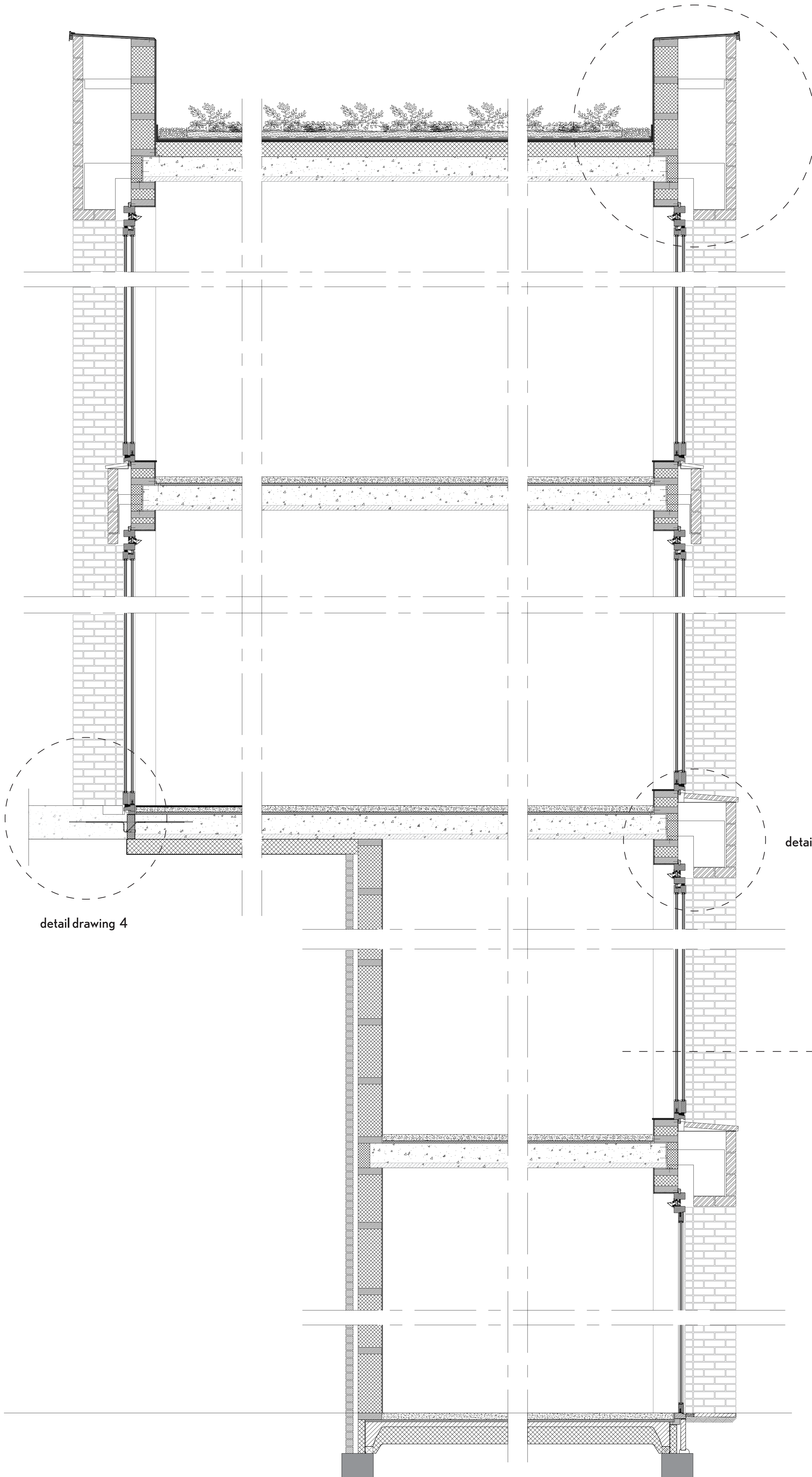
detail drawing 3
