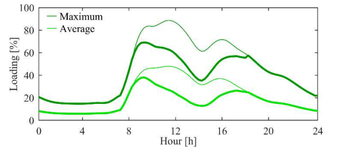
Fig. 6. Maximum and average line loading with (thicker) and without (thinner) PV production.
