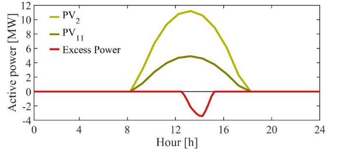
Fig. 5. Installed PV system active power production.
