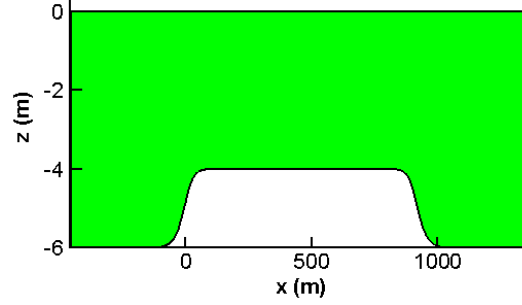
Figure 5.2 Bathymetry of the computational area
