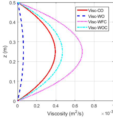
Figure 5.9 Reynolds turbulent viscosity ( \nu_v^T )
