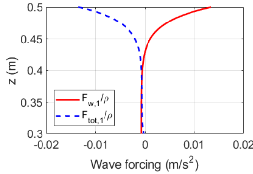
Figure 5.32 Vertical distribution of wave-induced forcing terms
