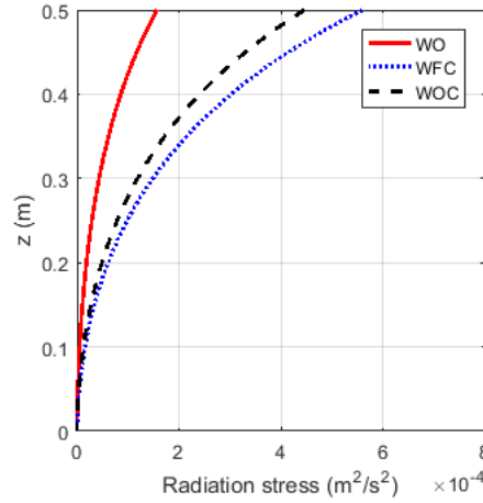
Figure 5.10 Vertical distribution of the wave radiation stress component \overline{\tilde{u}\tilde{w}_{CS}}
