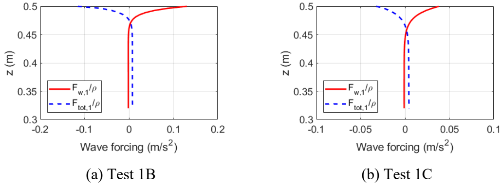
Figure 5.22 Distribution of wave-induced forcing terms at x = 22.9 m
