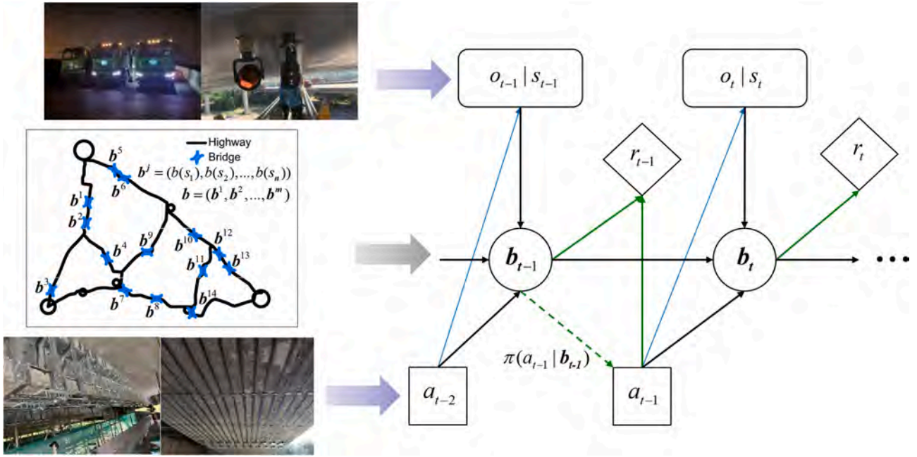
Fig. 2. Probabilistic graphical model of POMDPs.
