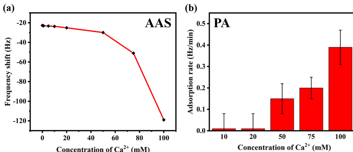
Fig. 4. Observed maximal frequency shifts for the adsorption of 0.15 wt% AAS (a) and observed adsorption rates for 20 ppm PA (b) both as a function of a varying \text{CaCl}_2 concentration (0–100 mM) in the presence of 500 mM NaCl. The unit conversion: 1 wt% = 10,000 ppm.
