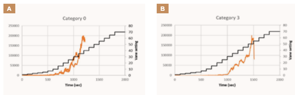
FIGURE 12 The increase in turbidity (left Y-axis in non-calibrated turbidity units; turbidity increases as the units do) over time (X-axis in seconds) in orange, with black being the stepwise increase of the vane setting every 100 seconds (right Y-axis in non-calibrated shear units; applied shear increases as the units do). Sediment in category 0 contains no sulfide oxidizer mat. Sediment in category 3 contains a well-developed mat.
