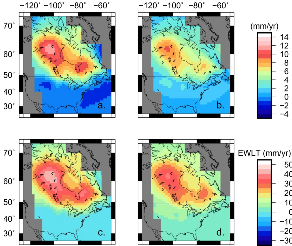
Figure 3. A priori GIA model inputs. Shown are vertical land motion rates averaged over a suite of 150 models (a) and the associated standard deviation of the vertical motion rates for the entire suite of models (b). (c) and (d) are the same as (a) and (b), except rates of gravity change are shown and are expressed as change to equivalent water layer thickness (EWLT). Uncertainty rates are not VCE-scaled.
