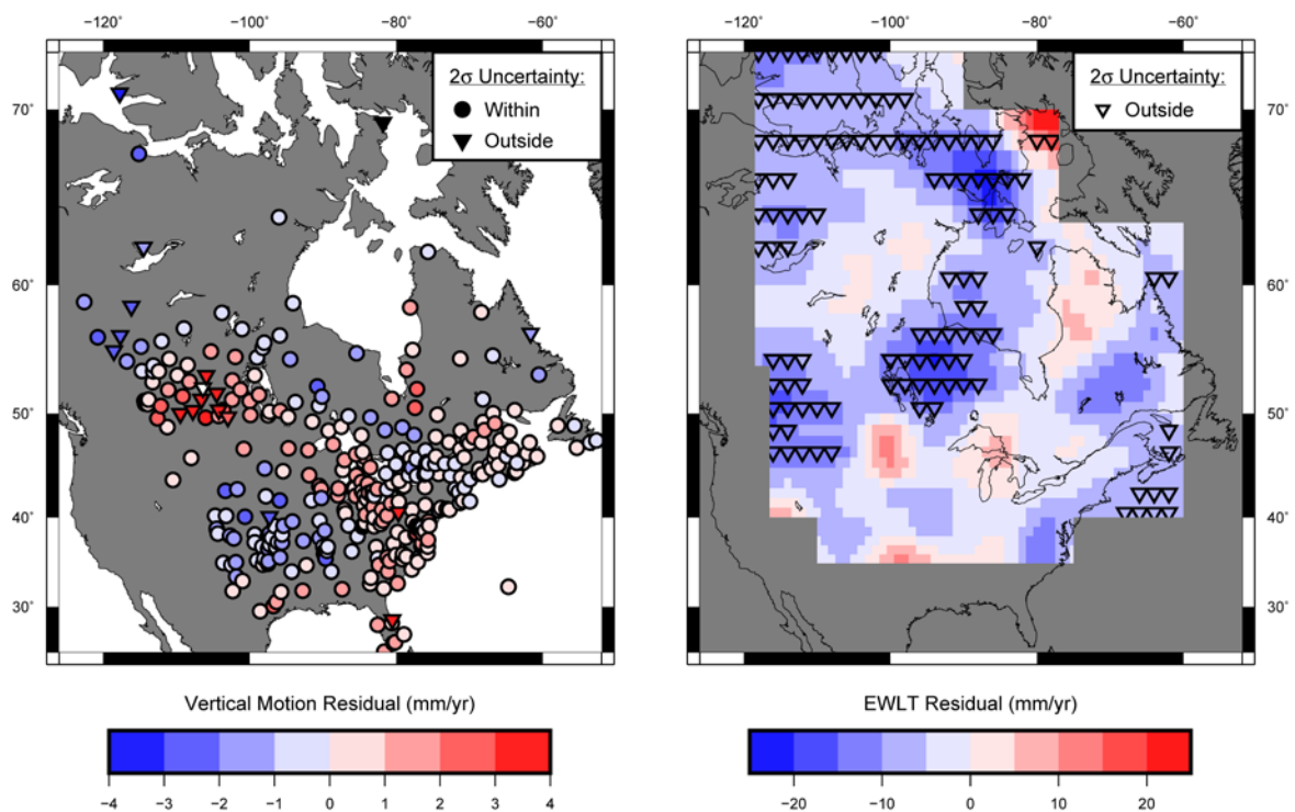
Figure 6. Residuals of model predictions relative to observations for vertical motion (left) and gravity change (right). Residuals that are within the 2\sigma uncertainty of the observations are plotted with a circle (left only); residuals that exceed the 2\sigma uncertainty of the observations are plotted with an inverted triangle (left and right). Model prediction is for the D3 combined data scenario (both vertical motion and gravity change data are incorporated).
