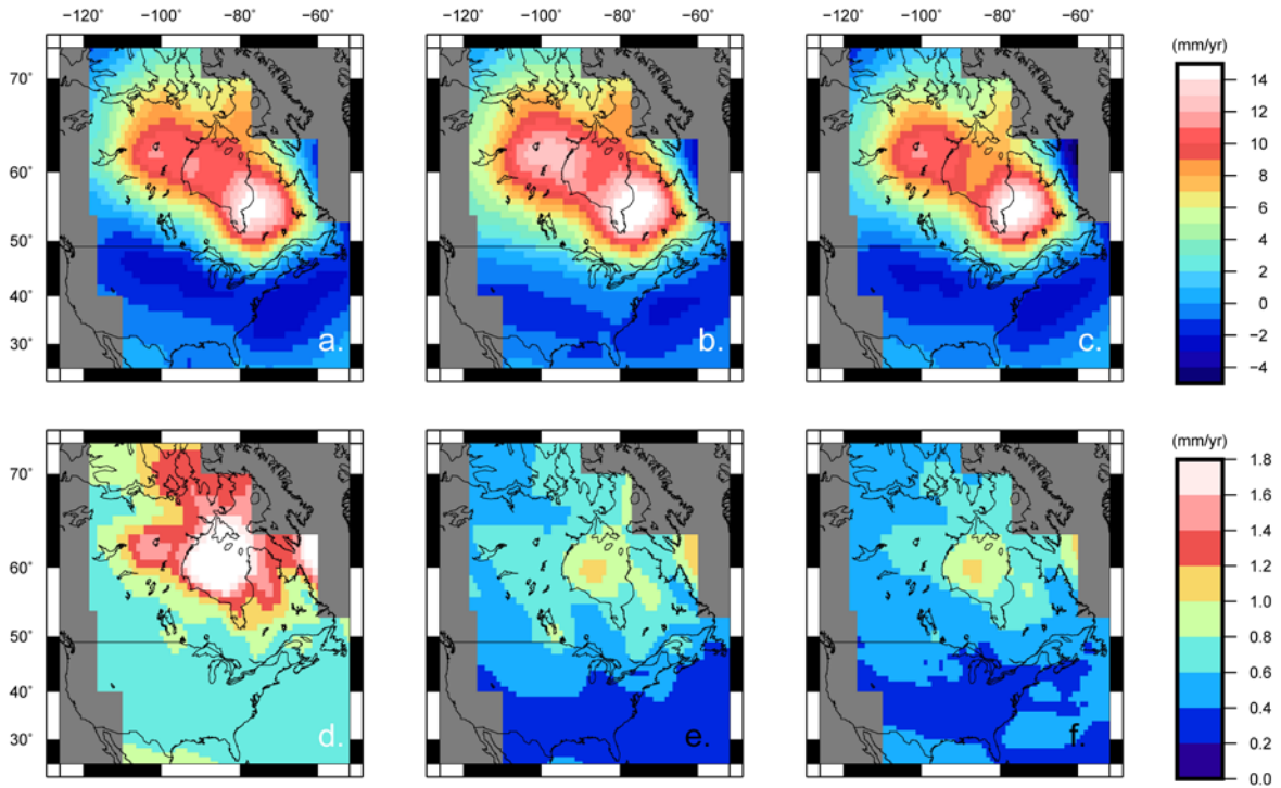
Figure 4. Results for prediction of rates of GIA-induced vertical land motion for three scenarios: a) inversion of the vertical motion data only (D1), b) inversion of the gravity change data only (D2), and c) inversion of both the vertical motion and gravity data (D3). (d-f) the predicted posterior 2\sigma uncertainties for each of (a-c). Uncertainties are not VCE scaled.
