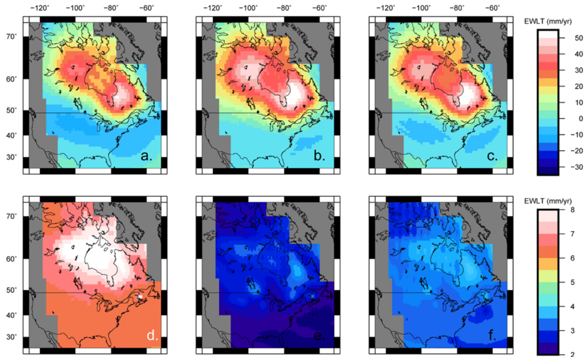
Figure 5. Results for prediction of rates of GIA-induced gravity change for three scenarios: a) inversion of the vertical motion data only (D1), b) inversion of the gravity change data only (D2), and c) inversion of both the vertical motion and gravity data (D3). (d-f) the predicted posterior 2\sigma uncertainties for each of (a-c). Shown in mm/yr of change to equivalent water layer thickness. Uncertainties are not VCE scaled.
