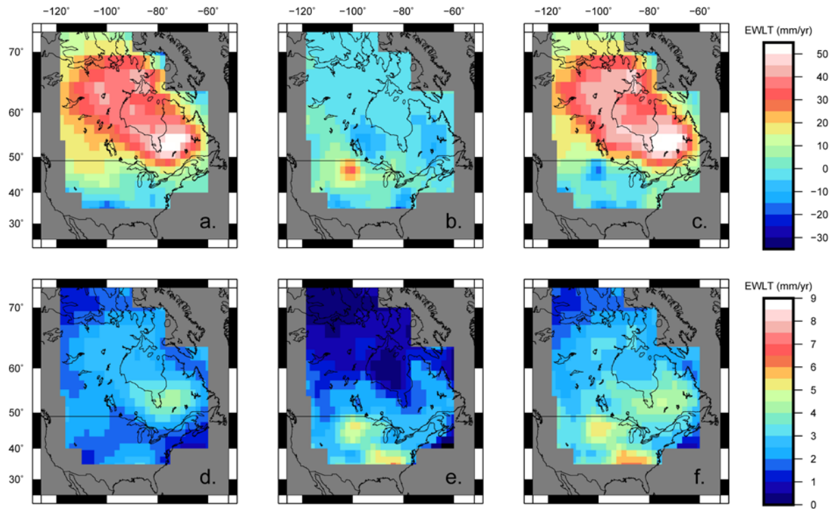
Figure 2. GRACE mass trend, uncorrected for hydrology changes (a), hydrology changes derived from model PCR-GLOBWB (b), GRACE mass trend corrected for hydrology (c). (d)-(f): The 2\sigma uncertainty associated with each of (a)-(c). Time span of all trends is 2004.02 – 2014.06. Units are mm/yr of change to equivalent water layer thickness (EWLT).
