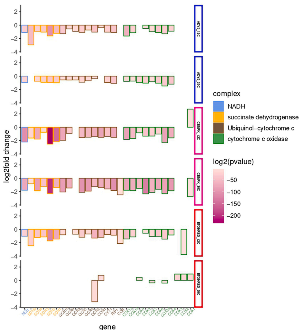
Fig. 5. Electron transport chain expression in ADY5, CEN.PK117-3D and Ethanol Red at 12 and 39 °C. The genes with a significant ( p < 0.05 ) differential expression ( \geq \pm 1.5 log2fc) are represented with bars. For the bars, the deeper the colour, the lowest the p -value. No bar indicates genes that are not differentially expressed in this condition. The genes belonging to the same protein complex are indicated in the same colour. (For interpretation of the references to colour in this figure legend, the reader is referred to the web version of this article.)
